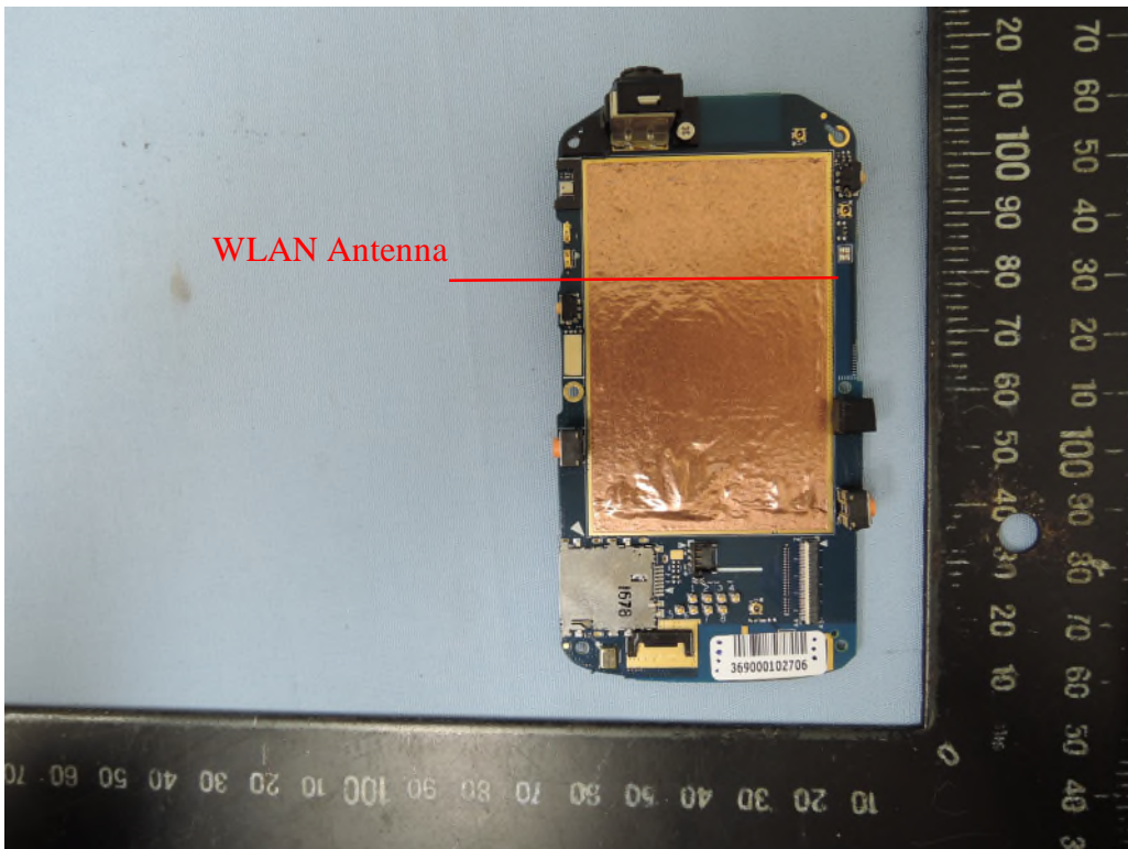
WLAN Antenna
