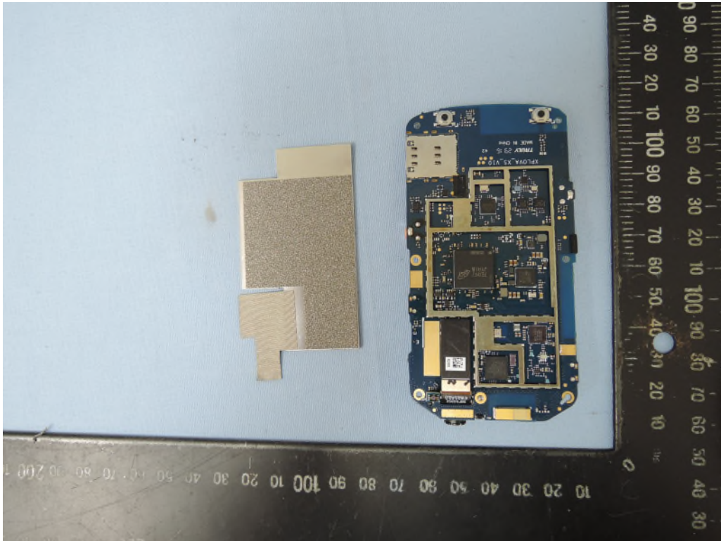
WLAN Antenna
