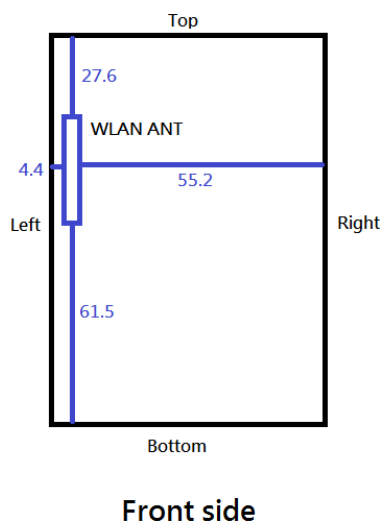
Fig.11 Antenna position (Front side)
