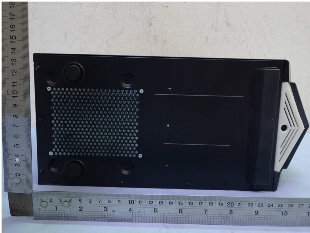
Figure 10 Personal Computer D19W6, General Appearance (Bottom View)
