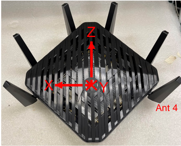
ANT 4_5GHz
