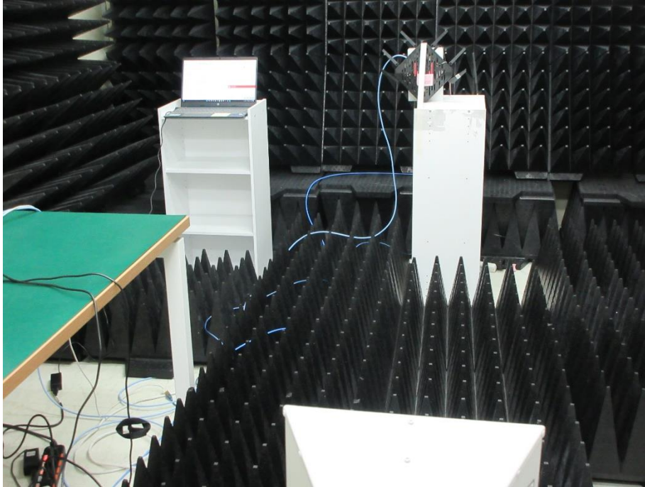
Photograph 9: Test Setup for DFS (Front View)
