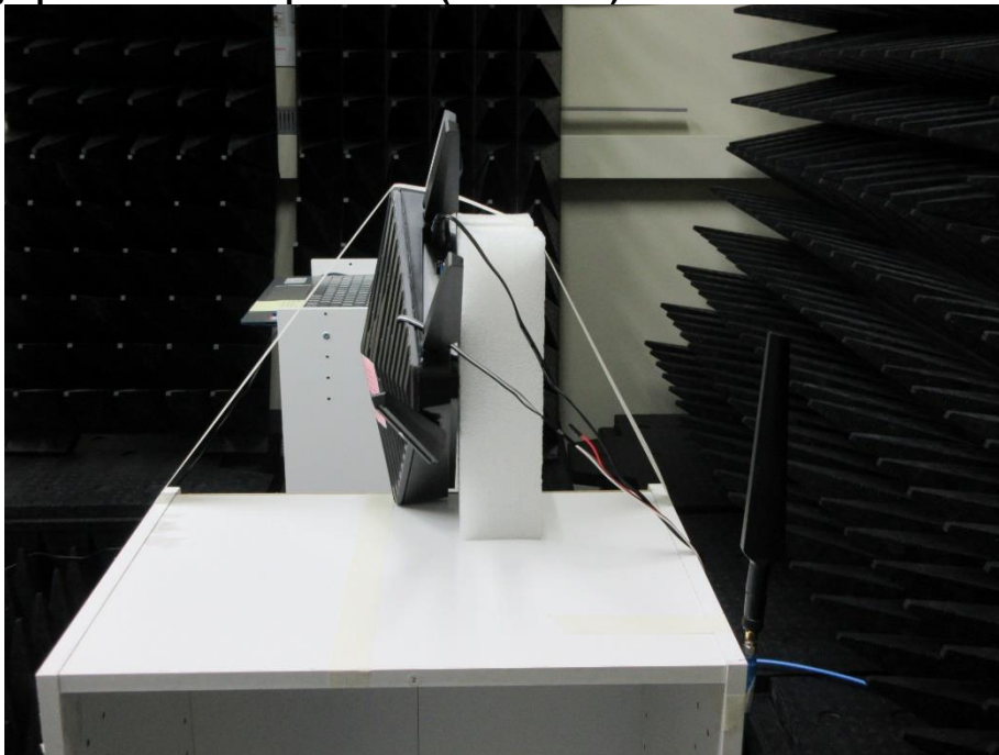
Photograph 10: Test Setup for DFS (Back View)
