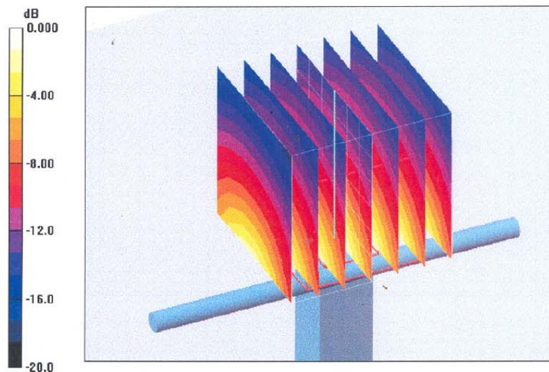
0 dB = 11.8mW/g
