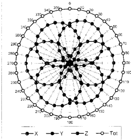
f = 1800 MHz, WG R22
