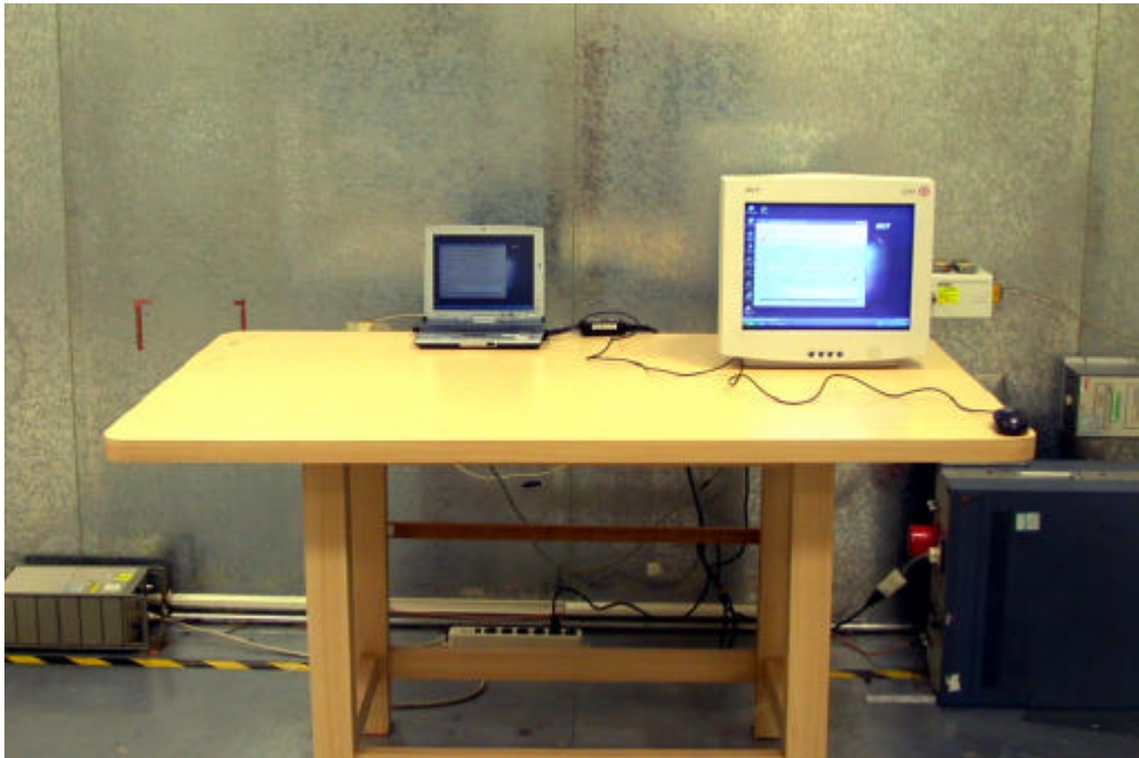
The Front View of Highest Conducted Set-up
