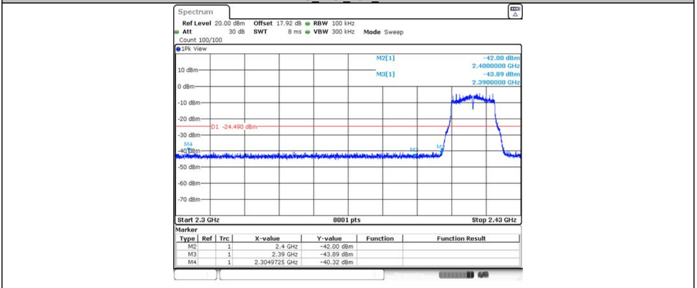
11G Ant2_Low_2412
