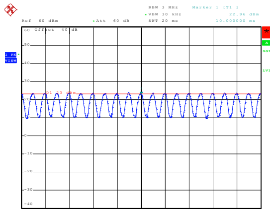
1880MHz - 80% AM
