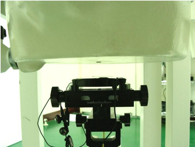
Bottom of the DUT with Phantom 2.5 cm Gap with Earphone 1 for Sample A
