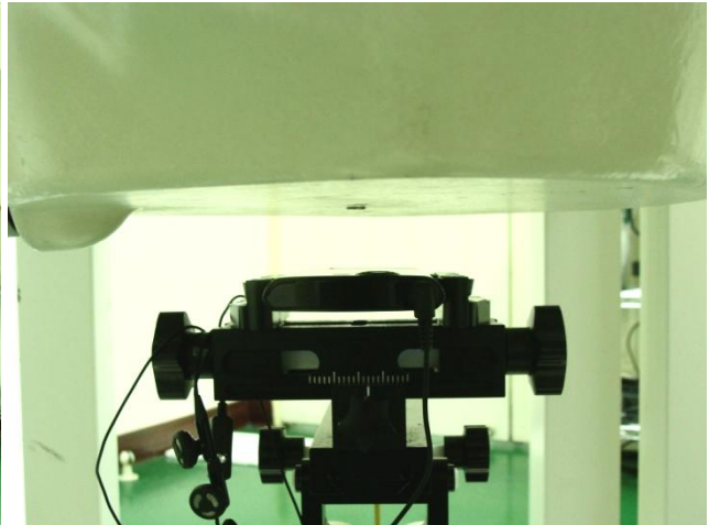
Bottom of the DUT with Phantom 2.5 cm Gap with Earphone 1 for Sample B
