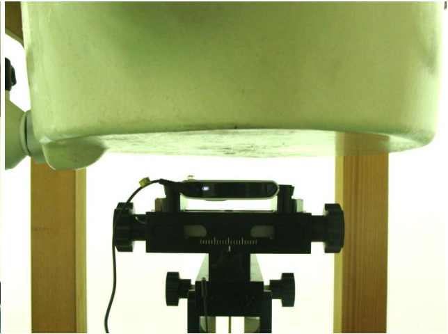
Face of the DUT with Phantom 2.5 cm Gap - Earphone 2
