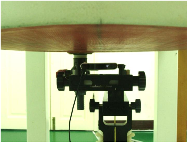
Face of the DUT with Phantom 2.5 cm Gap - Earphone 1
