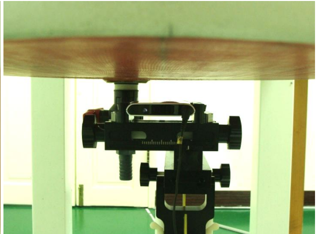
Bottom of the DUT with Phantom 2.5 cm Gap - Earphone 2
