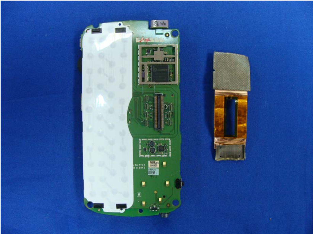
(32) EUT Photo
