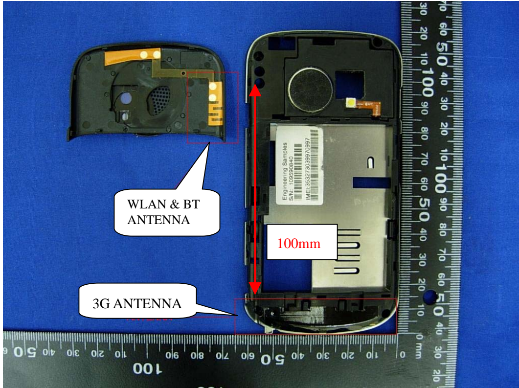
(42) EUT Photo
