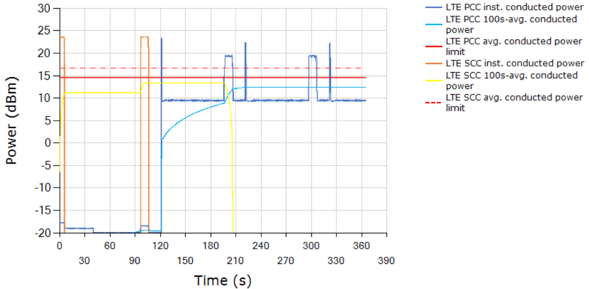
LTE PCC/SCC Instantaneous and Time-averaged TX Power Tech: LTE, Band 4 / Tech: LTE, Band 5
