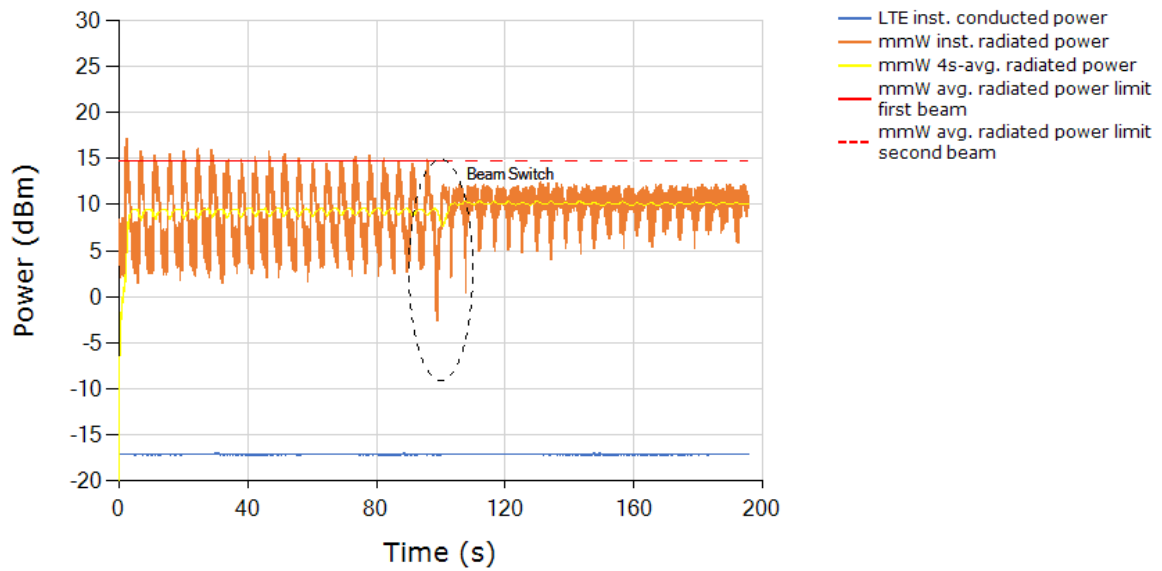
LTE and mmW Instantaneous and Time-averaged TX Power Tech: LTE, Band 66 / Tech: NR5G MMW, Band n260
