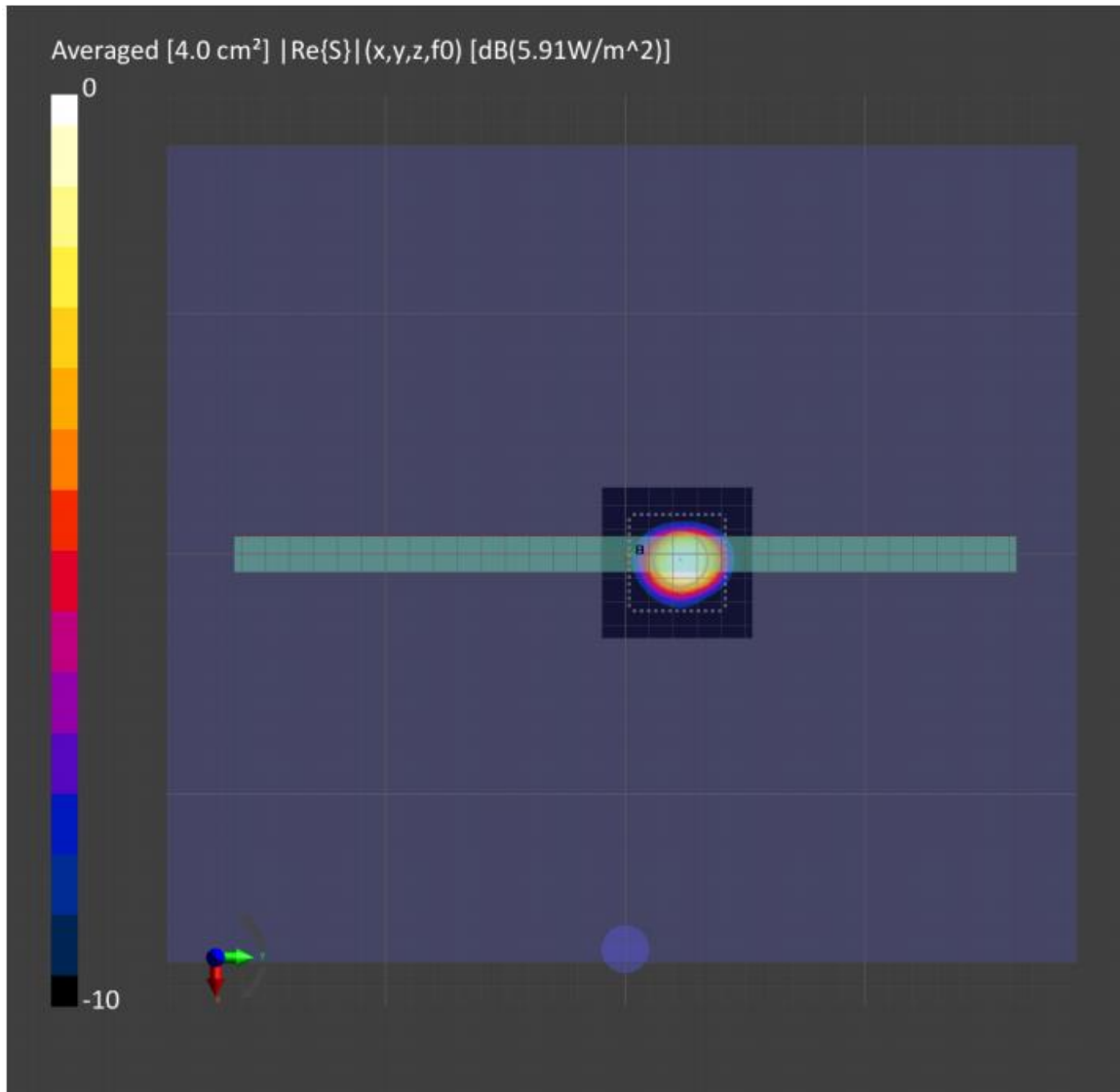
Figure 8-3: 4cm2-averaged power density distribution measured at input.power.limit of 2.36dBm on the back surface for n261 beam 43
