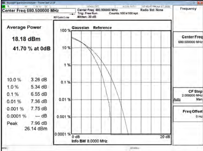
LTE_Band71_15MHz_256QAM_75_0_Mid CH133297-680.5
