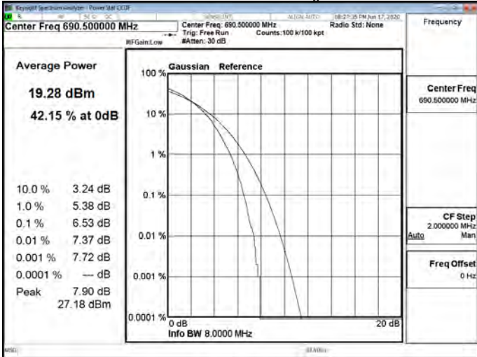
LTE_Band71_15MHz_256QAM_75_0_High CH133397-690.5
