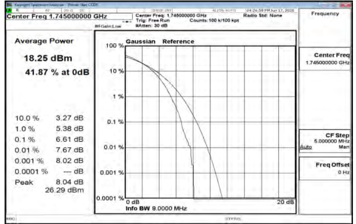
LTE_Band66_15MHz_256QAM_75_0_MidCH132322-1745
