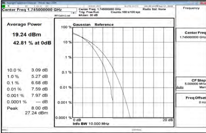
LTE_Band66_10MHz_256QAM_50_0_MidCH132322-1745
