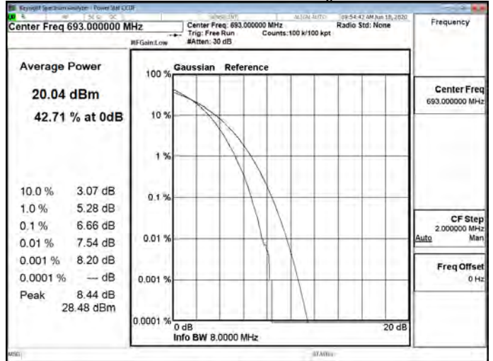
LTE_Band71_10MHz_256QAM_50_0_High CH133422-693
