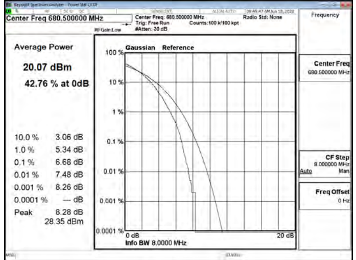
LTE_Band71_10MHz_256QAM_50_0_Mid CH133297-680.5
