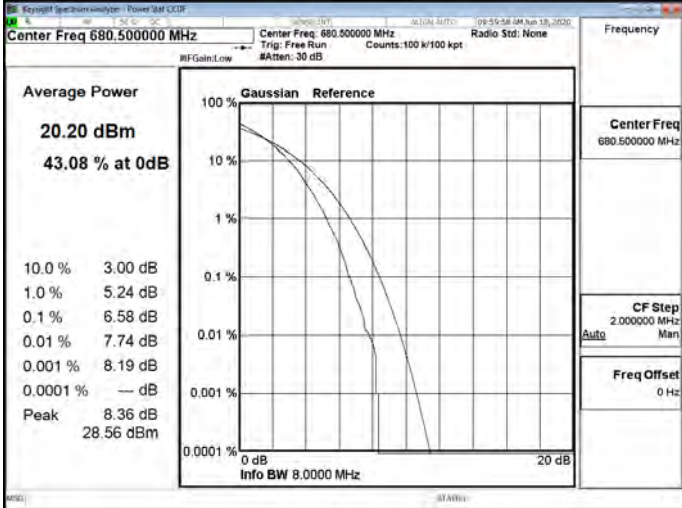
LTE_Band71_5MHz_256QAM_25_0_Mid CH133297-680.5
