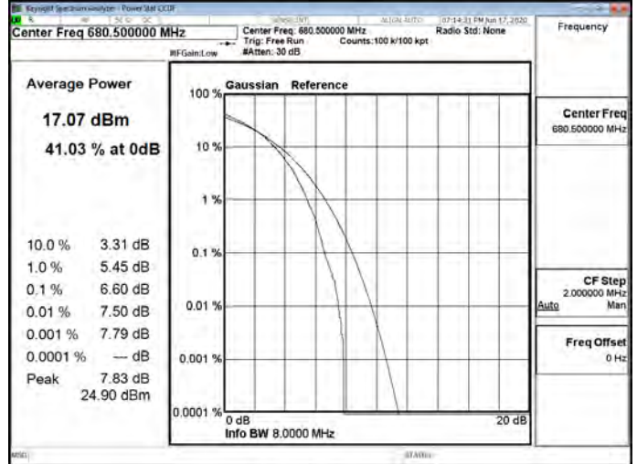
LTE_Band71_20MHz_256QAM_100_0_Mid CH133297-680.5
