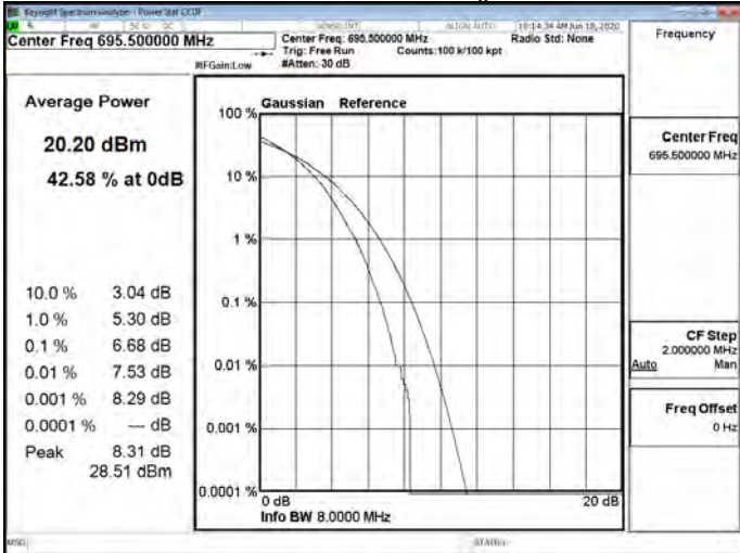
LTE_Band71_5MHz_256QAM_25_0_High CH133447-695.5
