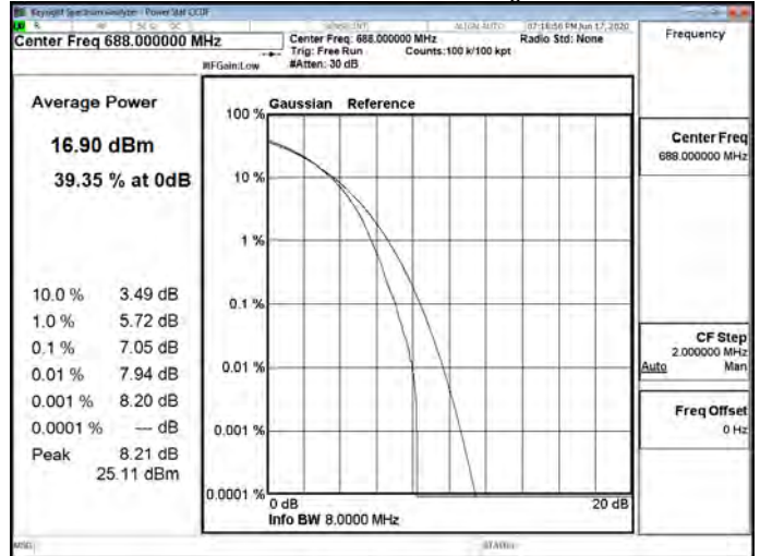
LTE_Band71_20MHz_256QAM_100_0_High CH133372-688
