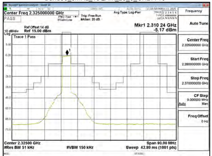
Band30_5MHz_16QAM_25_0_CH27710
