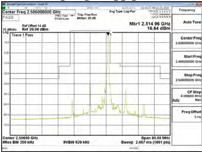
Band41_20MHz_256QAM_1_99_CH40620
