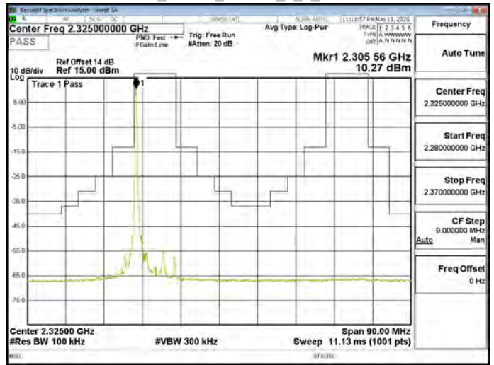
Band30_10MHz_16QAM_1_49_CH27710
