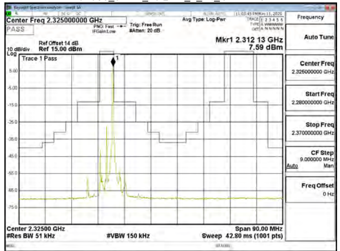
Band30_5MHz_16QAM_25_0_CH27710
