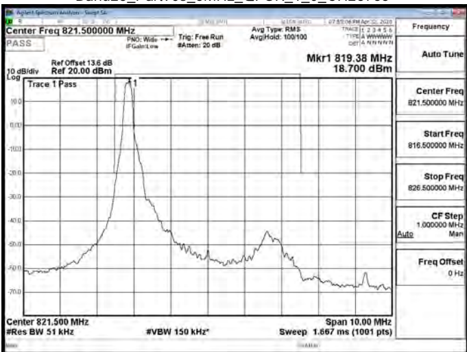
Band26_Part90s_5MHz_QPSK_1_0_CH26765
