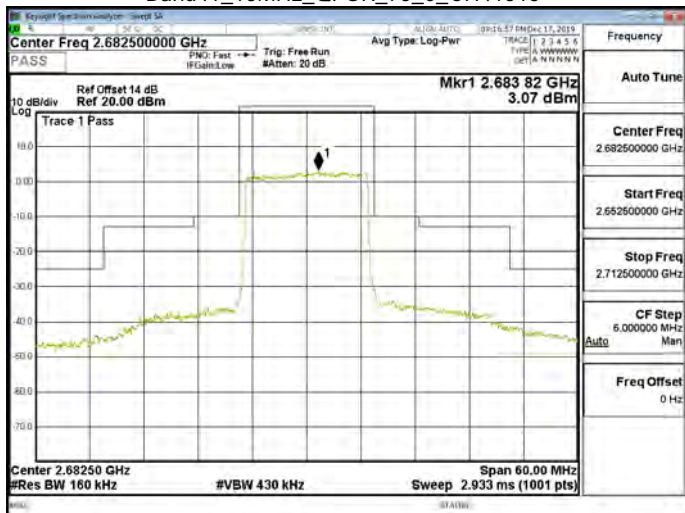
Band41_15MHz_QPSK_75_0_CH41515
