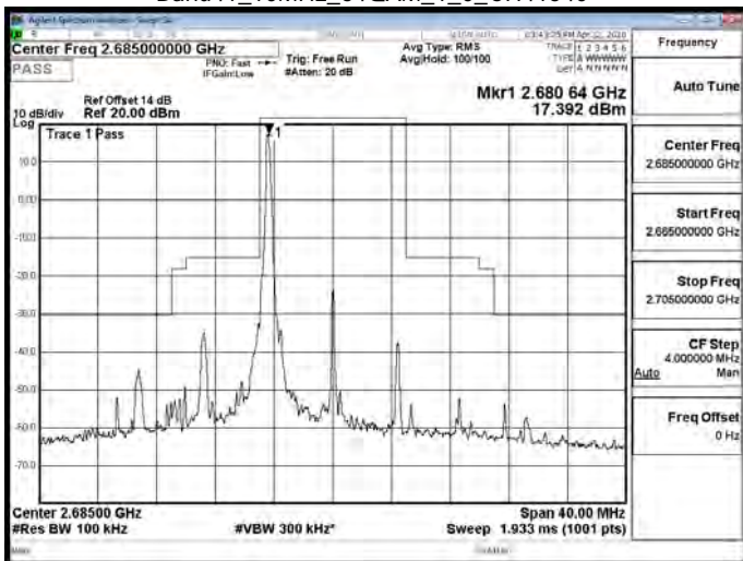
Band41_10MHz_64QAM_1_0_CH41540
