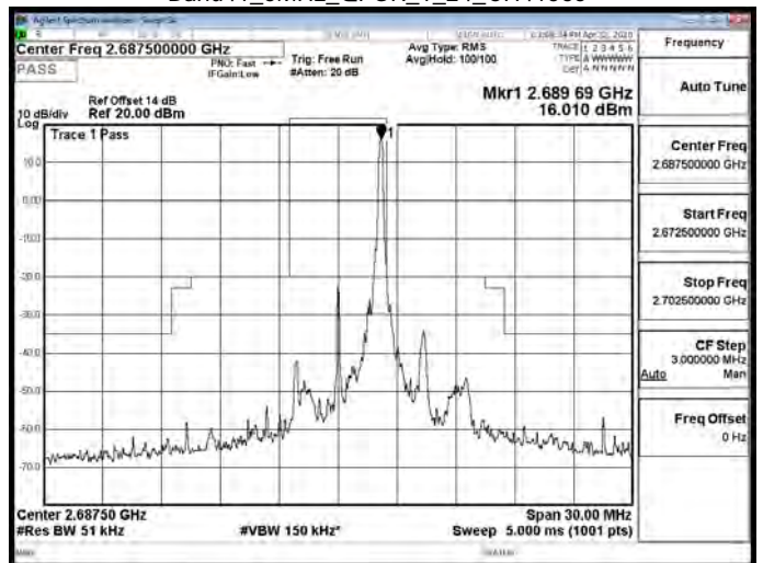
Band41_5MHz_QPSK_1_24_CH41565
