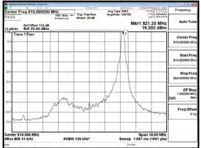
Band26_Part90s_5MHz_QPSK_1_24_CH26765
