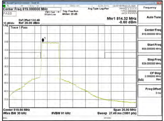
Band26_Part90s_3MHz_256QAM_15_0_CH26740
