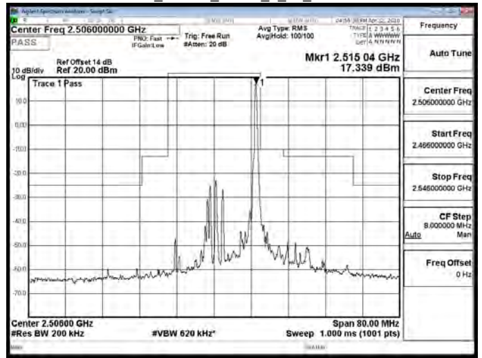
Band41_20MHz_QPSK_1_99_CH40620
