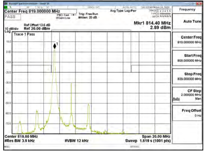
Band26_Part90s_5MHz_256QAM_1_0_CH26740
