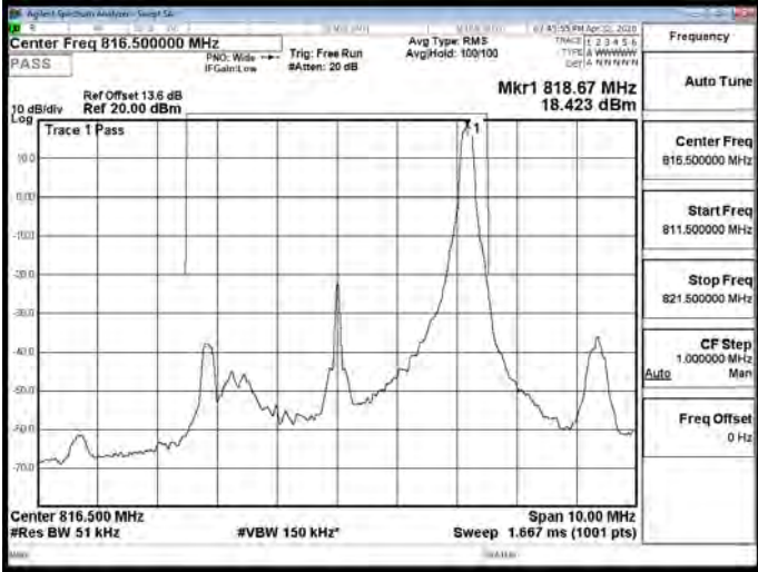
Band26_Part90s_5MHz_16QAM_1_24_CH26740
