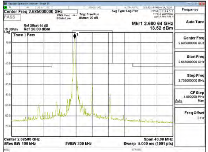
Band41_10MHz_256QAM_1_0_CH41540
