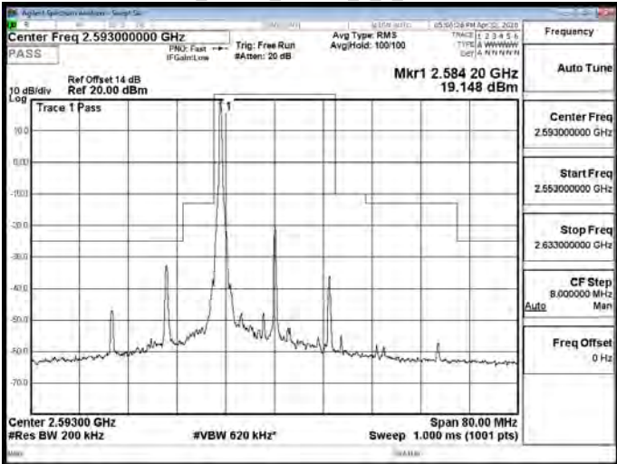
Band41_20MHz_64QAM_1_0_CH41490
