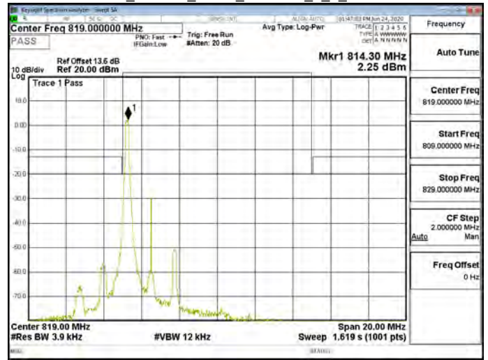
Band26_Part90s_3MHz_256QAM_1_0_CH26740
