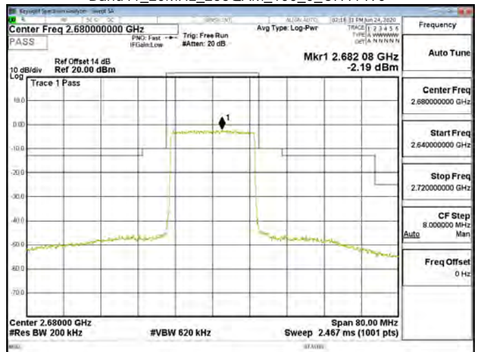
Band41_20MHz_256QAM_100_0_CH41490
