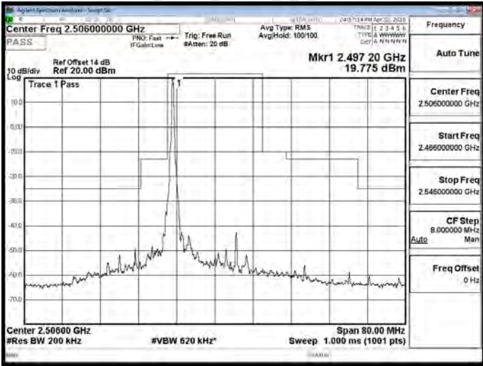
Band41_20MHz_64QAM_1_0_CH40620
