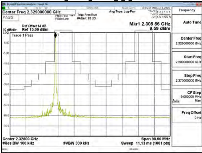
Band30_10MHz_64QAM_1_49_CH27710
