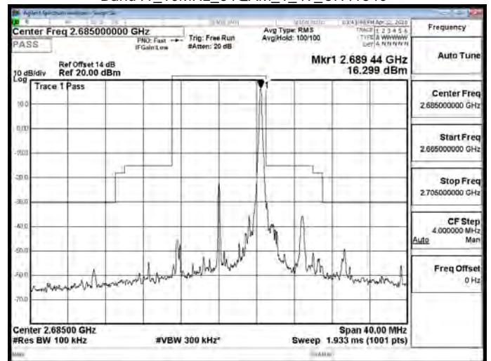
Band41_10MHz_64QAM_1_49_CH41540
