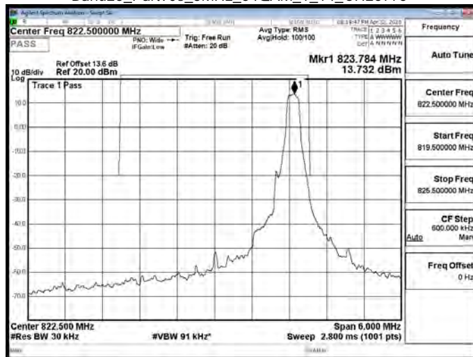
Band26_Part90s_3MHz_64QAM_1_14_CH26775
