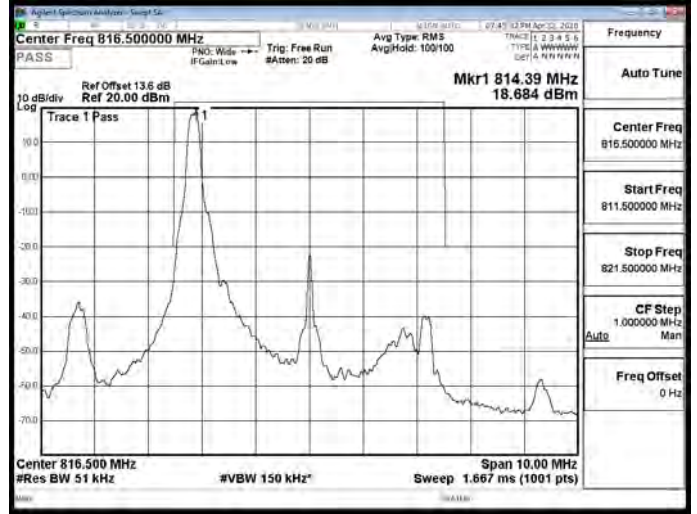
Band26_Part90s_5MHz_16QAM_1_0_CH26740
