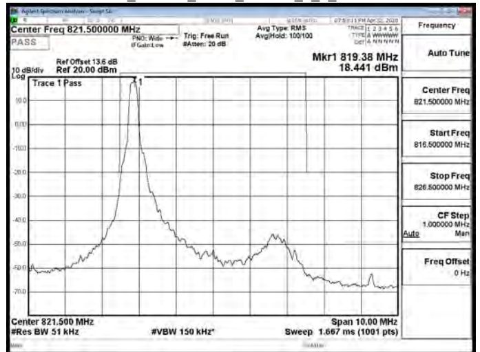
Band26_Part90s_5MHz_16QAM_1_0_CH26765
