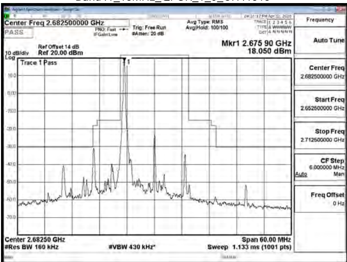
Band41_15MHz_QPSK_1_0_CH41515
