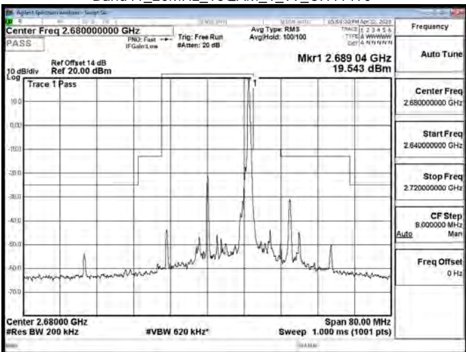
Band41_20MHz_16QAM_1_99_CH41490
