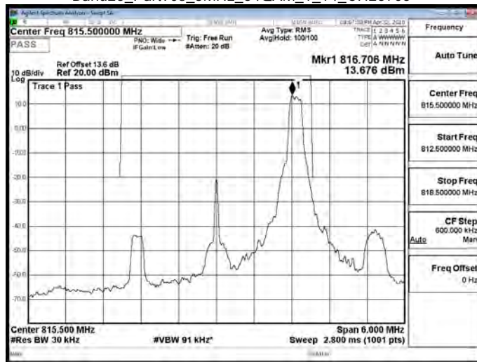
Band26_Part90s_3MHz_64QAM_1_14_CH26740
