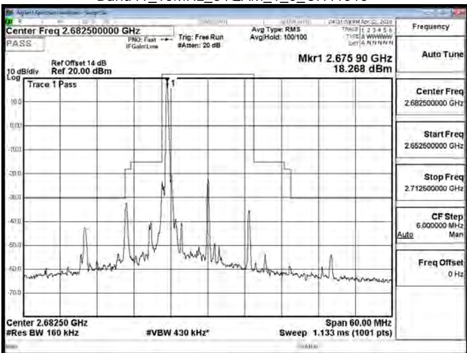
Band41_15MHz_64QAM_1_0_CH41515
