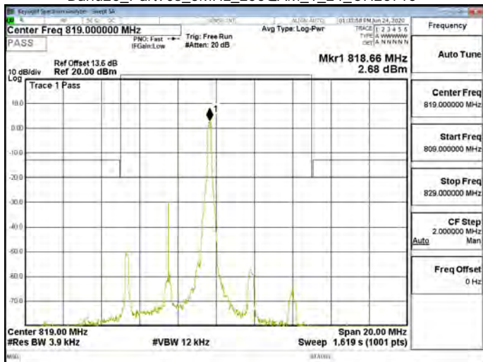
Band26_Part90s_5MHz_256QAM_1_24_CH26740
