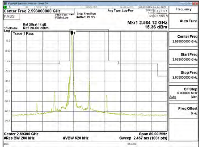
Band41_20MHz_256QAM_1_0_CH41490
