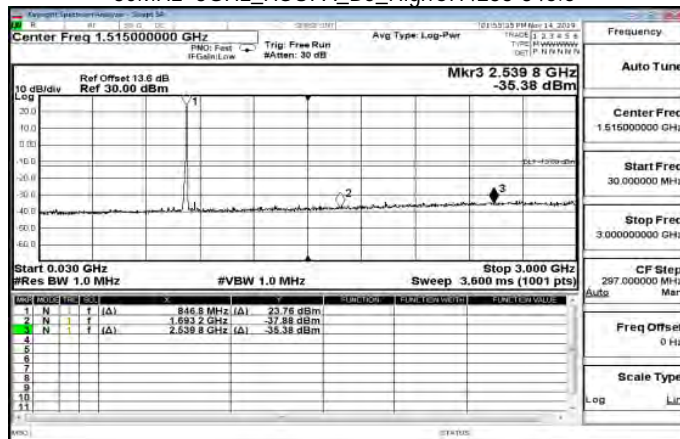
30MHz-3GHz_HSUPA_B5_HighCH4233-846.6
