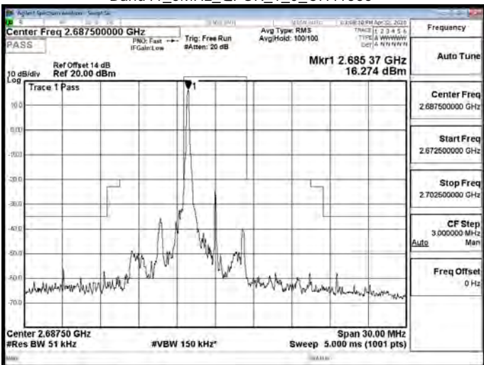
Band41_5MHz_QPSK_1_0_CH41565
