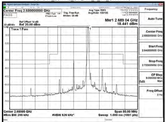
Band41_20MHz_64QAM_1_99_CH41490
