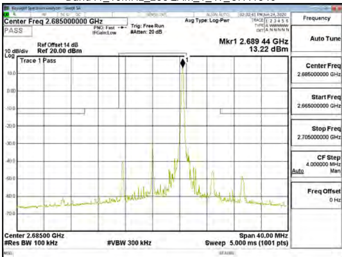
Band41_10MHz_256QAM_1_49_CH41540
