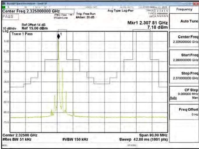
Band30_5MHz_64QAM_1_24_CH27710
