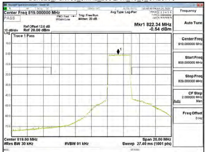
Band26_Part90s_3MHz_256QAM_15_0_CH26775
