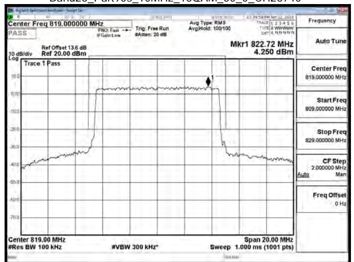
Band26_Part90s_10MHz_16QAM_50_0_CH26740
