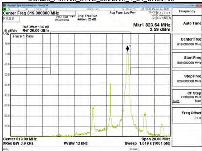
Band26_Part90s_5MHz_256QAM_1_24_CH26765
