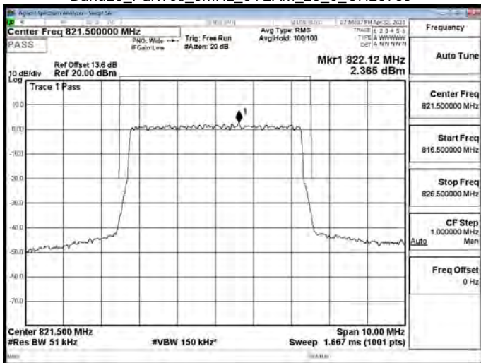
Band26_Part90s_5MHz_64QAM_25_0_CH26765
