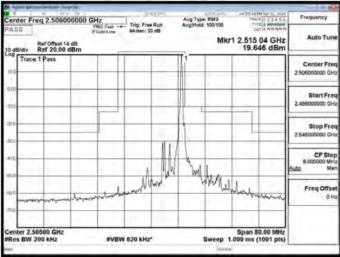
Band41_20MHz_16QAM_1_99_CH40620
