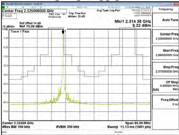
Band30_10MHz_64QAM_50_0_CH27710
