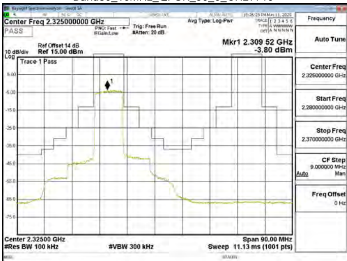
Band30_10MHz_QPSK_50_0_CH27710
