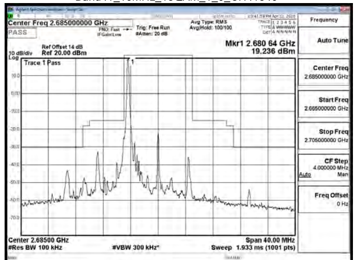
Band41_10MHz_16QAM_1_0_CH41540
