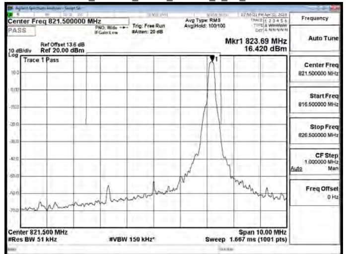
Band26_Part90s_5MHz_64QAM_1_24_CH26765
