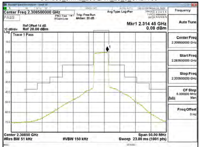
Band30_5MHz_256QAM_25_0_CH27735
