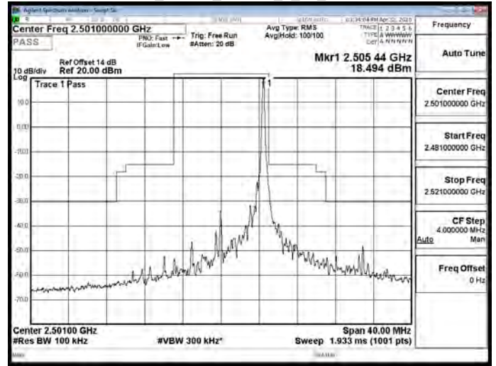
Band41_10MHz_64QAM_1_49_CH40620
