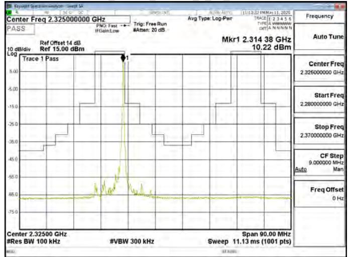
Band30_10MHz_16QAM_50_0_CH27710
