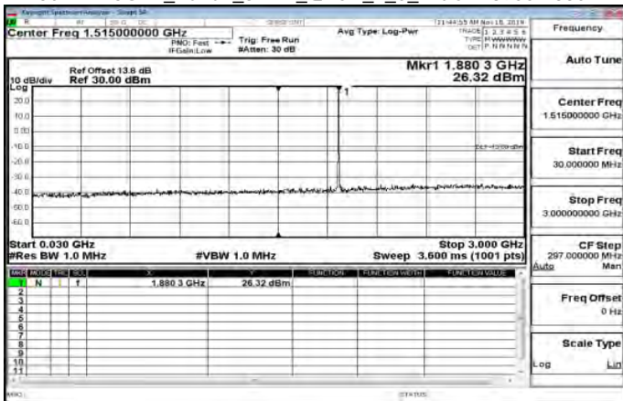
30MHz-3GHz_Band2_3MHz_QPSK_1_0_MidCH1890-1880
