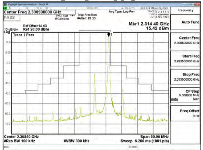
Band30_10MHz_256QAM_50_0_CH27710
