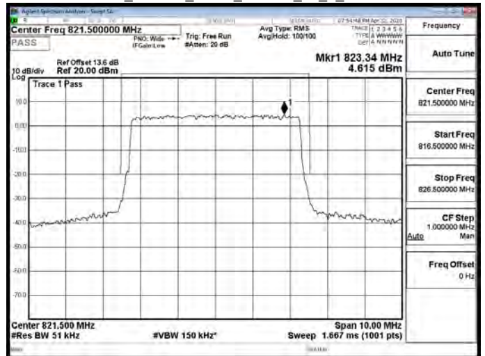
Band26_Part90s_5MHz_16QAM_25_0_CH26765
