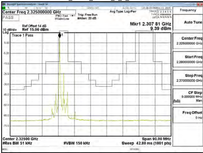
Band30_5MHz_QPSK_1_24_CH27710
