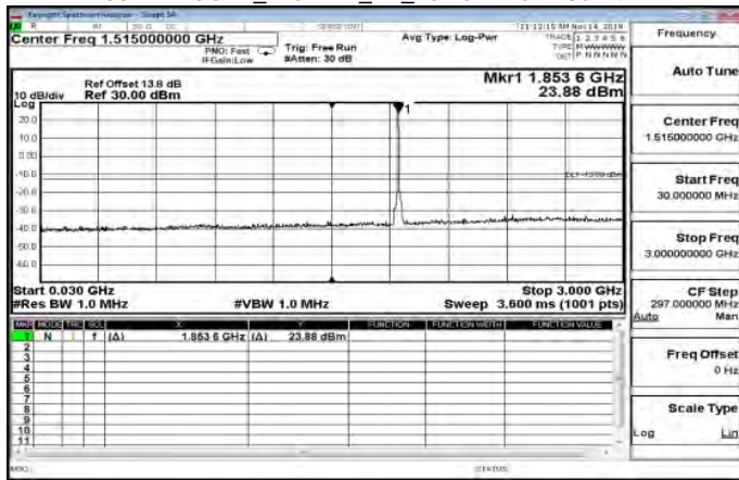
30MHz~3GHz_WCDMA_B2_LowCH9262-1852.4
