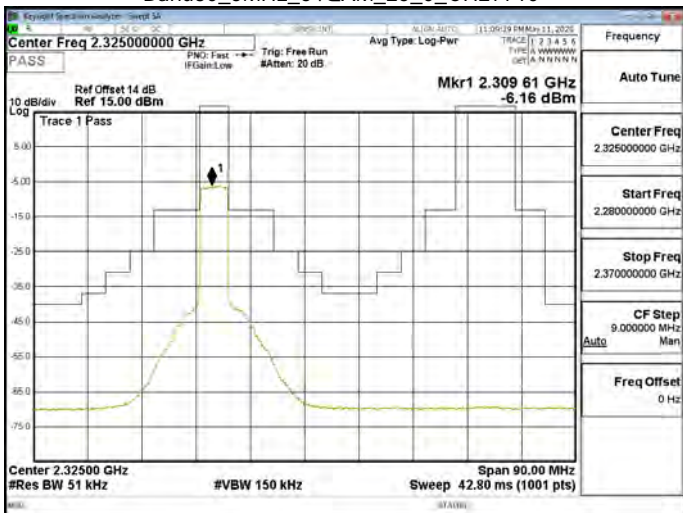
Band30_5MHz_64QAM_25_0_CH27710
