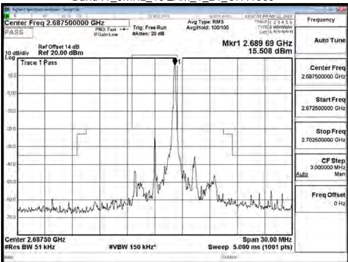
Band41_5MHz_16QAM_1_24_CH41565
