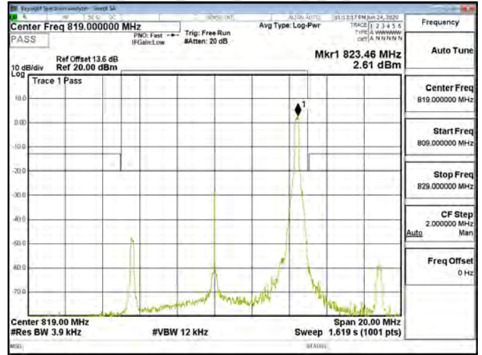
Band26_Part90s_10MHz_256QAM_50_0_CH26740
