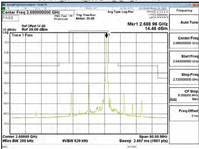
Band41_20MHz_256QAM_1_99_CH41490
