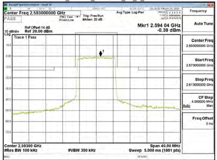
Band41_10MHz_256QAM_50_0_CH41540
