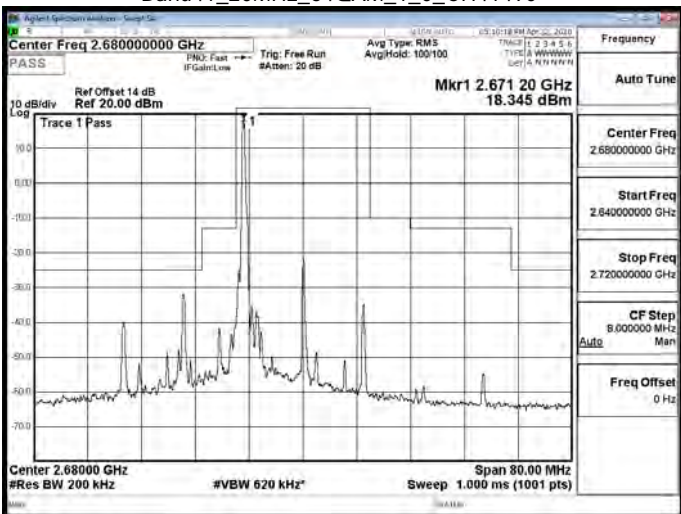
Band41_20MHz_64QAM_1_0_CH41490
