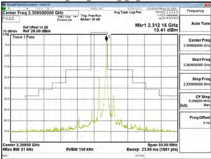
Band30_5MHz_256QAM_1_24_CH27735
