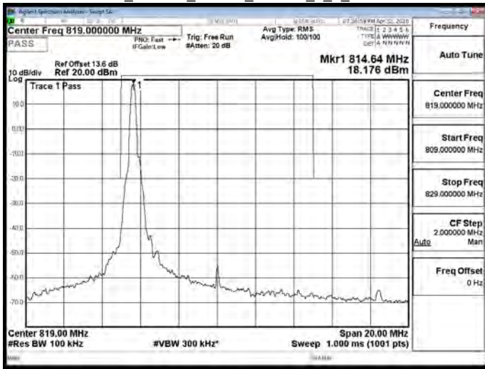
Band26_Part90s_10MHz_64QAM_1_49_CH26740
