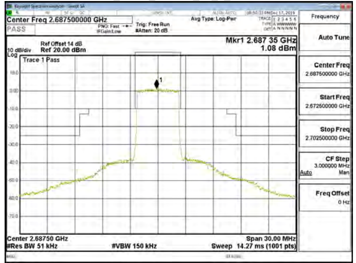
Band41_5MHz_16QAM_25_0_CH41565
