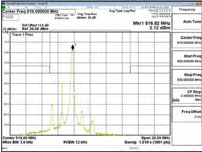
Band26_Part90s_3MHz_256QAM_1_14_CH26740
