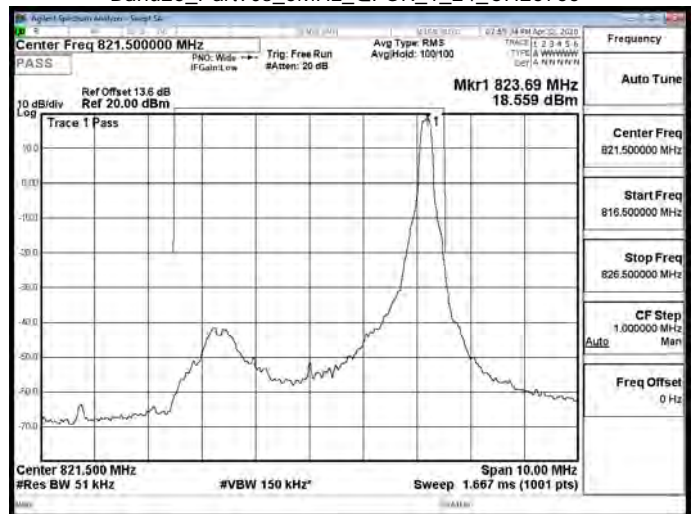
Band26_Part90s_5MHz_QPSK_1_24_CH26765
