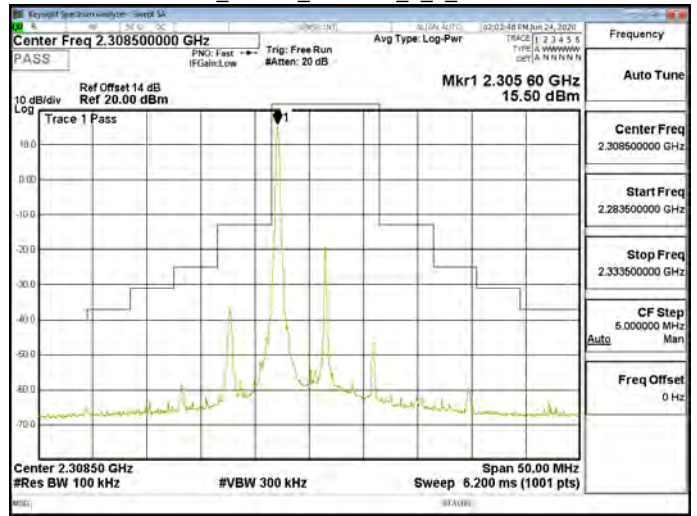
Band30_10MHz_256QAM_1_49_CH27710
