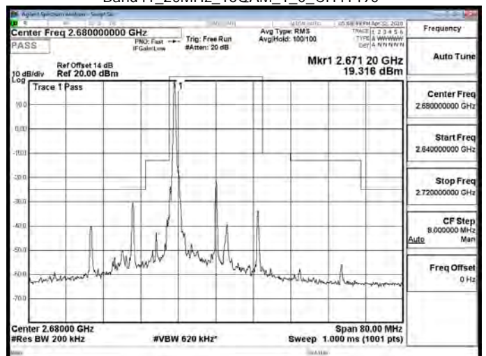
Band41_20MHz_16QAM_1_0_CH41490
