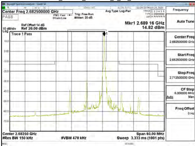
Band41_15MHz_256QAM_1_74_CH41515
