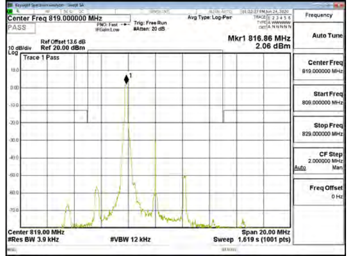
Band26_Part90s_5MHz_256QAM_1_0_CH26765
