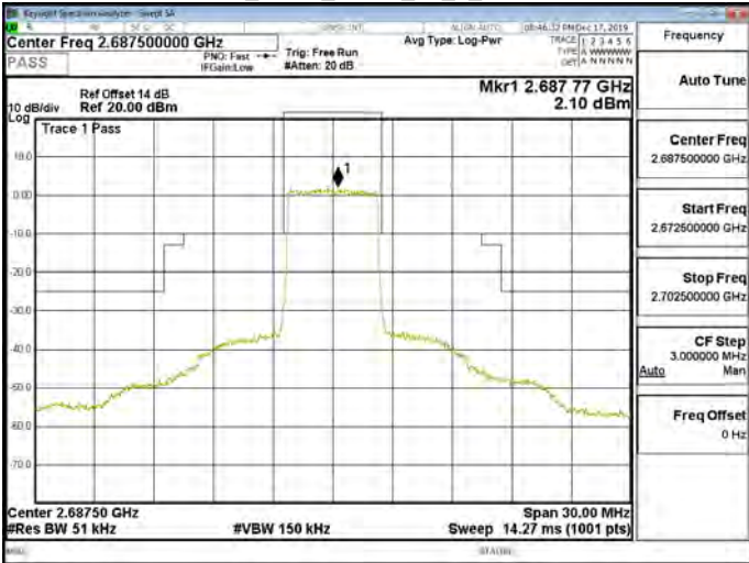
Band41_5MHz_QPSK_25_0_CH41565
