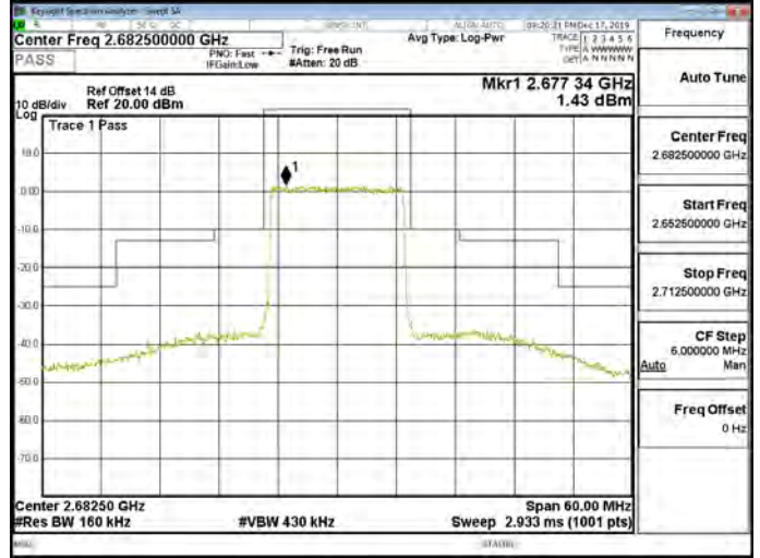
Band41_15MHz_16QAM_75_0_CH41515
