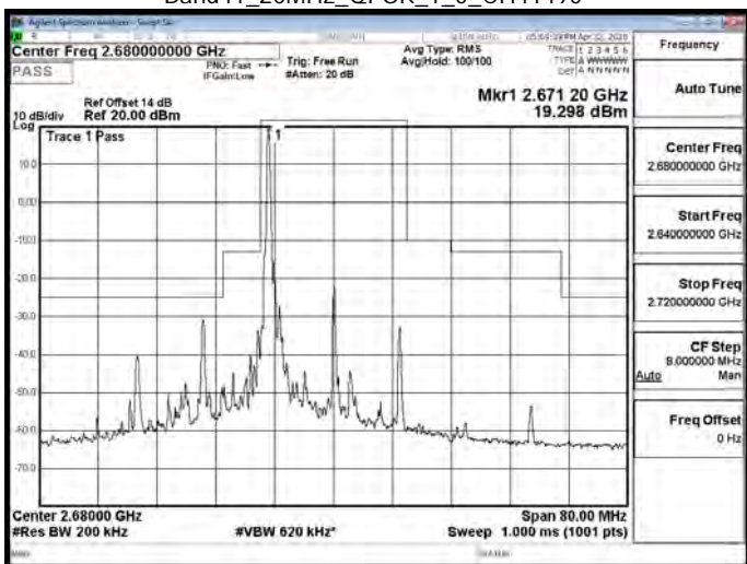
Band41_20MHz_QPSK_1_0_CH41490
