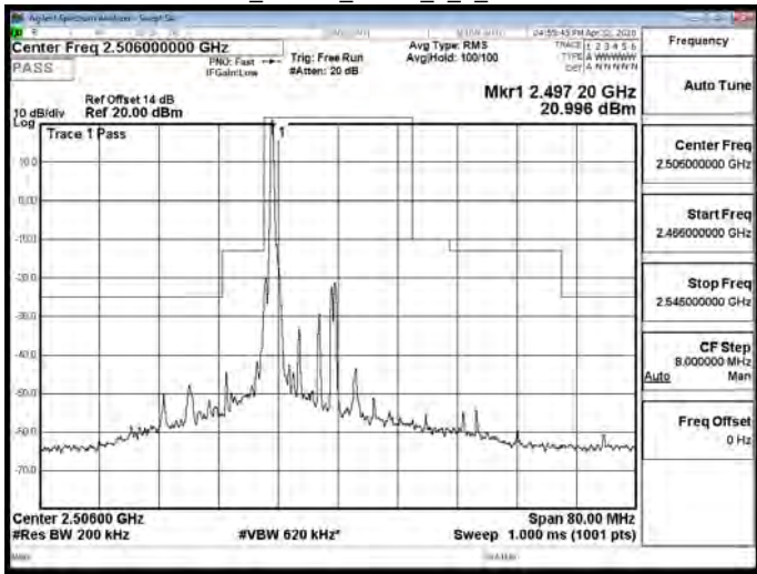
Band41_20MHz_QPSK_1_0_CH40620
