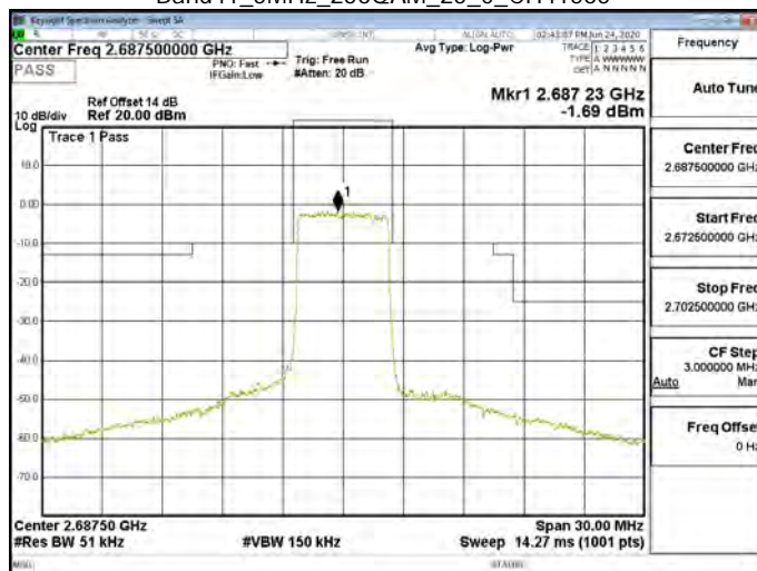
Band41_5MHz_256QAM_25_0_CH41565
