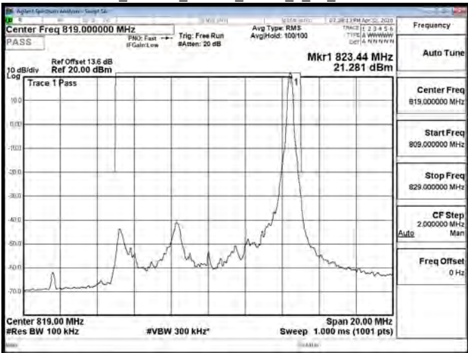
Band26_Part90s_10MHz_QPSK_50_0_CH26740
