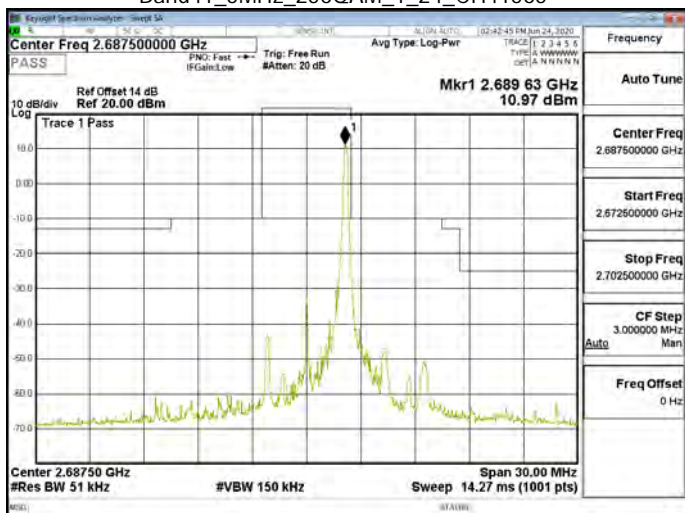
Band41_5MHz_256QAM_1_24_CH41565
