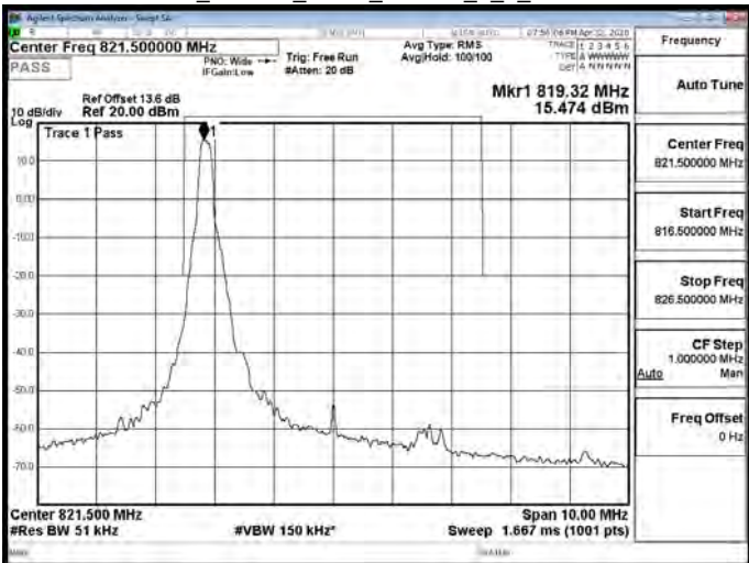
Band26_Part90s_5MHz_64QAM_1_0_CH26765
