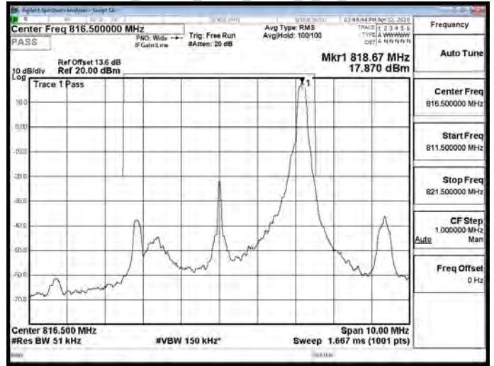
Band26_Part90s_5MHz_QPSK_1_24_CH26740
