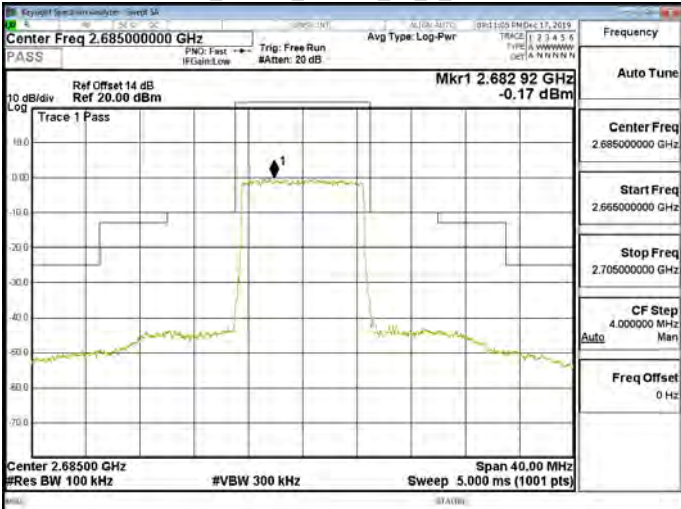
Band41_10MHz_64QAM_50_0_CH41540
