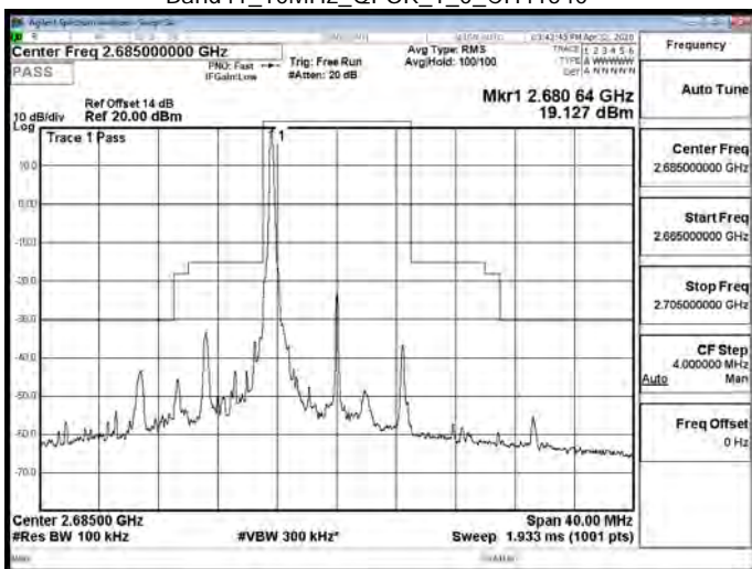
Band41_10MHz_QPSK_1_0_CH41540
