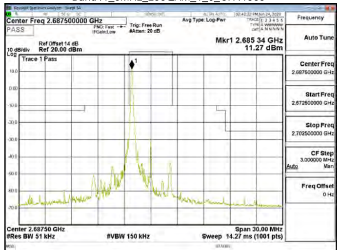
Band41_5MHz_256QAM_1_0_CH41565
