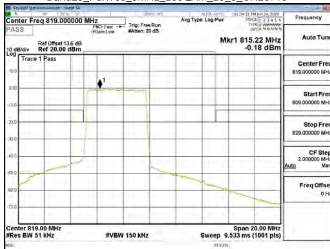
Band26_Part90s_5MHz_256QAM_25_0_CH26740
