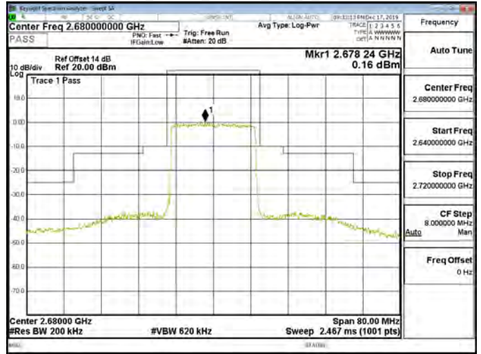
Band41_20MHz_16QAM_100_0_CH41490
