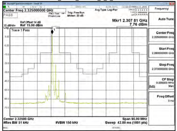
Band30_5MHz_16QAM_1_24_CH27710
