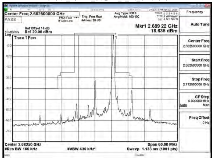
Band41_15MHz_64QAM_1_74_CH41515
