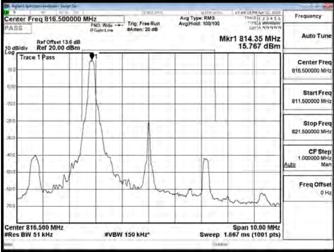
Band26_Part90s_5MHz_64QAM_1_0_CH26740
