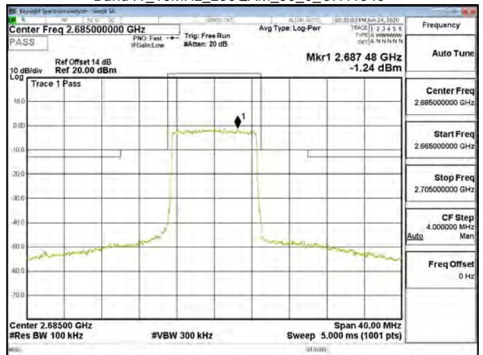
Band41_10MHz_256QAM_50_0_CH41540
