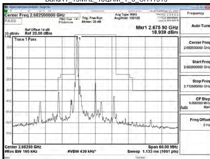
Band41_15MHz_16QAM_1_0_CH41515
