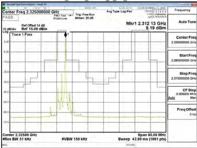
Band30_5MHz_QPSK_25_0_CH27710
