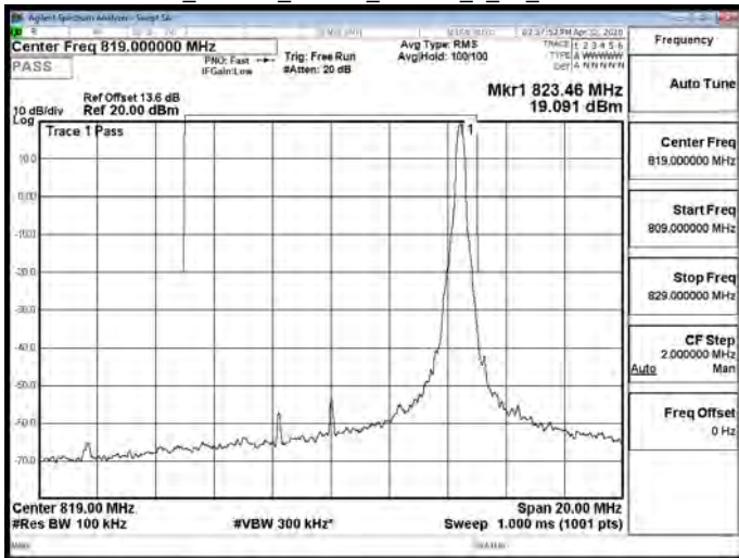
Band26_Part90s_10MHz_64QAM_50_0_CH26740
