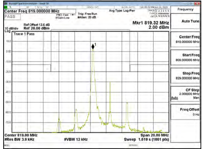
Band26_Part90s_5MHz_256QAM_1_0_CH26765
