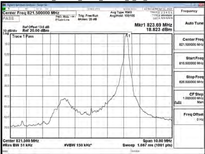
Band26_Part90s_5MHz_16QAM_1_24_CH26765
