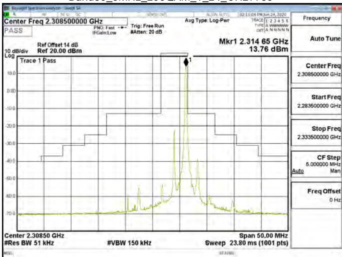
Band30_5MHz_256QAM_1_24_CH27735
