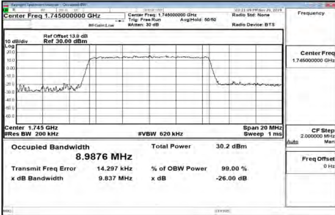
Band66_10MHz_64QAM_50_0_Main_MidCH132322-1745
