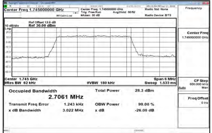
Band66_3MHz_256QAM_15_0_Main_MidCH132322-1745
