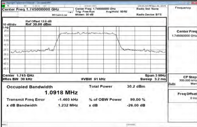
Band66_1_4MHz_QPSK_6_0_Main_MidCH132322-1745
