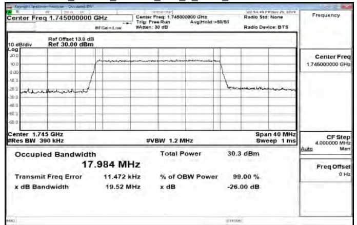
Band66_20MHz_16QAM_100_0_Main_MidCH132322-1745
