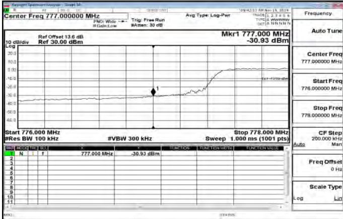
LTE\Band13_10MHz_QPSK_50_0_LowCH23230-782
