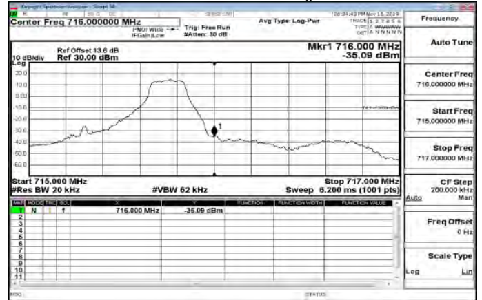
LTEBand12_1_4MHz_QPSK_1_5_HighCH23173-715.3
