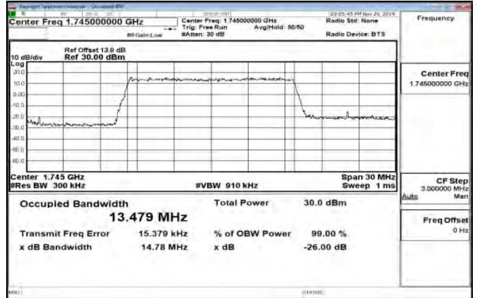
Band66_15MHz_16QAM_75_0_Main_MidCH132322-1745
