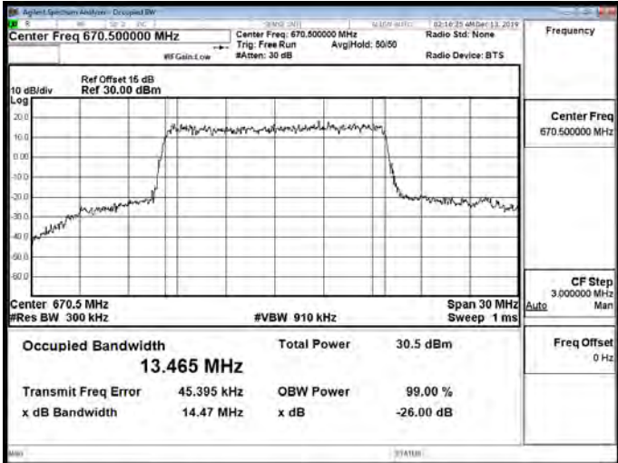
Band71_15MHz_QPSK_75_0_Main_Low CH133197-670.5
