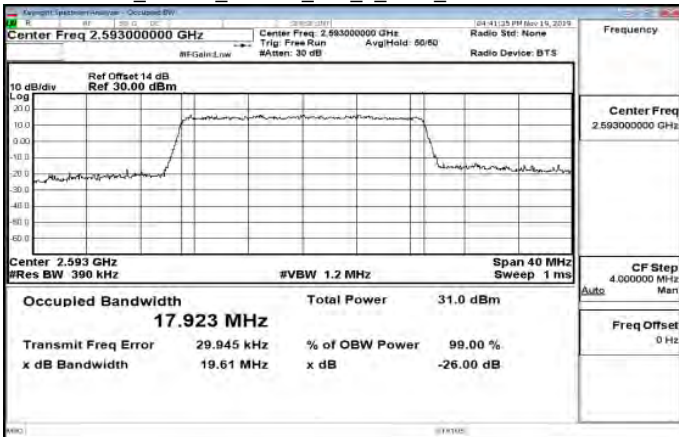
Band41_20MHz_64QAM_100_0_Main_MidCH40620-2593
