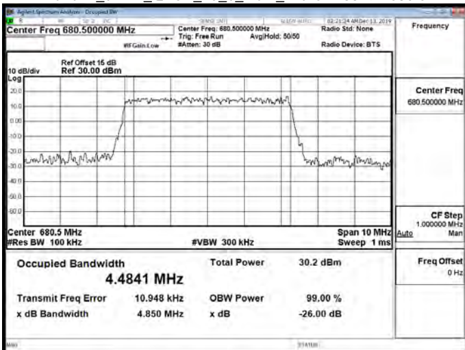
Band71_5MHz_QPSK_25_0_Main_MidCH133297-680.5
