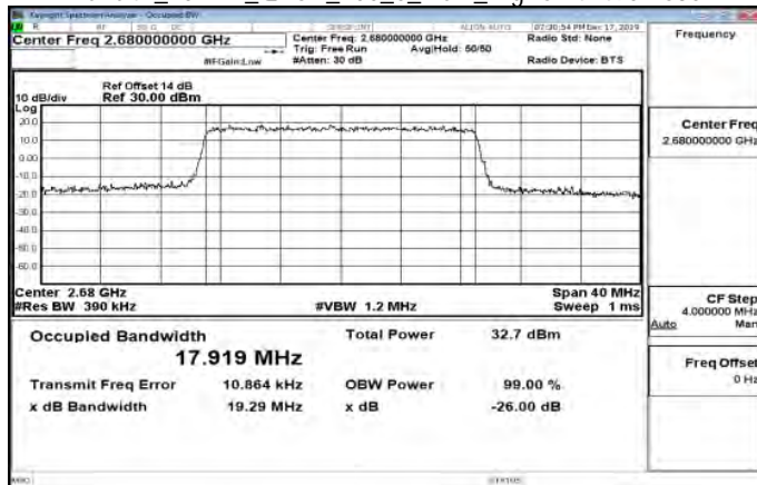
Band41_20MHz_QPSK_100_0_Main_HighCH41490-2680
