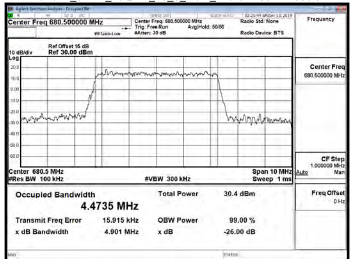
Band71_5MHz_16QAM_25_0_Main_MidCH133297-680.5
