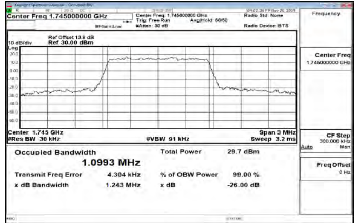
Band66_1_4MHz_16QAM_6_0_Main_MidCH132322-1745
