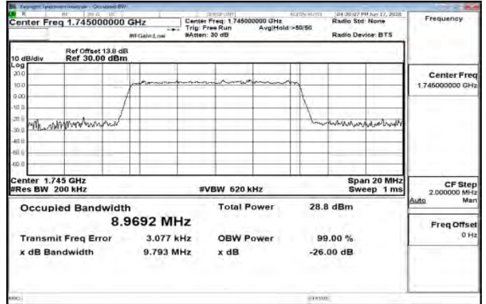
Band66_10MHz_256QAM_50_0_Main_MidCH132322-1745
