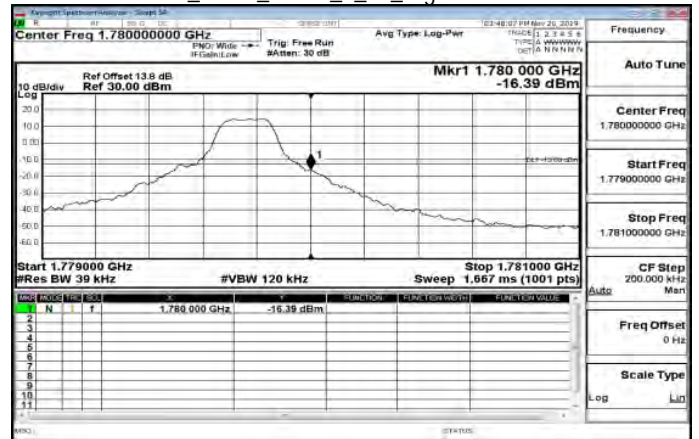
LTE\Band66_3MHz_QPSK_1_14_HighCH132657-1778.5
