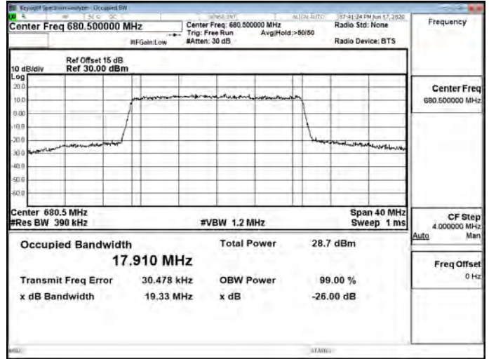
Band71_20MHz_256QAM_100_0_Main_Mid CH133297-680.5
