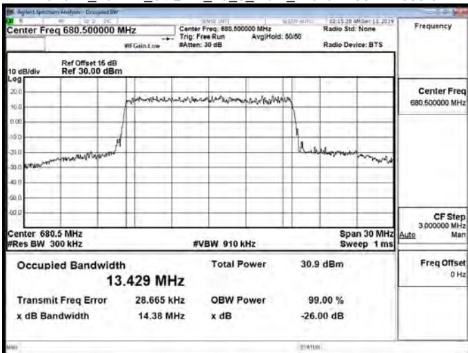
Band71_15MHz_64QAM_75_0_Main_Mid CH133297-680.5
