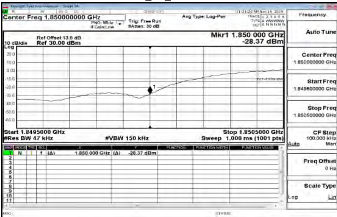
HSDPAHSDPA_B2_LowCH9262-1852.4
