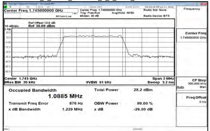
Band66_1_4MHz_256QAM_6_0_Main_MidCH132322-1745
