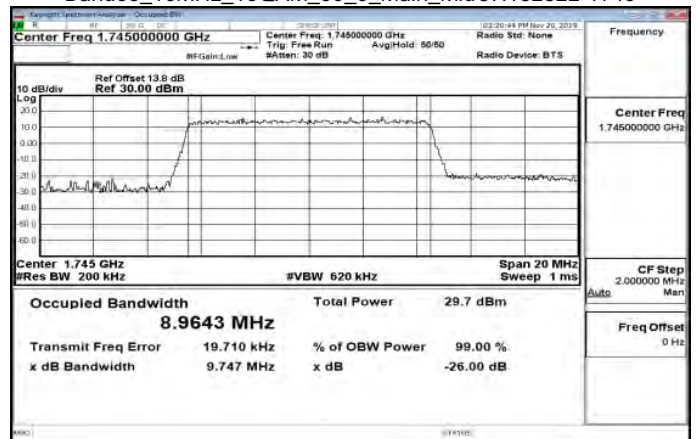
Band66_10MHz_16QAM_50_0_Main_MidCH132322-1745
