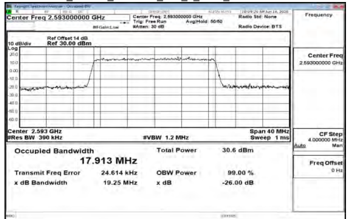
Band41_20MHz_256QAM_100_0_Main_MidCH40620-2593
