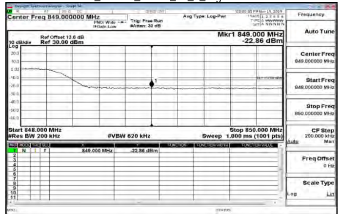
LTE\Band26_15MHz_QPSK_75_0_HighCH26965-841.5
