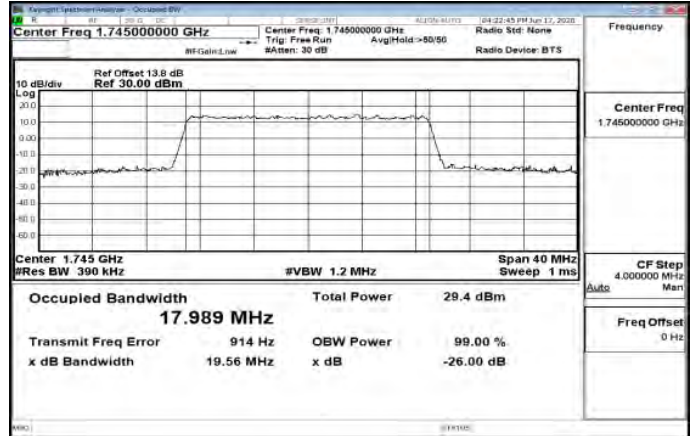
Band66_20MHz_256QAM_100_0_Main_MidCH132322-1745
