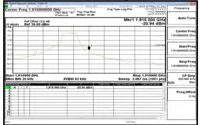
LTE\Band25_1_4MHz_QPSK_1_5_HighCH26683-1914.3
