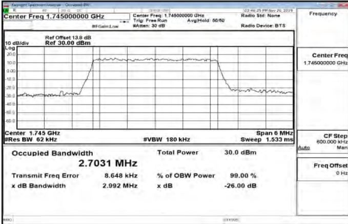
Band66_3MHz_64QAM_15_0_Main_MidCH132322-1745
