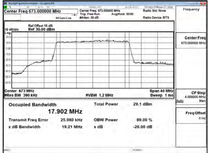
Band71_20MHz_256QAM_100_0_Main_Low CH133222-673
