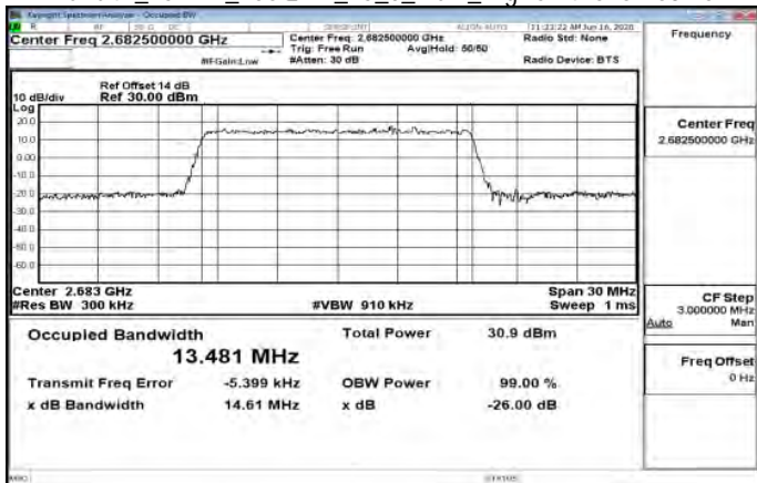
Band41_15MHz_256QAM_75_0_Main_HighCH41515-2682.5
