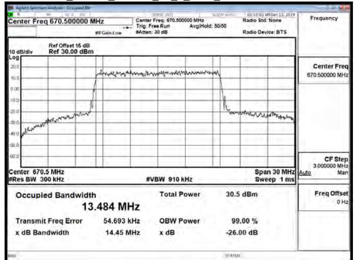
Band71_15MHz_16QAM_75_0_Main_Low CH133197-670.5
