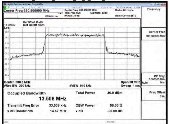
Band71_15MHz_16QAM_75_0_Main_Mid CH133297-680.5
