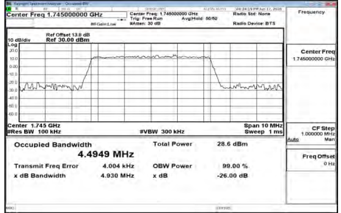
Band66_5MHz_256QAM_25_0_Main_MidCH132322-1745
