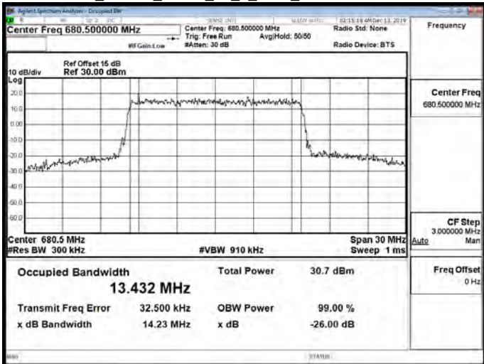
Band71_15MHz_QPSK_75_0_Main_Mid CH133297-680.5
