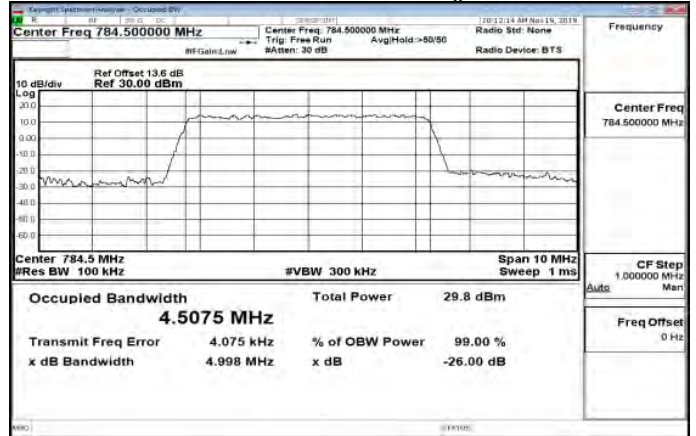
Band13_5MHz_64QAM_25_0_Main_HighCH23255-784.5
