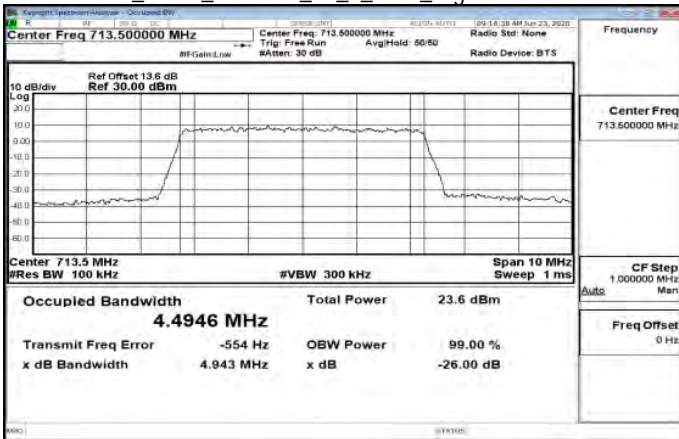
Band12_5MHz_256QAM_25_0_Main_HighCH23155-713.5
