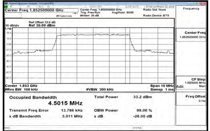
Band25_5MHz_QPSK_25_0_Main_LowCH26065-1852.5
