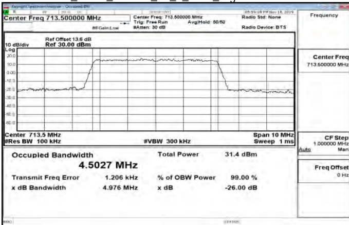
Band12_5MHz_16QAM_25_0_Main_HighCH23155-713.5
