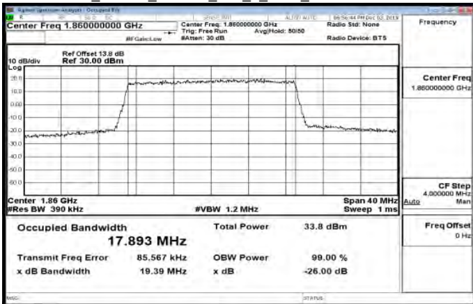
Band25_20MHz_16QAM_100_0_Main_LowCH26140-1860
