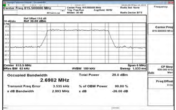
Band26_Part90s_3MHz_64QAM_15_0_Main_LowCH26705-815.5
