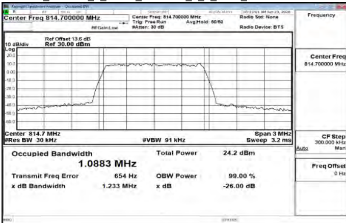
Band26_Part90s_1_4MHz_256QAM_6_0_Main_LowCH26697-814.7
