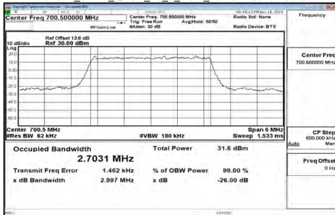
Band12_3MHz_QPSK_15_0_Main_LowCH23025-700.5
