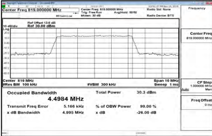
Band26_Part90s_5MHz_QPSK_25_0_Main_MidCH26740-819
