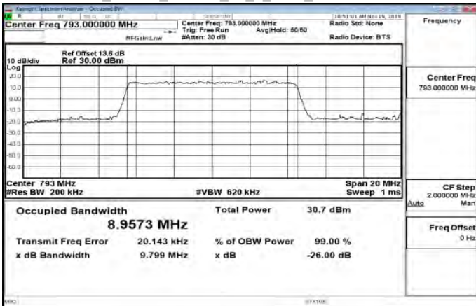
Band14_10MHz_16QAM_50_0_Main_MidCH23330-793
