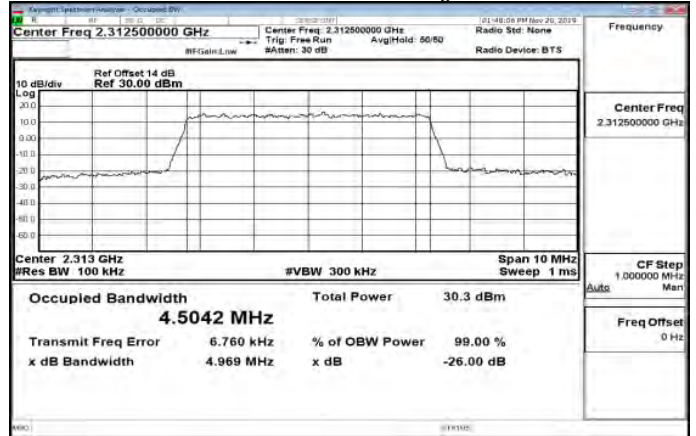
Band30_5MHz_QPSK_25_0_Main_HighCH27735-2312.5
