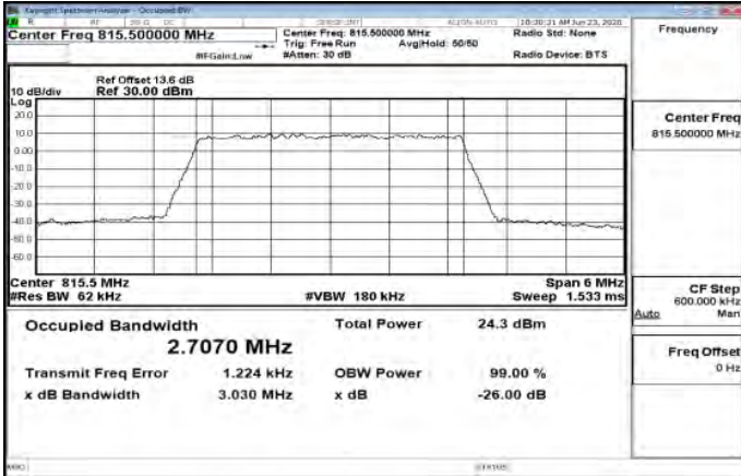
Band26_Part90s_3MHz_256QAM_15_0_Main_LowCH26705-815.5
