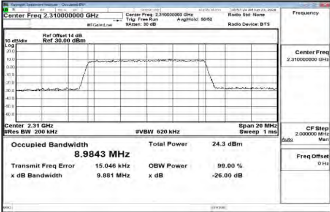
Band30_10MHz_256QAM_50_0_Main_MidCH27710-2310
