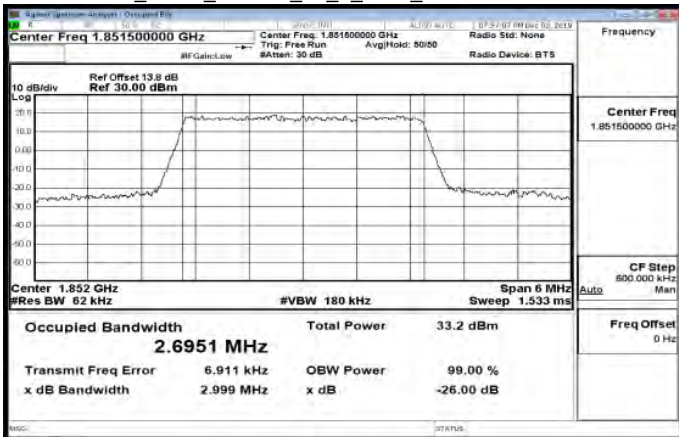
Band25_3MHz_16QAM_15_0_Main_LowCH26055-1851.5
