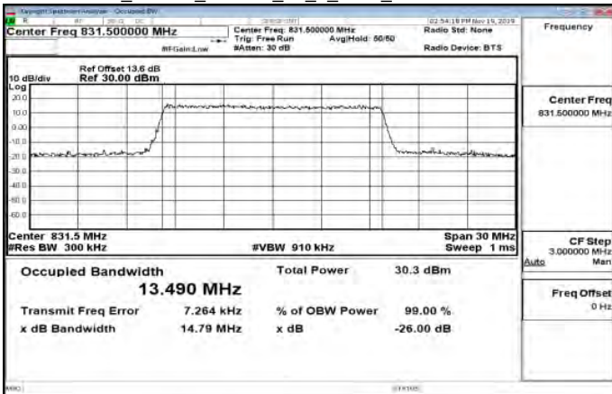
Band26_15MHz_16QAM_75_0_Main_LowCH26865-831.5
