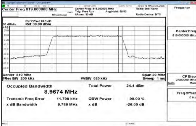
Band26_Part90s_10MHz_256QAM_50_0_Main_MidCH26740-819
