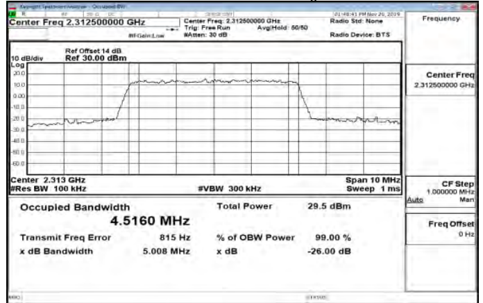
Band30_5MHz_64QAM_25_0_Main_HighCH27735-2312.5
