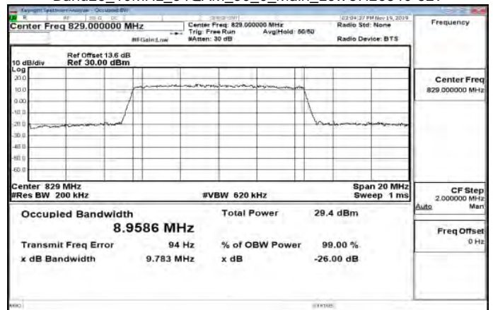
Band26_10MHz_64QAM_50_0_Main_LowCH26840-829
