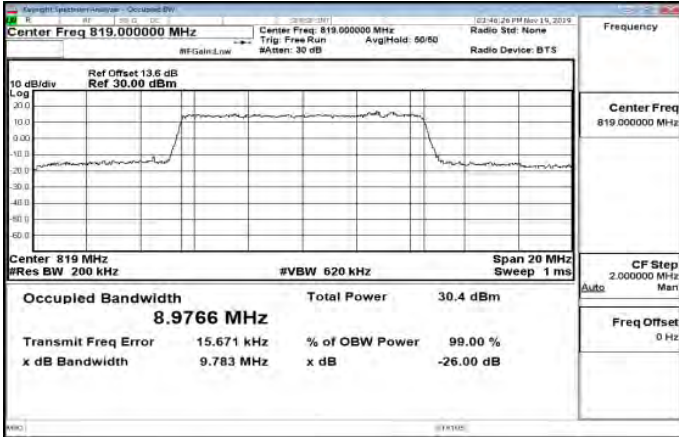
Band26_Part90s_10MHz_64QAM_50_0_Main_MidCH26740-819
