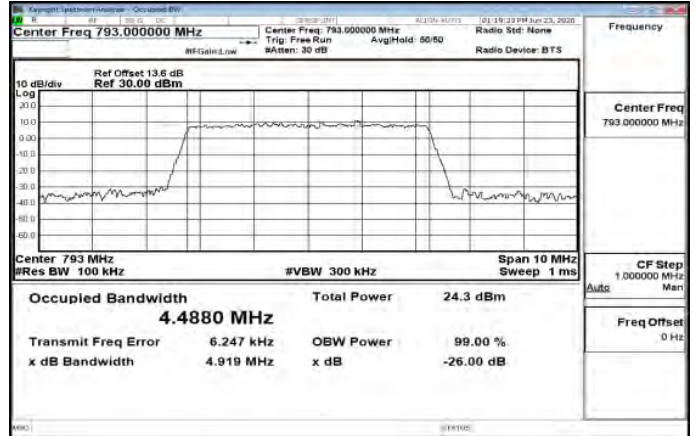
Band14_5MHz_256QAM_25_0_Main_MidCH23330-793
