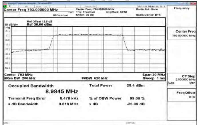
Band14_10MHz_256QAM_50_0_Main_MidCH23330-793
