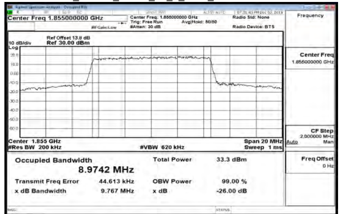
Band25_10MHz_QPSK_50_0_Main_LowCH26090-1855
