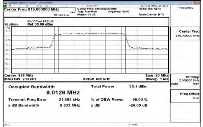
Band26_Part90s_10MHz_QPSK_50_0_Main_MidCH26740-819
