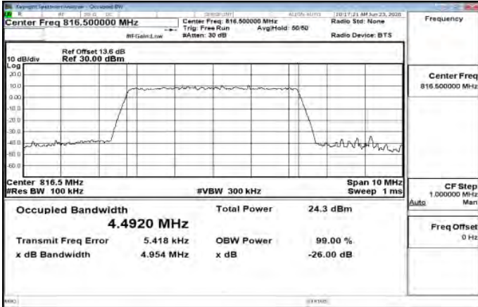
Band26_Part90s_5MHz_256QAM_25_0_Main_LowCH26715-816.5
