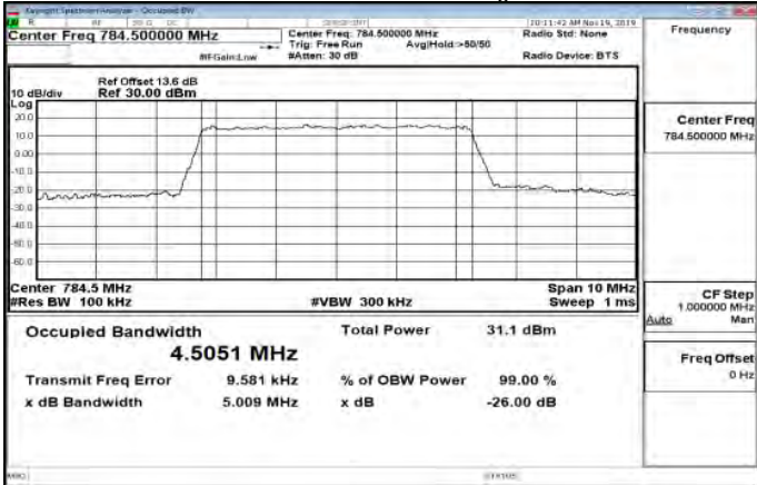
Band13_5MHz_16QAM_25_0_Main_HighCH23255-784.5
