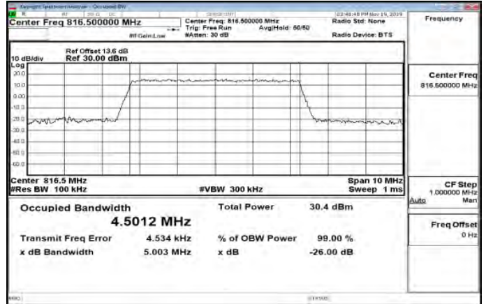
Band26_Part90s_5MHz_QPSK_25_0_Main_LowCH26715-816.5
