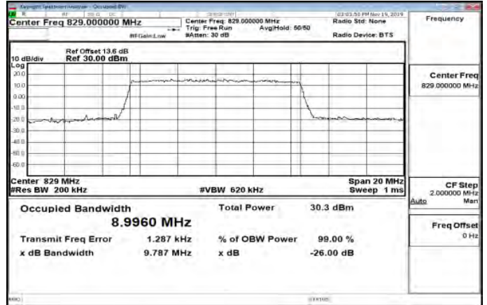
Band26_10MHz_QPSK_50_0_Main_LowCH26840-829
