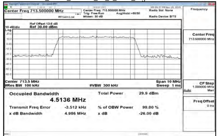
Band12_5MHz_64QAM_25_0_Main_HighCH23155-713.5
