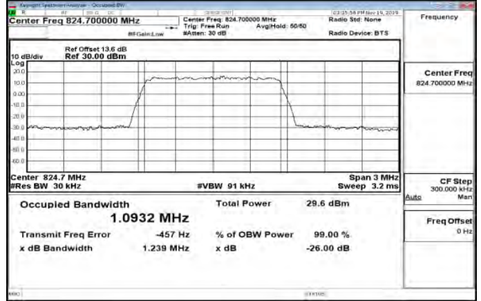
Band26_1_4MHz_QPSK_6_0_Main_LowCH26797-824.7
