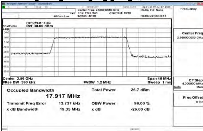
Band7_20MHz_256QAM_100_0_Main_HighCH21350-2560
