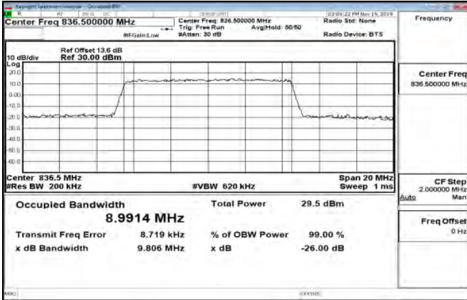
Band26_10MHz_64QAM_50_0_Main_MidCH26915-836.5
