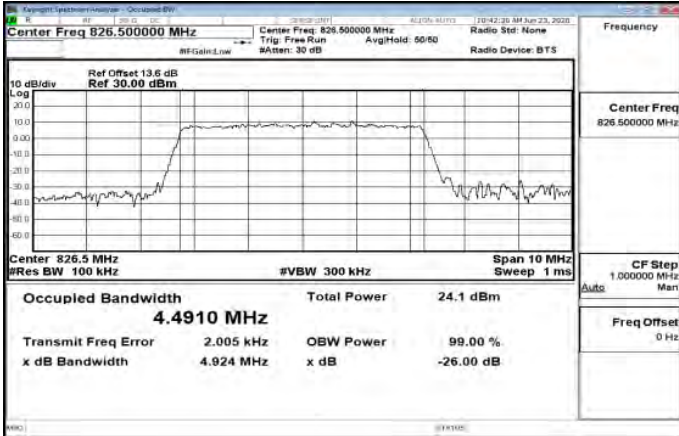
Band26_5MHz_256QAM_25_0_Main_LowCH26815-826.5
