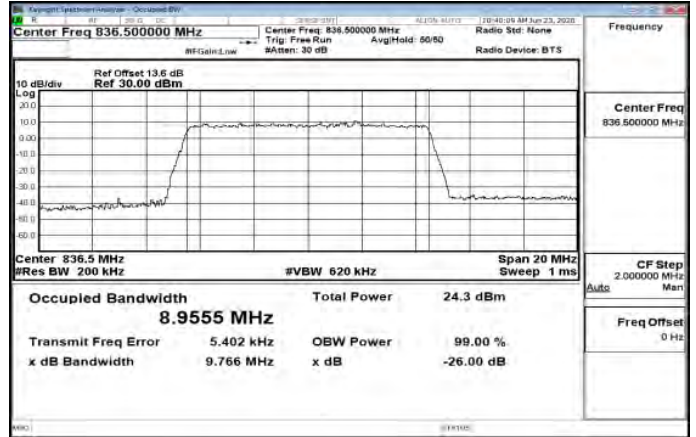
Band26_10MHz_256QAM_50_0_Main_MidCH26915-836.5
