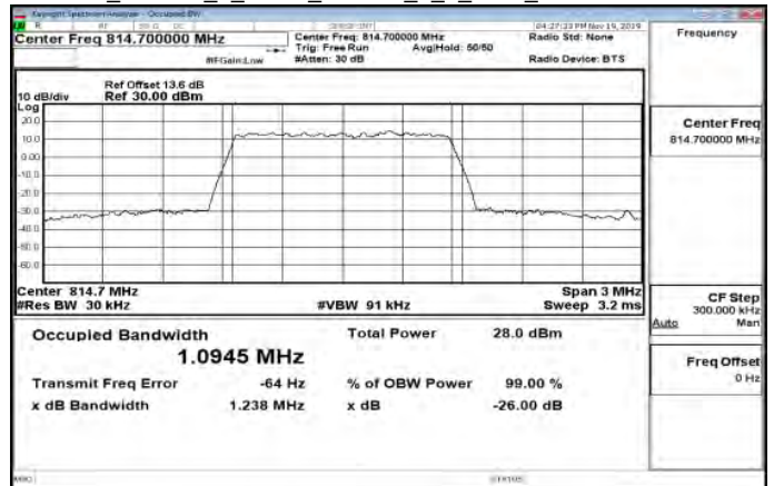
Band26_Part90s_1_4MHz_64QAM_6_0_Main_LowCH26697-814.7
