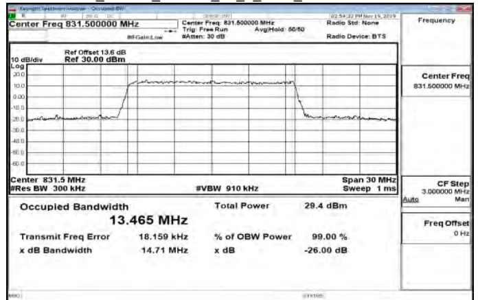
Band26_15MHz_64QAM_75_0_Main_LowCH26865-831.5
