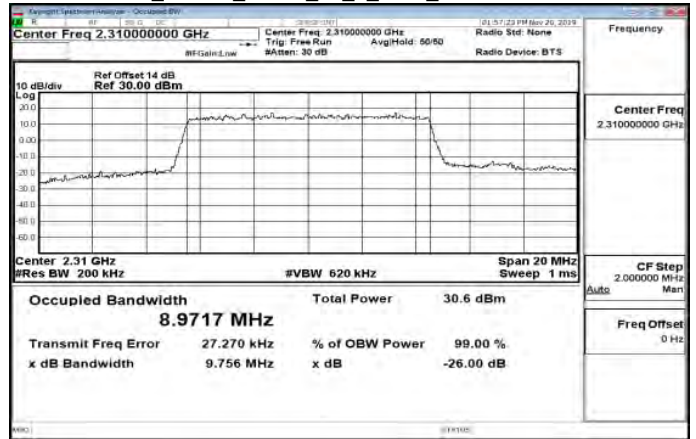
Band30_10MHz_16QAM_50_0_Main_MidCH27710-2310
