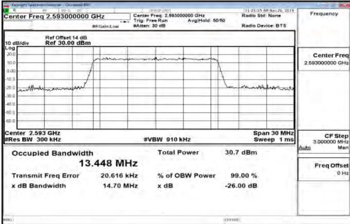
Band41_15MHz_64QAM_75_0_Main_MidCH40620-2593
