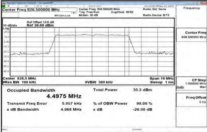
Band26_5MHz_16QAM_25_0_Main_LowCH26815-826.5
