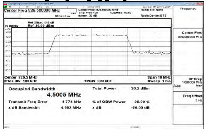
Band26_5MHz_QPSK_25_0_Main_LowCH26815-826.5
