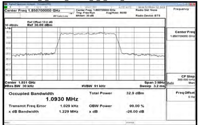
Band25_1_4MHz_64QAM_6_0_Main_LowCH26047-1850.7
