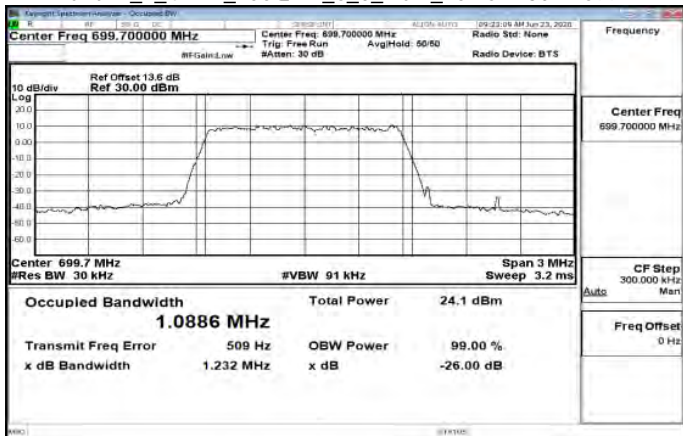
Band12_1_4MHz_256QAM_6_0_Main_LowCH23017-699.7
