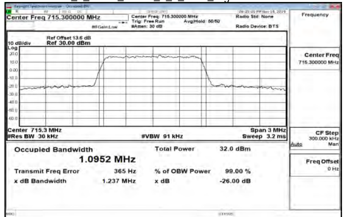
Band12_1_4MHz_QPSK_6_0_Main_HighCH23173-715.3
