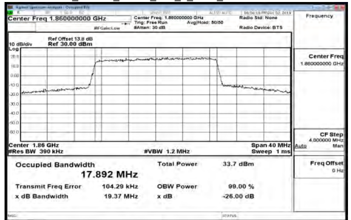
Band25_20MHz_QPSK_100_0_Main_LowCH26140-1860
