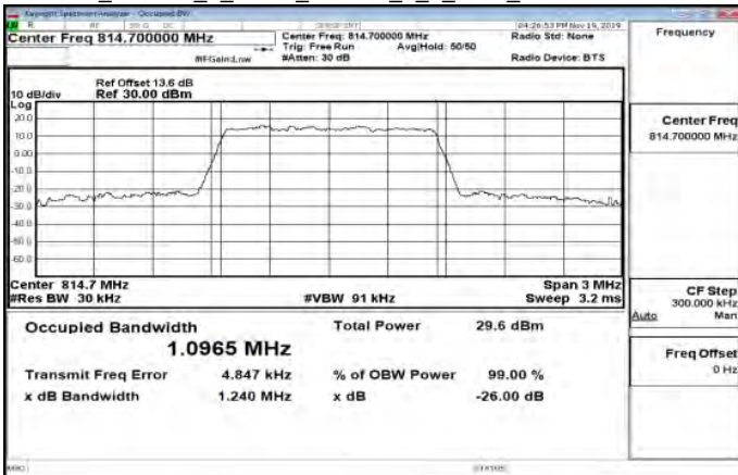
Band26_Part90s_1_4MHz_16QAM_6_0_Main_LowCH26697-814.7
