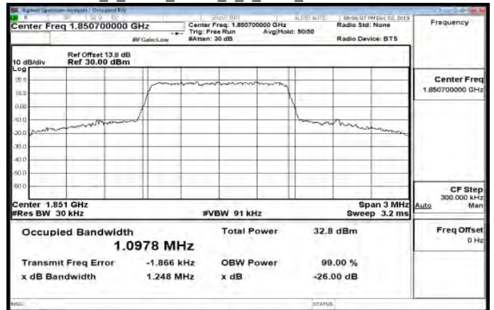
Band25_1_4MHz_QPSK_6_0_Main_LowCH26047-1850.7
