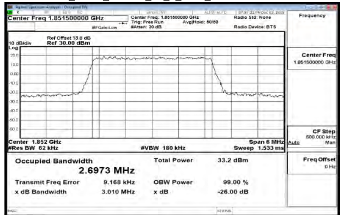
Band25_3MHz_64QAM_15_0_Main_LowCH26055-1851.5
