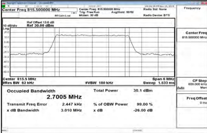
Band26_Part90s_3MHz_16QAM_15_0_Main_LowCH26705-815.5
