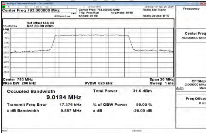
Band14_10MHz_16QAM_50_0_Main_MidCH23330-793
