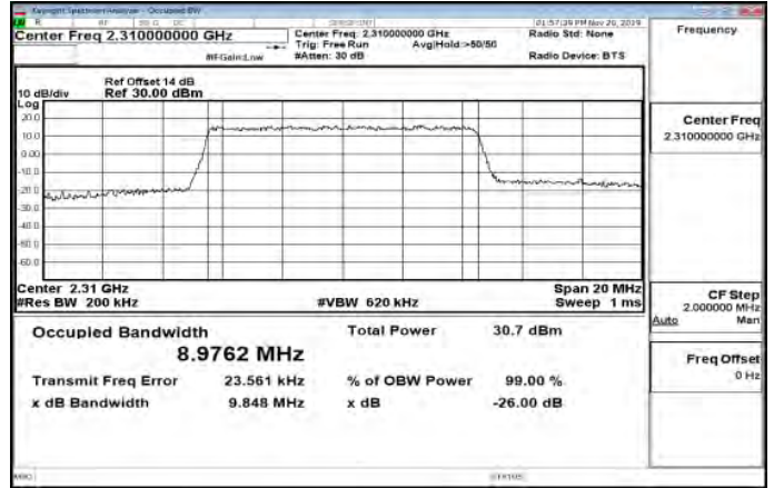
Band30_10MHz_64QAM_50_0_Main_MidCH27710-2310
