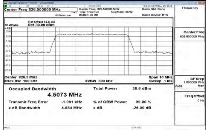
Band26_5MHz_64QAM_25_0_Main_LowCH26815-826.5
