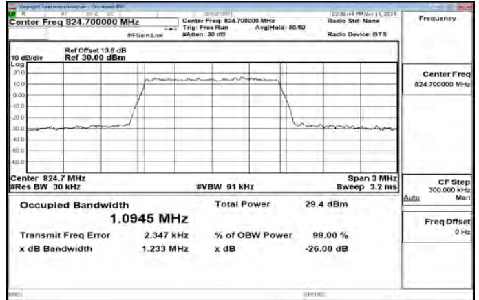
Band26_1_4MHz_64QAM_6_0_Main_LowCH26797-824.7
