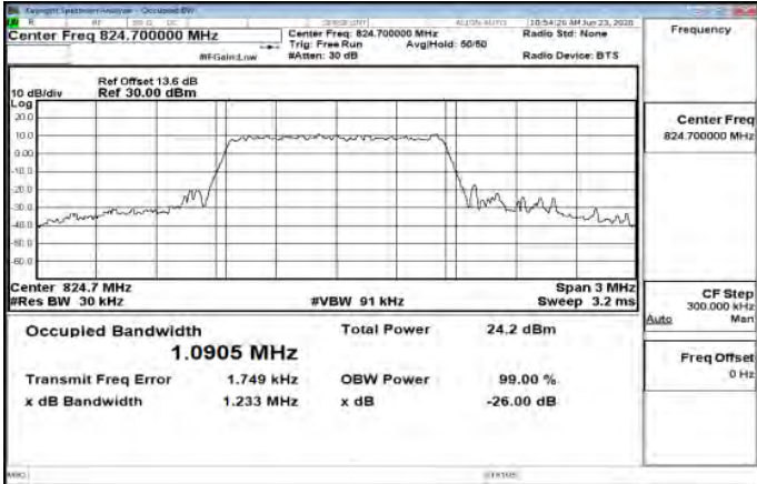
Band26_1_4MHz_256QAM_6_0_Main_LowCH26797-824.7
