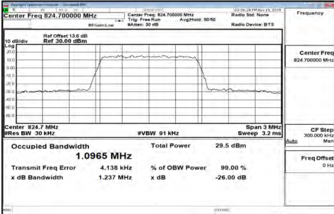
Band26_1_4MHz_16QAM_6_0_Main_LowCH26797-824.7
