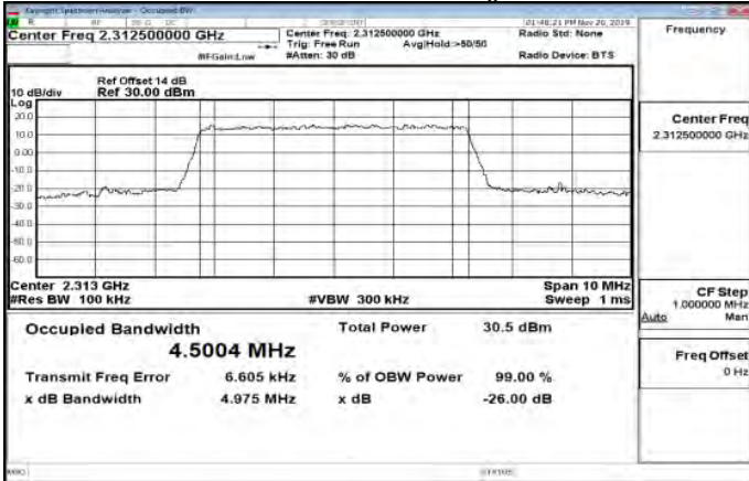
Band30_5MHz_16QAM_25_0_Main_HighCH27735-2312.5
