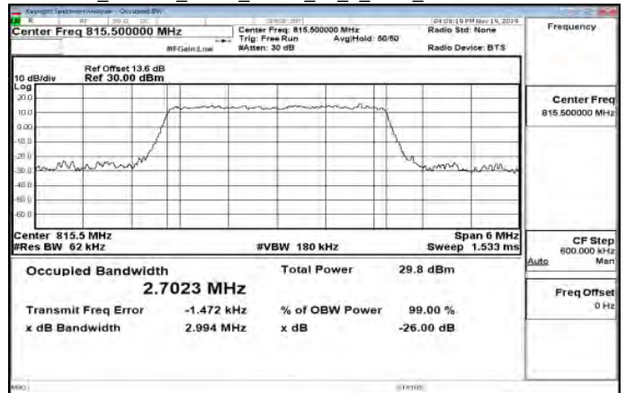
Band26_Part90s_3MHz_QPSK_15_0_Main_LowCH26705-815.5
