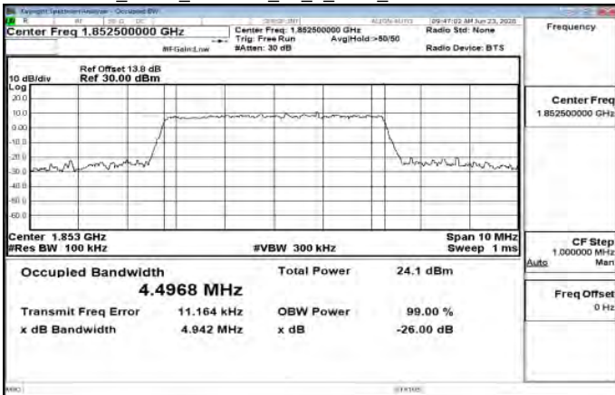
Band25_5MHz_256QAM_25_0_Main_LowCH26065-1852.5
