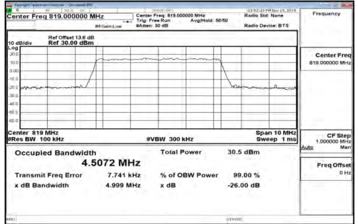
Band26_Part90s_5MHz_16QAM_25_0_Main_MidCH26740-819
