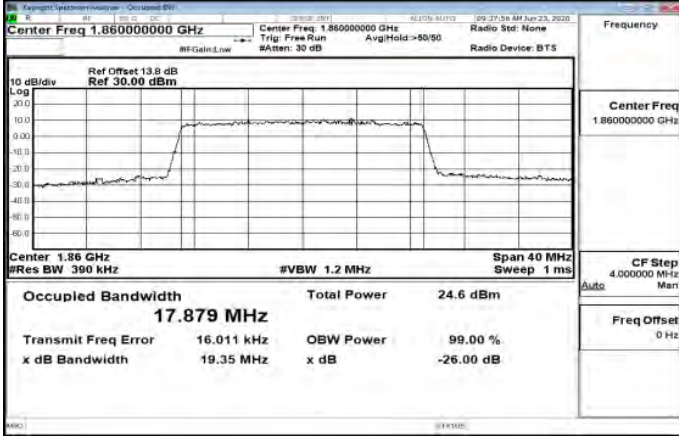
Band25_20MHz_256QAM_100_0_Main_LowCH26140-1860
