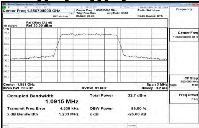
Band25_1_4MHz_16QAM_6_0_Main_LowCH26047-1850.7
