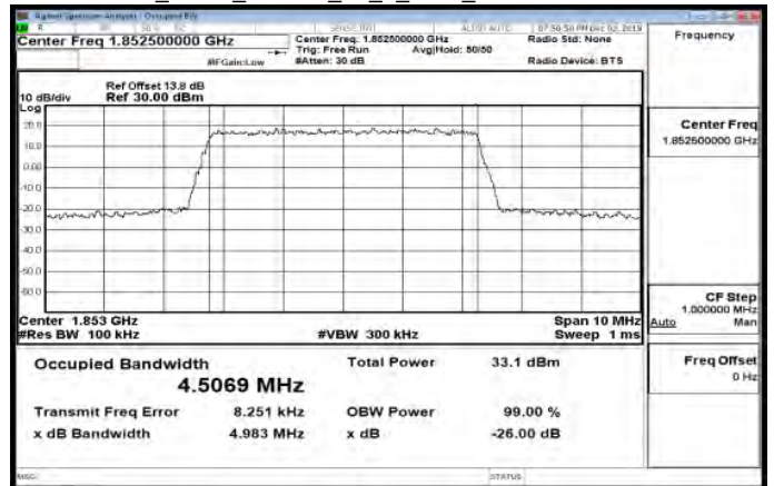
Band25_5MHz_64QAM_25_0_Main_LowCH26065-1852.5
