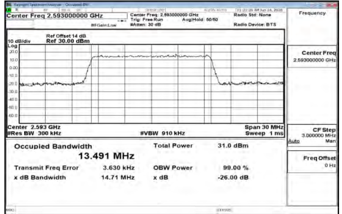
Band41_15MHz_256QAM_75_0_Main_MidCH40620-2593
