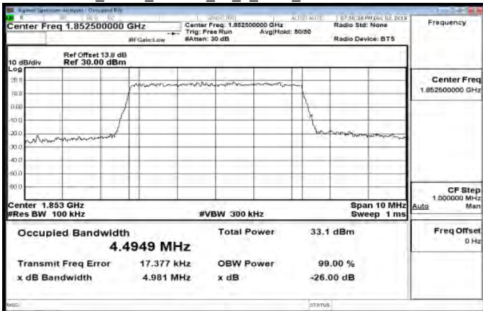
Band25_5MHz_16QAM_25_0_Main_LowCH26065-1852.5
