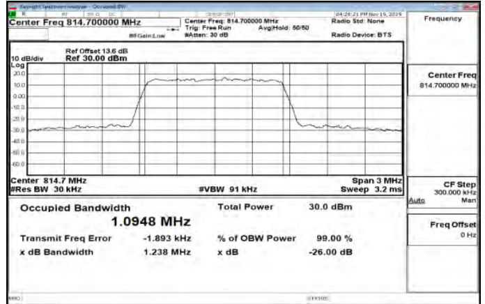
Band26_Part90s_1_4MHz_QPSK_6_0_Main_LowCH26697-814.7
