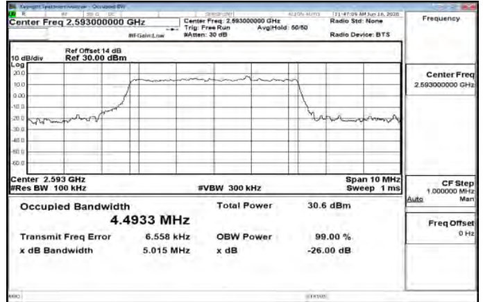
Band41_5MHz_256QAM_25_0_Main_MidCH40620-2593
