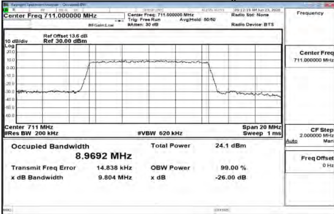
Band12_10MHz_256QAM_50_0_Main_HighCH23130-711
