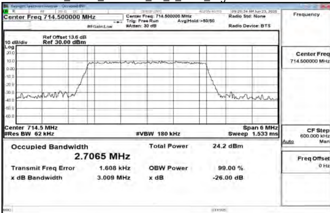
Band12_3MHz_256QAM_15_0_Main_HighCH23165-714.5
