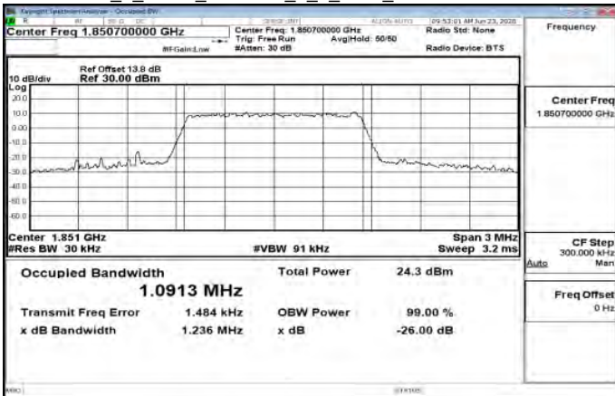
Band25_1_4MHz_256QAM_6_0_Main_LowCH26047-1850.7
