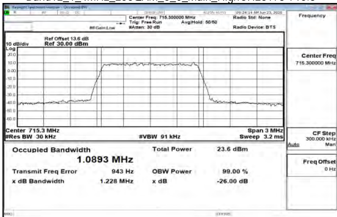
Band12_1_4MHz_256QAM_6_0_Main_HighCH23173-715.3
