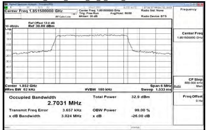
Band25_3MHz_QPSK_15_0_Main_LowCH26055-1851.5
