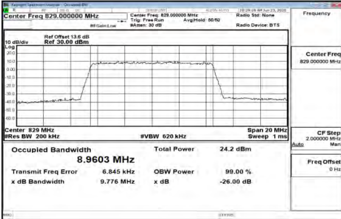
Band26_10MHz_256QAM_50_0_Main_LowCH26840-829
