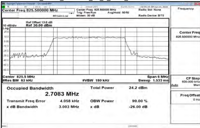
Band26_3MHz_256QAM_15_0_Main_LowCH26805-825.5
