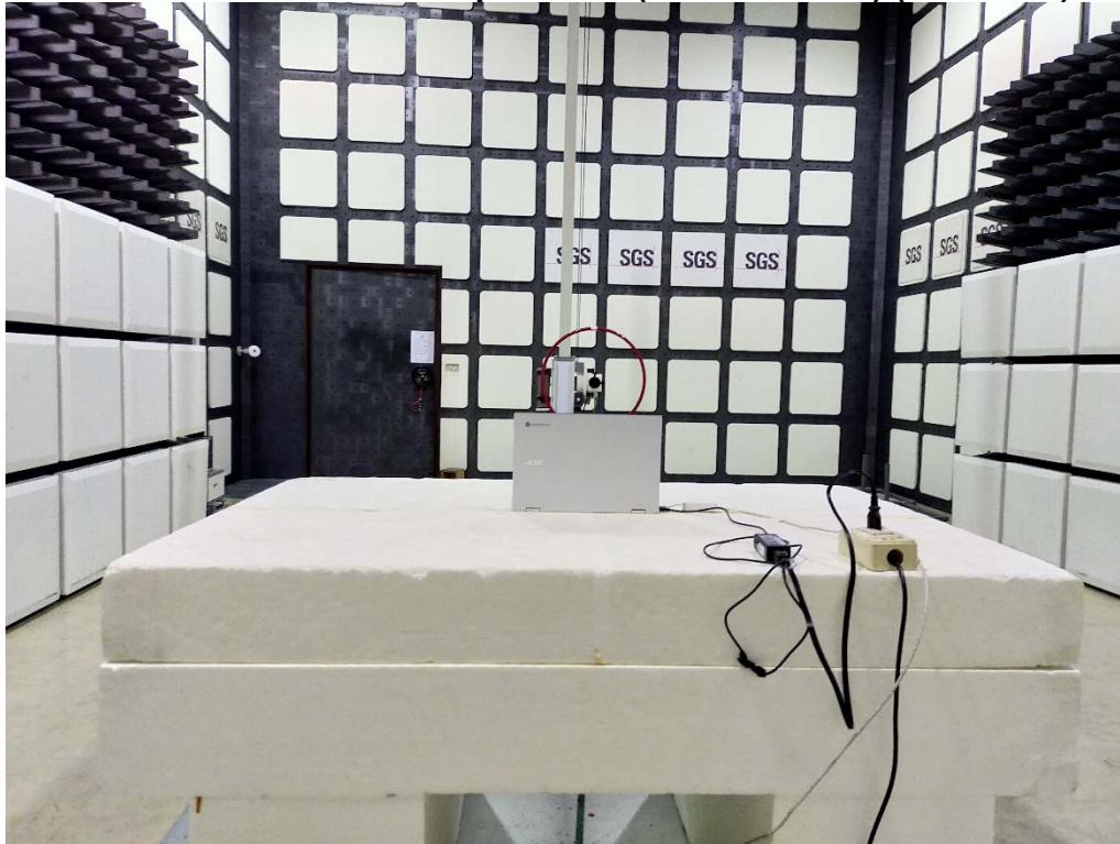
Radiated Emission Set up Photos (Below 1GHz) (NB Plane)
