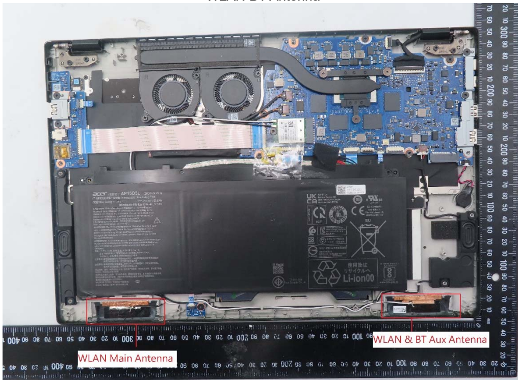
WLAN BT Antenna
