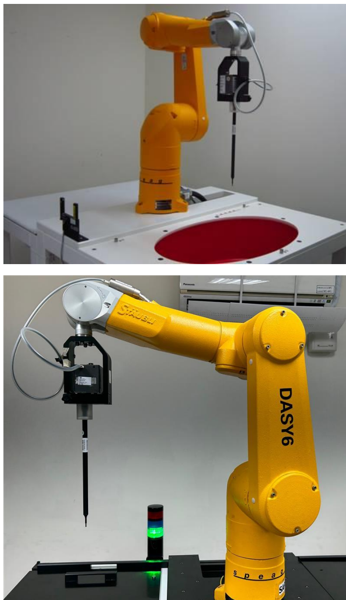
Fig.1 Photograph of the SAR measurement system
