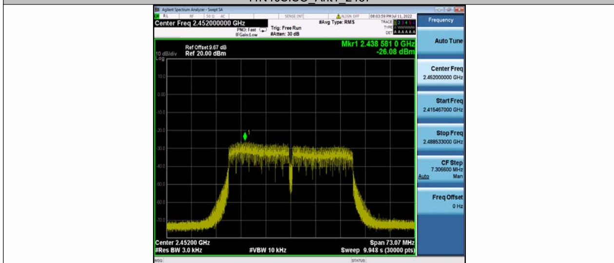
11N40SISO_Ant1_2452
