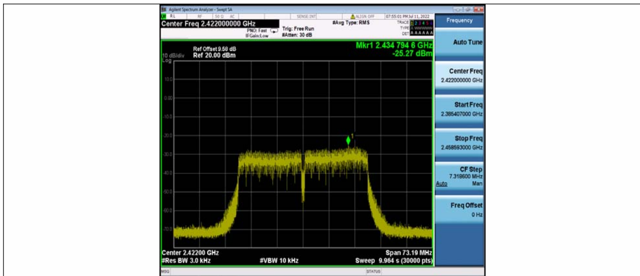
11N40SISO_Ant1_2422
