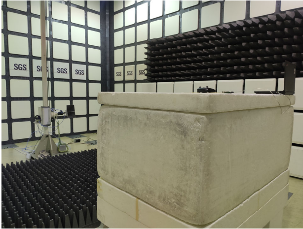
FCC_15_247_BT_Radiated_Setup
