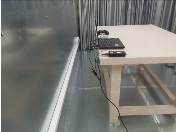
FCC_15_247_BT_Conduction_Setup
