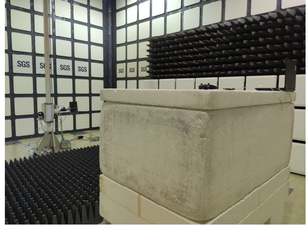
FCC_15_247_2.4G_Radiated_Setup
