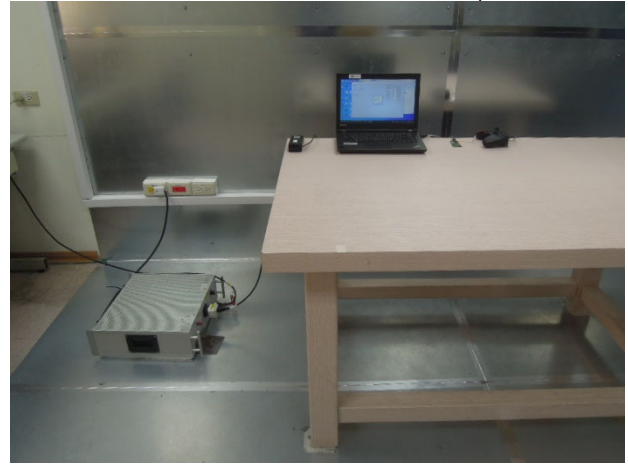
FCC_15_247_2.4G_Conduction_Setup
