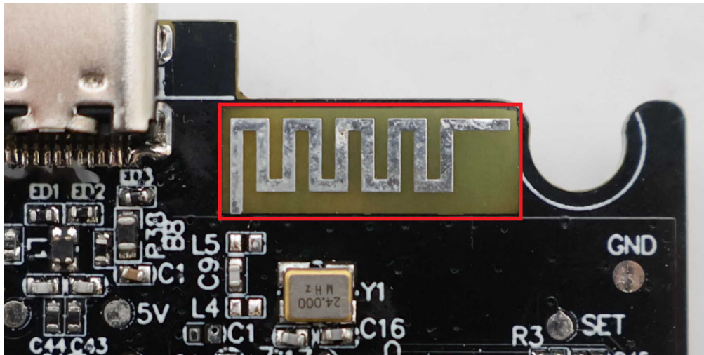
BT&BLE&SRD2.4G Antenna
