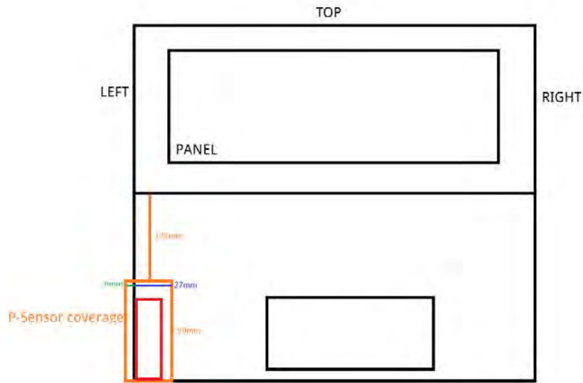
Fig.7 Antenna position of EUT
