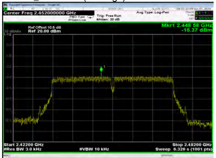
802.11n_HT40 PSD (CH-High)
