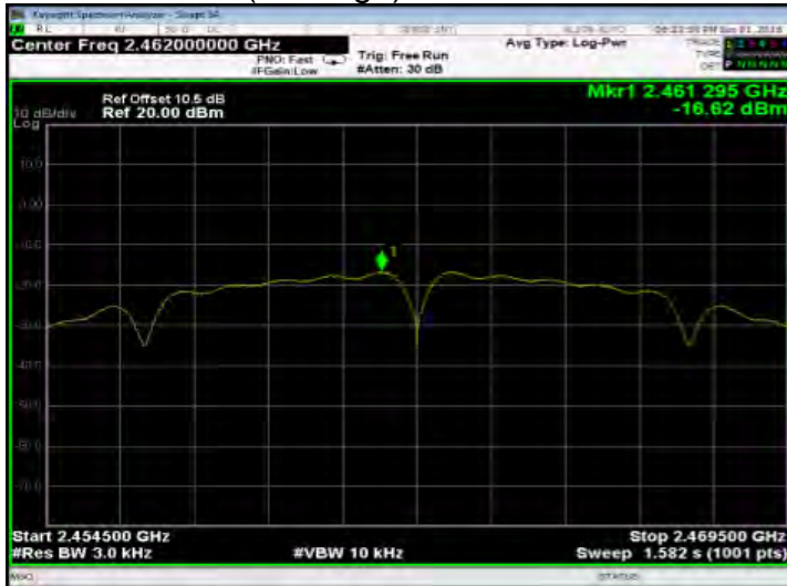
802.11b PSD (CH-High)
