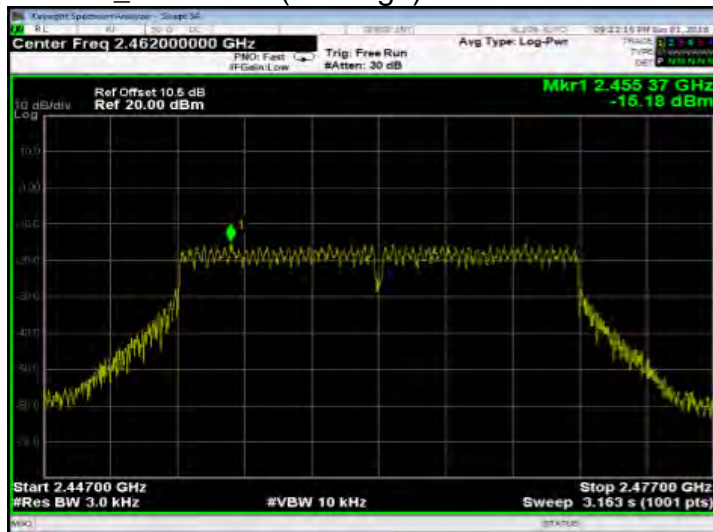
802.11n_HT20 PSD (CH-High)
