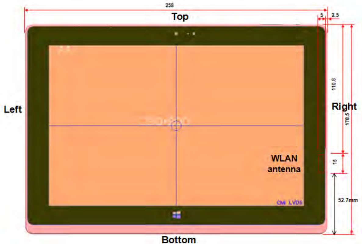
Fig.7 Antenna position (Front view)
