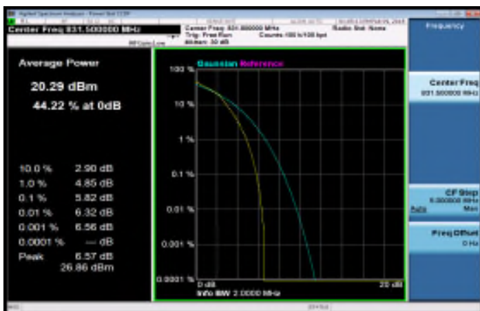
LTE_Band26_1_4MHz_16QAM_6_0_MidCH26865
