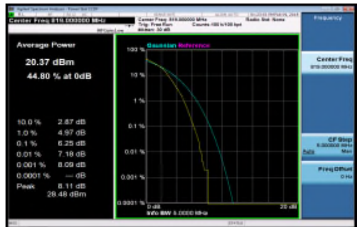
Part 90_LTE_Band26_5MHz_16QAM_25_0_MidCH26740
