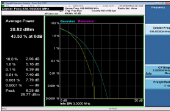
LTE_Band5_3MHz_16QAM_15_0_HighCH20635-847.5
