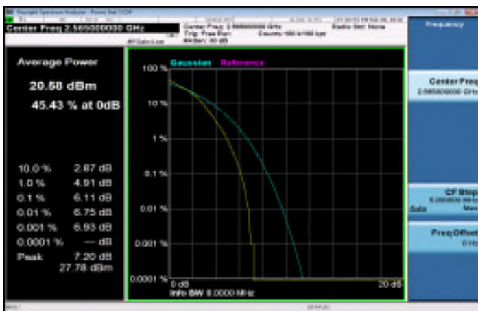
LTE_Band7_10MHz_16QAM_50_0_HighCH21400-2565
