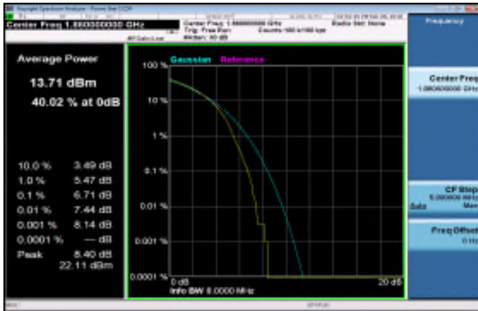
LTE_Band2_20MHz_16QAM_100_0_MidCH18900-1880
