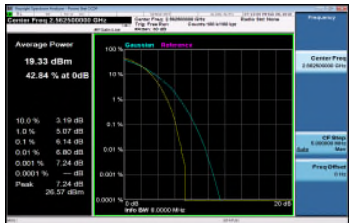
LTE_Band7_15MHz_16QAM_75_0_HighCH21375-2562.5
