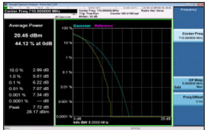
LTE_Band17_10MHz_16QAM_50_0_MidCH23790-710
