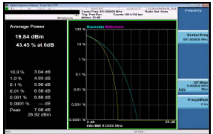
LTE_Band26_10MHz_16QAM_50_0_MidCH26865
