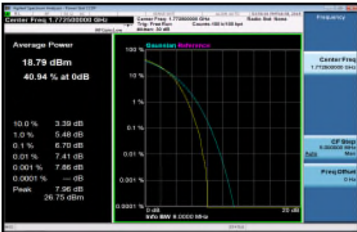
LTE_Band66_15MHz_16QAM_75_0_HighCH132597
