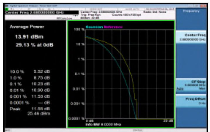
LTE_Band41_20MHz_16QAM_100_0_HighCH41490
