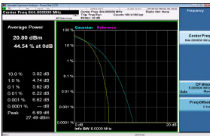
LTE_Band5_10MHz_16QAM_50_0_HighCH20600-844
