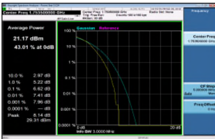
LTE_Band4_3MHz_16QAM_15_0_HighCH20385-1753.5
