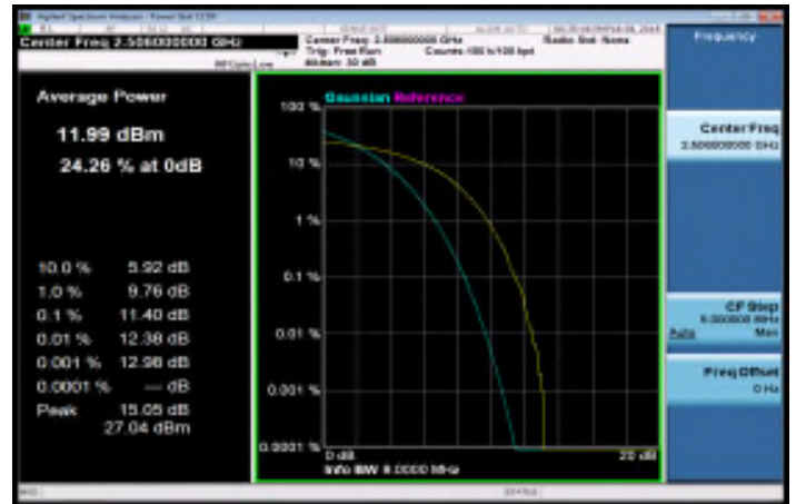
LTE_Band41_20MHz_16QAM_100_0_MidCH40620
