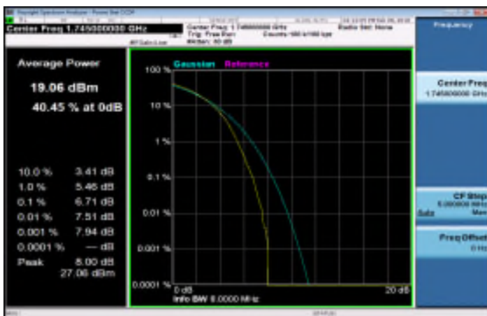
LTE_Band4_20MHz_16QAM_100_0_HighCH20300-1745
