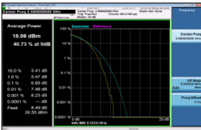
LTE_Band7_20MHz_16QAM_100_0_HighCH21350-2560
