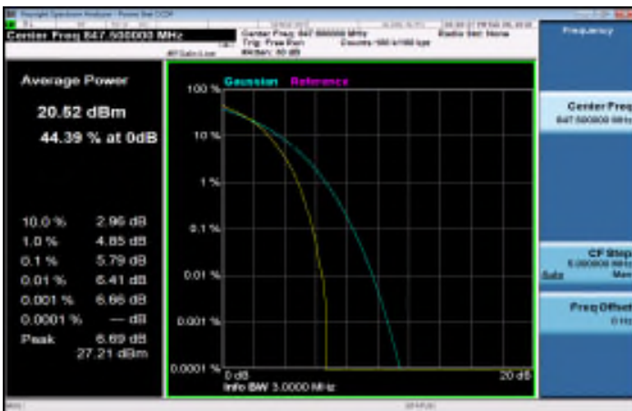
LTE_Band5_3MHz_16QAM_15_0_HighCH20635-847.5
