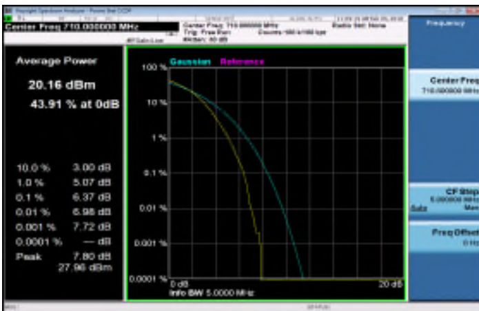
LTE_Band17_5MHz_16QAM_25_0_MidCH23790-710
