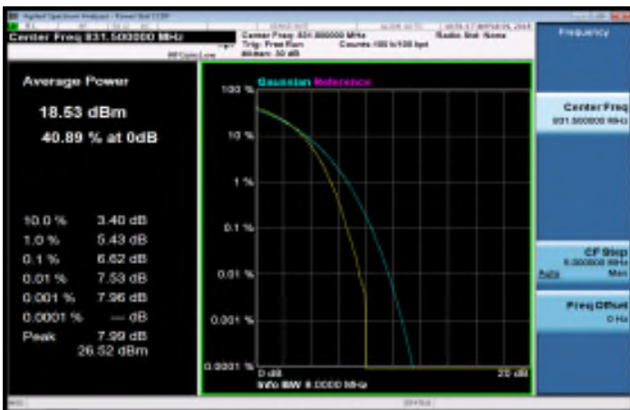
LTE_Band26_15MHz_16QAM_75_0_MidCH26865
