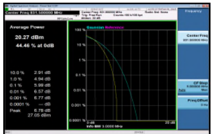
LTE_Band26_3MHz_16QAM_15_0_MidCH26865
