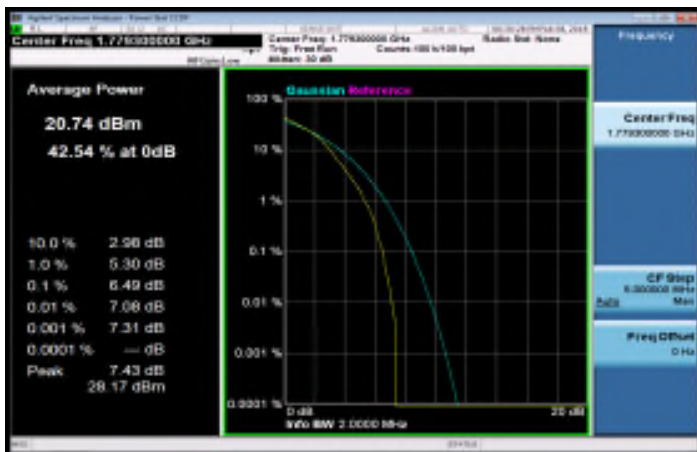
LTE_Band66_1_4MHz_16QAM_6_0_HighCH132665
