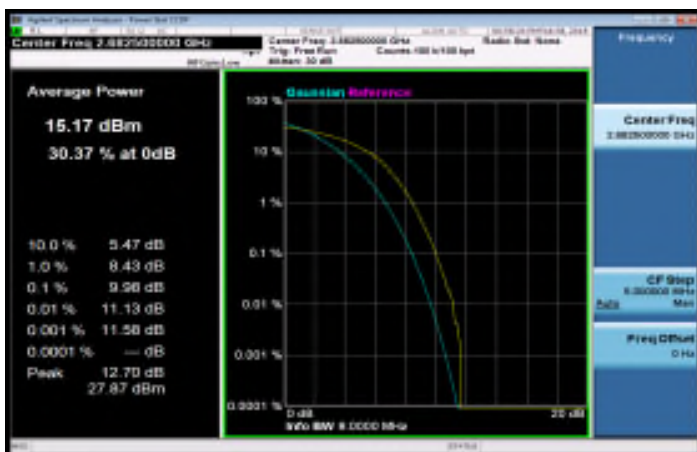
LTE_Band41_15MHz_16QAM_75_0_HighCH41515
