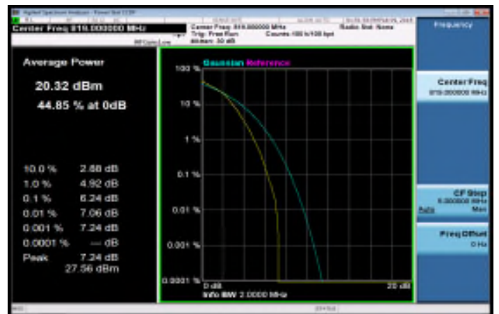
Part 90_LTE_Band26_1_4MHz_16QAM_6_0_MidCH26740
