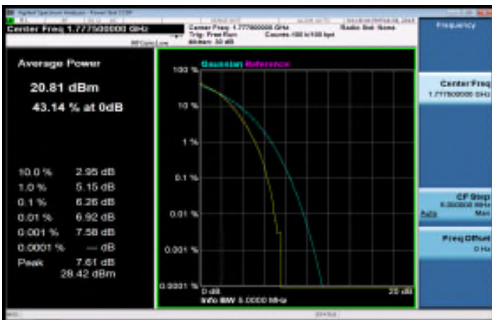
LTE_Band66_5MHz_16QAM_25_0_HighCH132647
