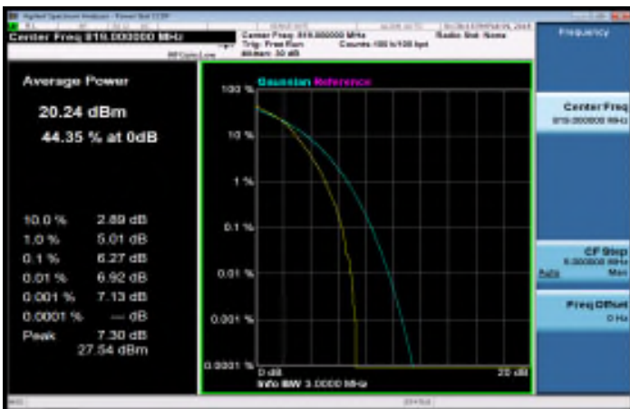
Part 90_LTE_Band26_3MHz_16QAM_15_0_MidCH26740
