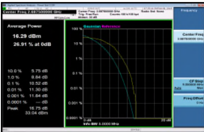
LTE_Band41_5MHz_16QAM_25_0_HighCH41565
