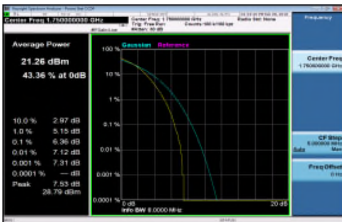
LTE_Band4_10MHz_16QAM_50_0_HighCH20350-1750
