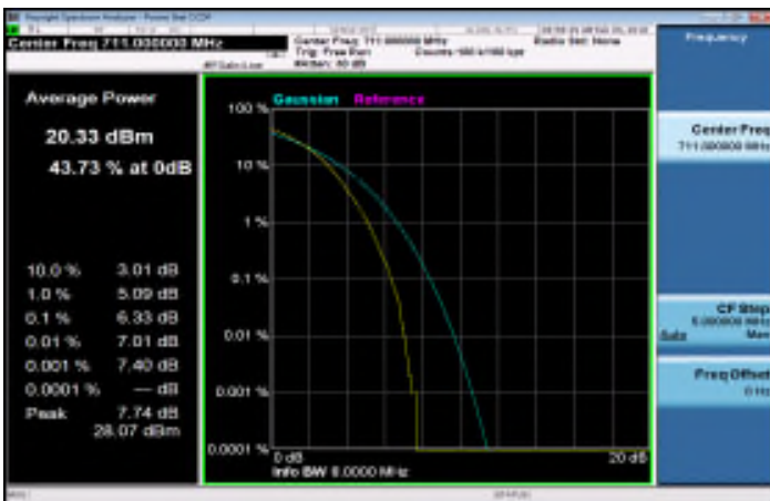
LTE_Band12_10MHz_16QAM_50_0_HighCH23130-711
