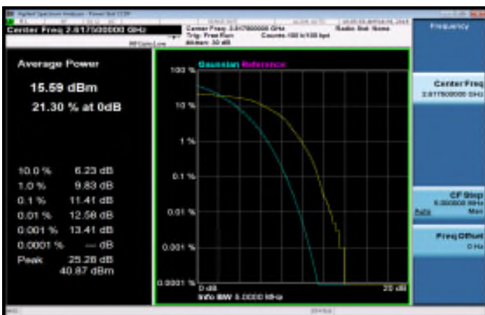
LTE_Band38_5MHz_16QAM_25_0_HighCH38225-2617.5
