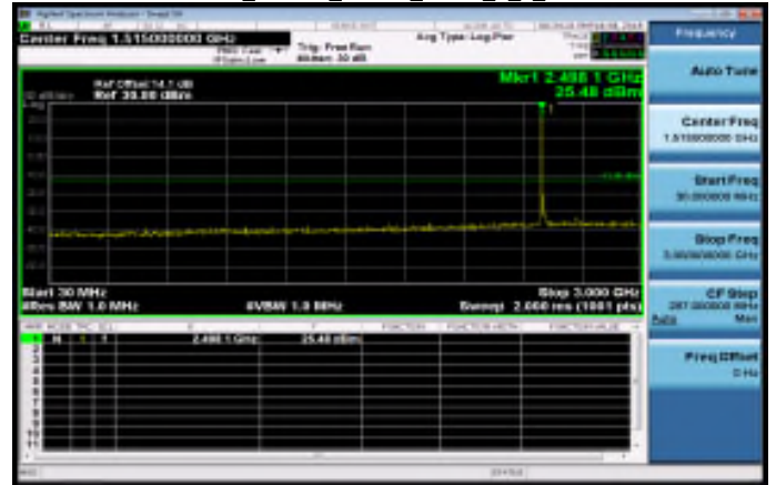
30MHz~3GHz_Band41_20MHz_QPSK_1_0_LowCH39750
