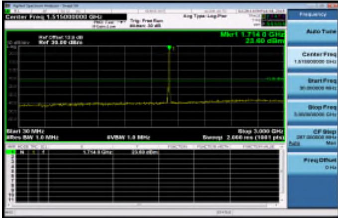
30MHz~3GHz_HSUPA_B4_LowCH1312-1712.4
