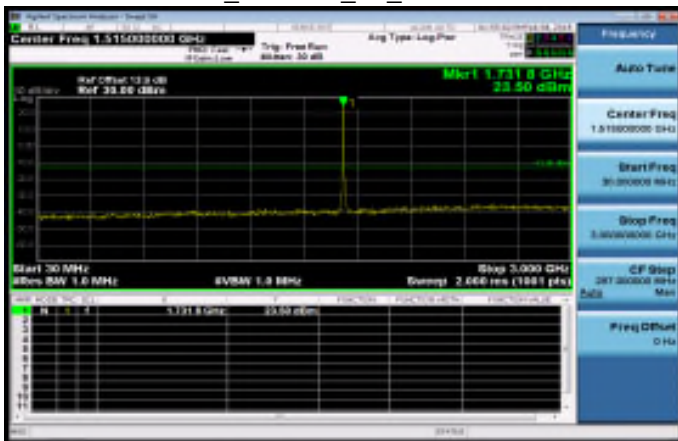
30MHz~3GHz_WCDMA_B4_MidCH1413-1732.6
