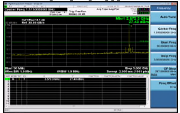
30MHz~3GHz_Band38_20MHz_QPSK_1_0_LowCH37850-2580
