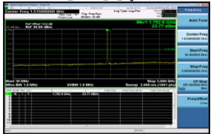
30MHz~3GHz_WCDMA_B4_HighCH1513-1752.6
