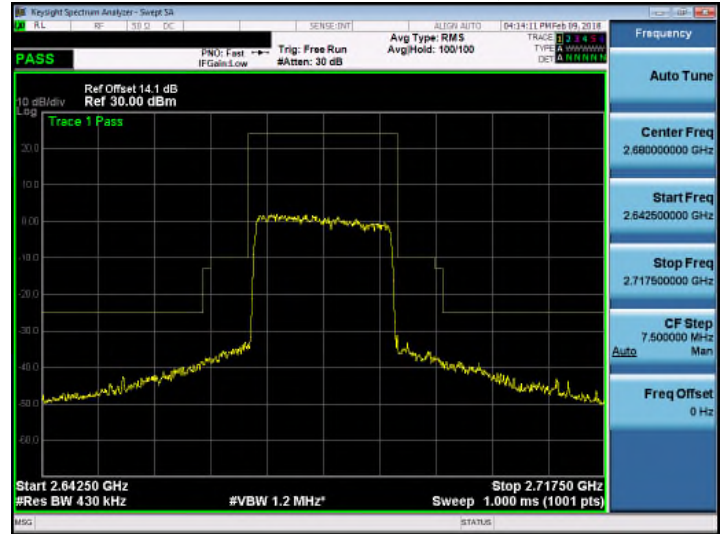
Band 41_16QAM_20M_RB100,0
