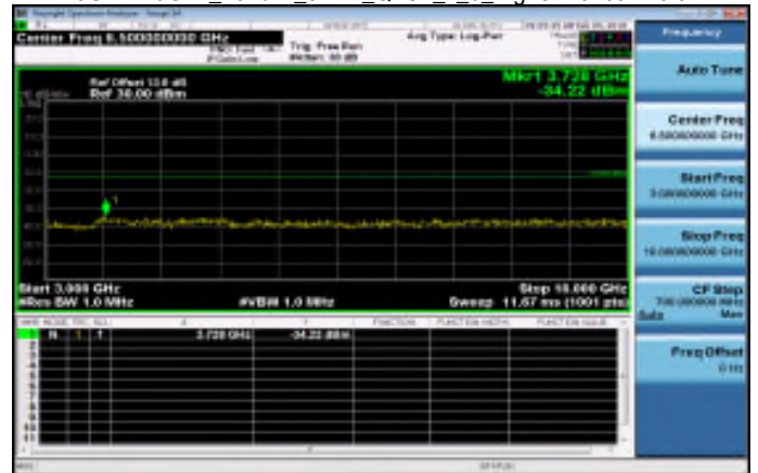
3GHz~10GHz_Band12_5MHz_QPSK_1_0_HighCH23155-713.5
