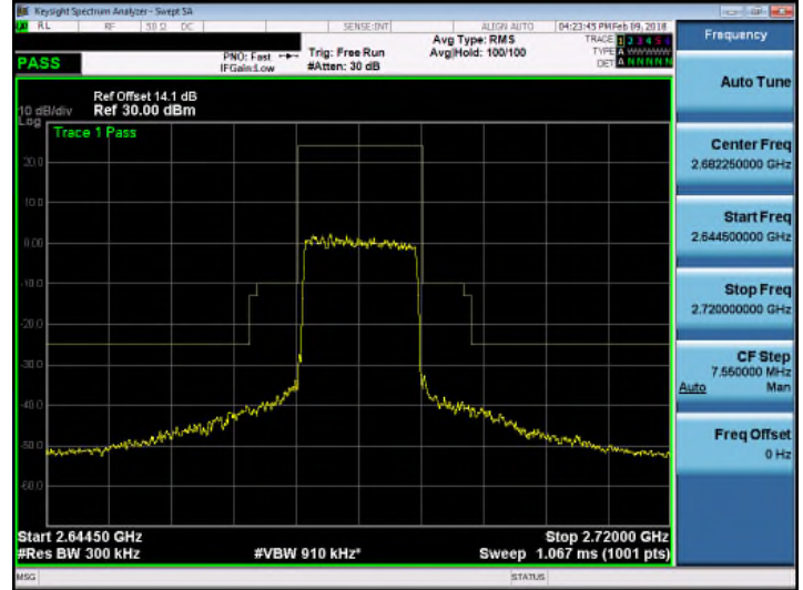
Band 41_QPSK_20M_RB1,0
