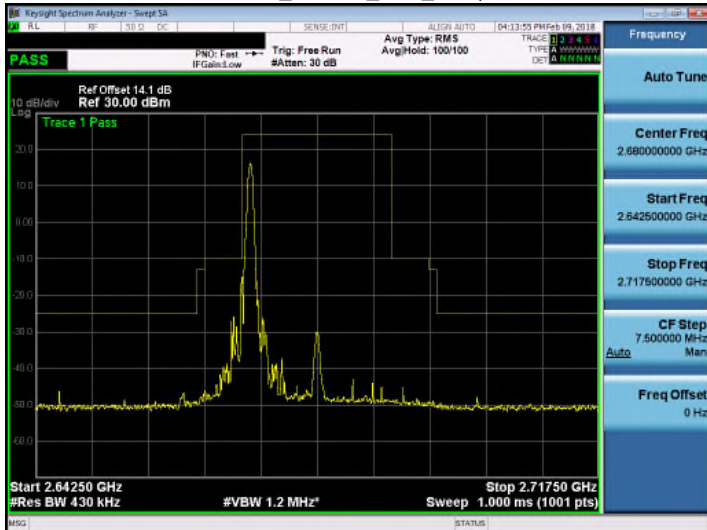
Band 41_16QAM_20M_RB1,99
