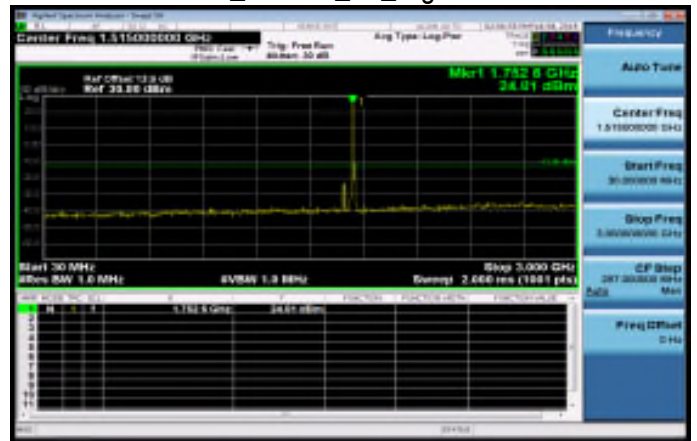
30MHz~3GHz_HSDPA_B4_HighCH1513-1752.6
