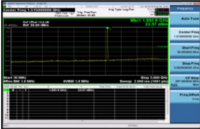
30MHz~3GHz_WCDMA_B2_LowCH9262-1852.4
