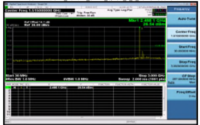
30MHz~3GHz_Band41_5MHz_QPSK_1_0_LowCH39675
