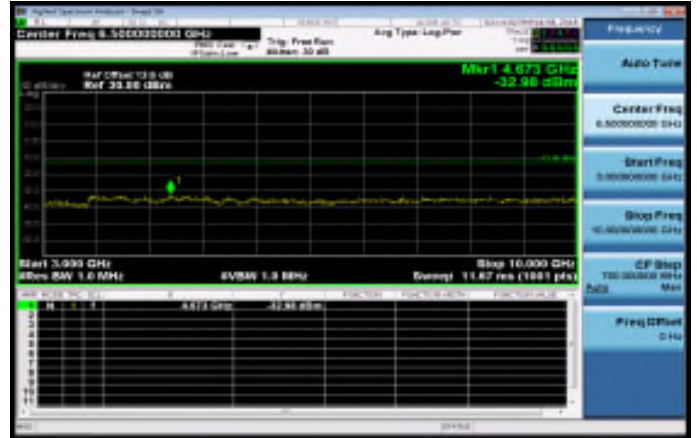
3GHz~10GHz_HSDPA_B5_MidCH4183-836.6
