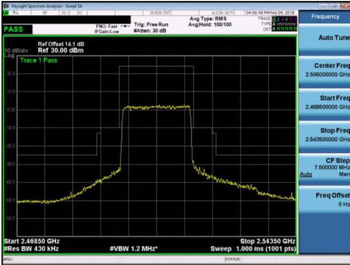
Band 41_QPSK_20M_RB1,0
