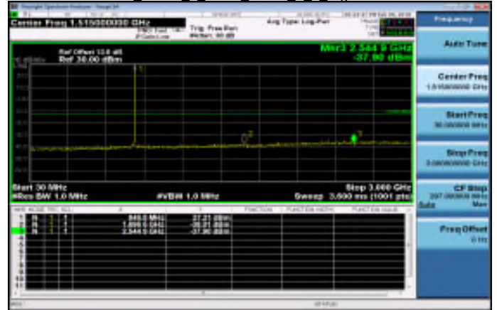
30MHz~3GHz_Band5_1_4MHz_QPSK_1_0_HighCH20643-848.3
