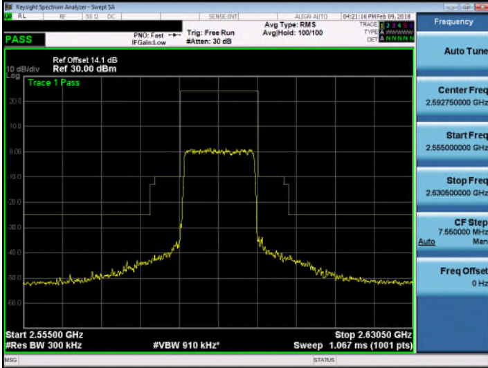
Band 41_16QAM_15M_RB1,0
