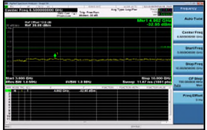
3GHz~10GHz_HSUPA_B5_MidCH4183-836.6
