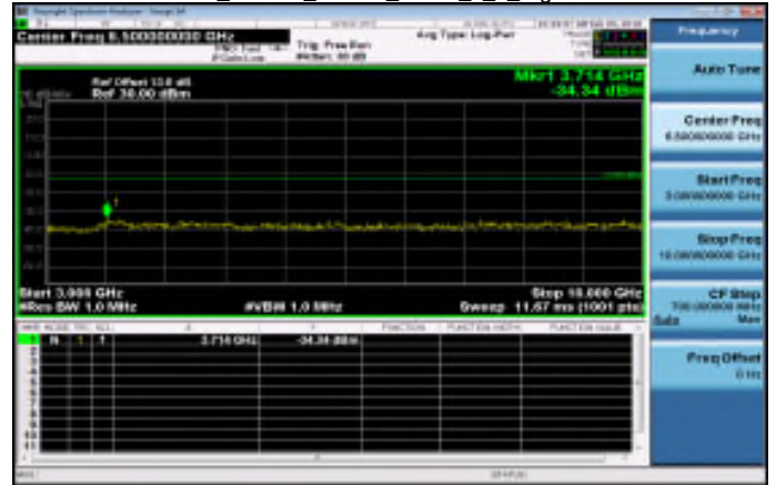
3GHz~10GHz_Band17_10MHz_QPSK_1_0_HighCH23800-711
