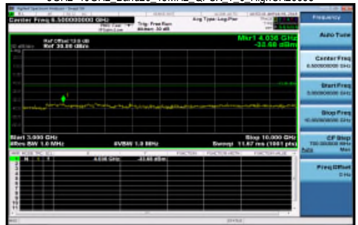
3GHz~10GHz_Band26_15MHz_QPSK_1_0_HighCH26965
