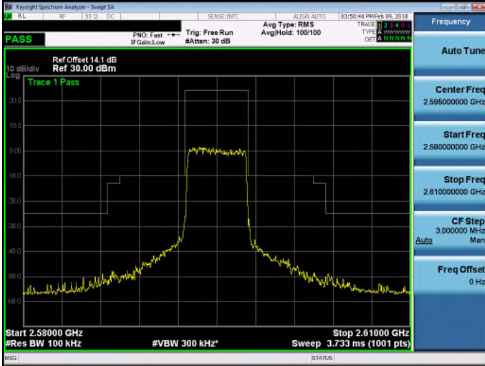
Band 38_16QAM_5M_RB1,0
