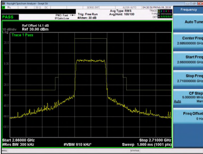
Band 41_16QAM_10M_RB1,0
