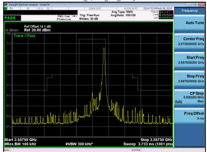
Band 38_QPSK_5M_RB1,24
