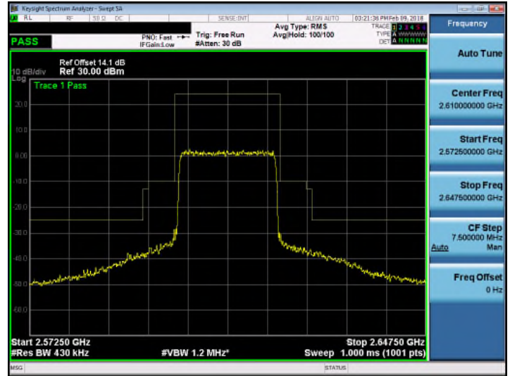
Band 41_QPSK_5M_RB1,0
