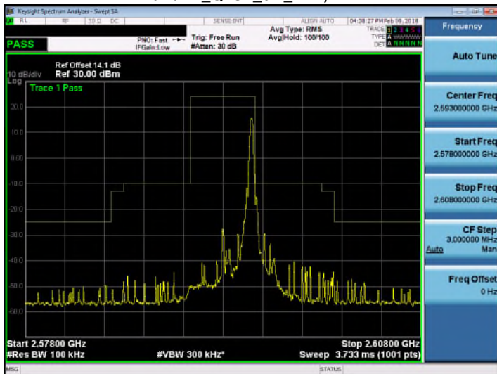
Band 41_QPSK_5M_RB1,24
