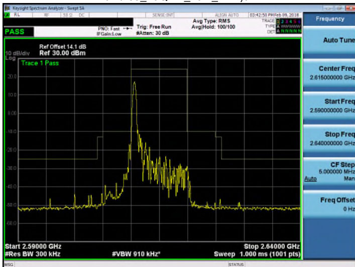
Band 38_16QAM_10M_RB1,49
