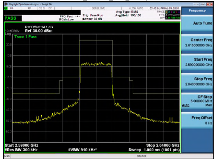
Band 38_QPSK_15M_RB1,0
