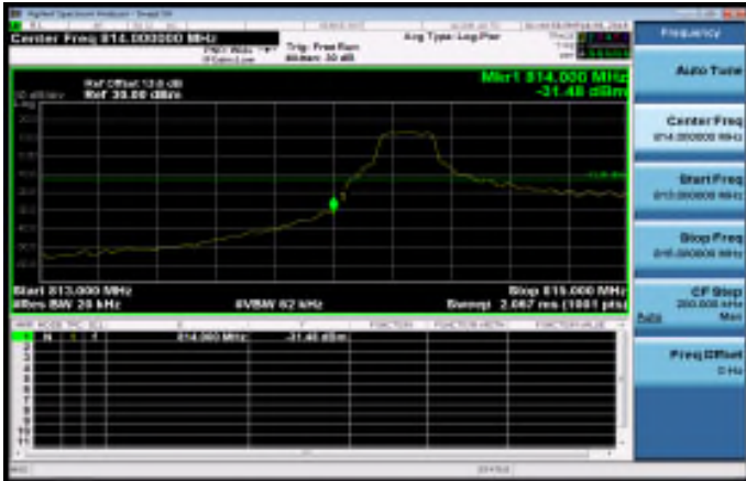
Part 90_Band26_1_4MHz_QPSK_1_0_LowCH26697
