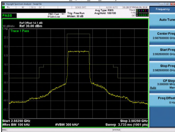
Band 7_QPSK_5M_RB25,0
