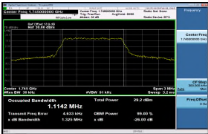
Band66_1_4MHz_16QAM_6_0_MidCH132322
