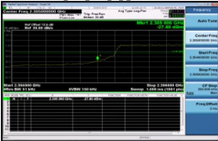
Band30_5MHz_QPSK_25_0_LowCH27685
