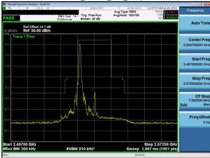
Band 7_16QAM_15M_RB1,74
