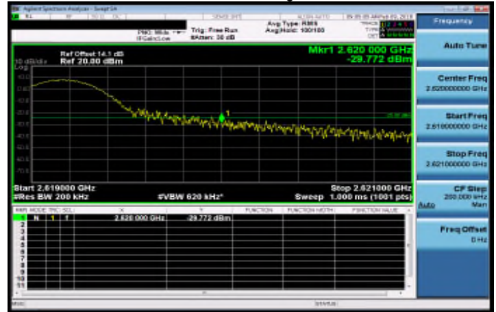
Band38_15MHz_QPSK_1_74_HighCH38175-2612.5
