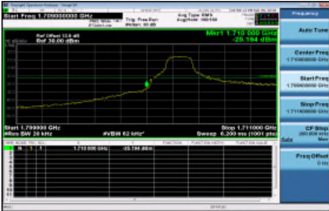
Band4_1_4MHz_QPSK_1_0_LowCH19957-1710.7
