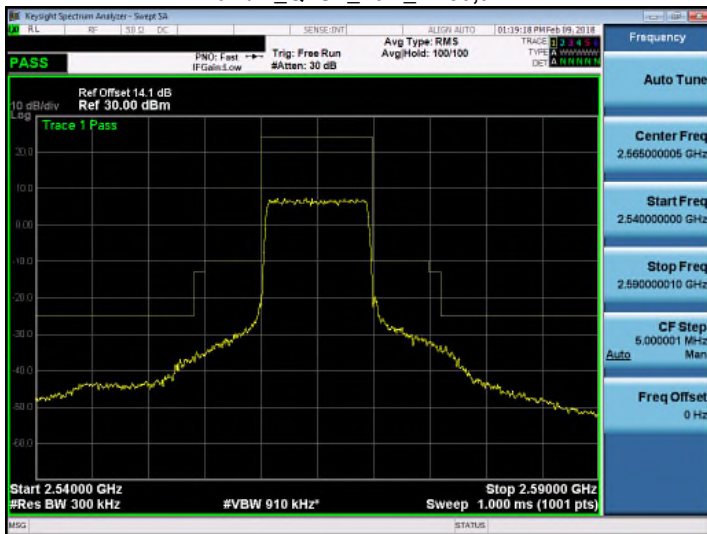
Band 7_QPSK_10M_RB50,0
