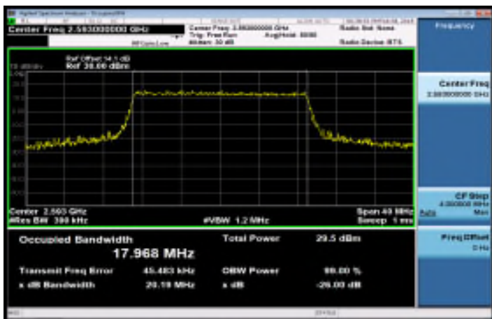
Band41_20MHz_16QAM_100_0_MidCH40620
