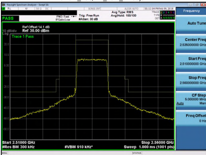
Band 7_16QAM_10M_RB50,0
