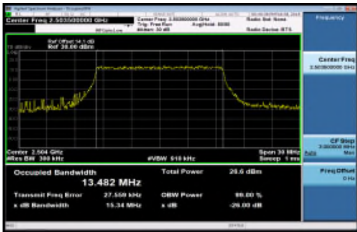
Band41_15MHz_16QAM_75_0_MidCH40620
