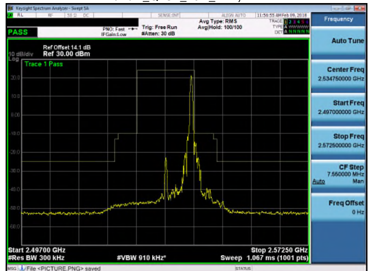
Band 7_QPSK_15M_RB75,0
