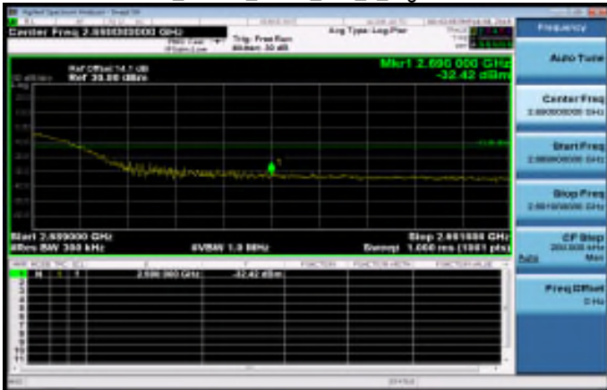
Band41_20MHz_QPSK_100_0_HighCH41490
