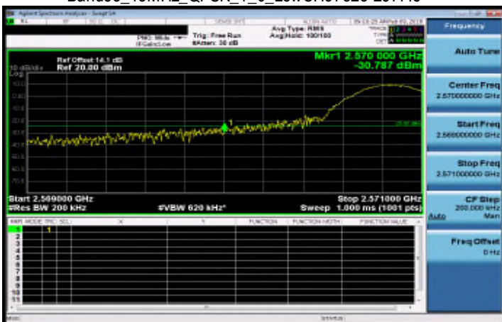
Band38_15MHz_QPSK_1_0_LowCH37825-2577.5
