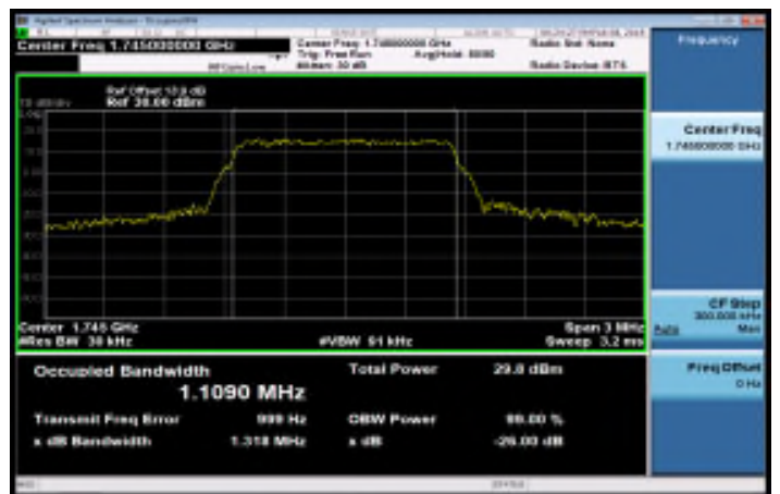
Band66_1_4MHz_QPSK_6_0_MidCH132322
