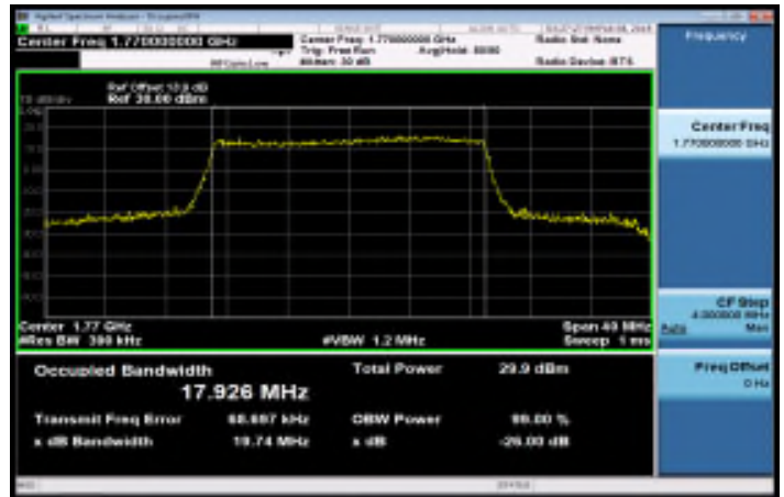
Band66_20MHz_16QAM_100_0_HighCH132572
