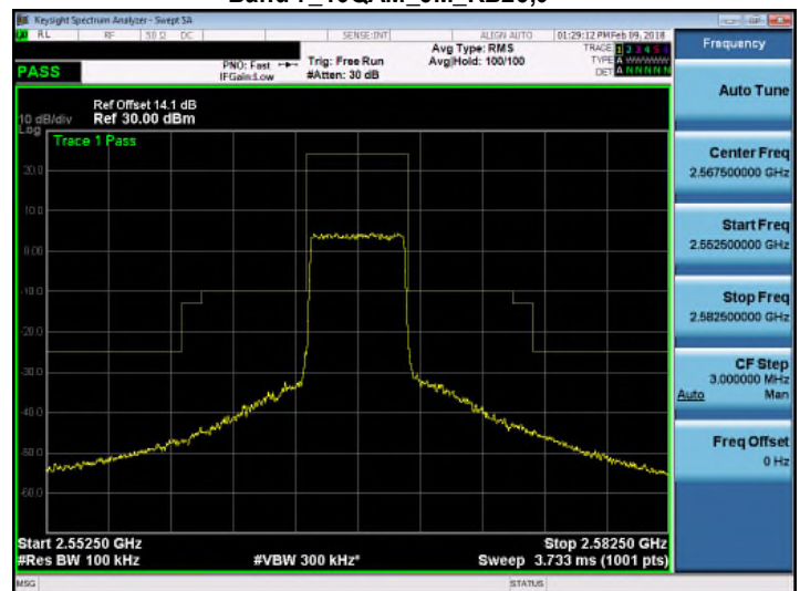
Band 7_16QAM_5M_RB25,0
