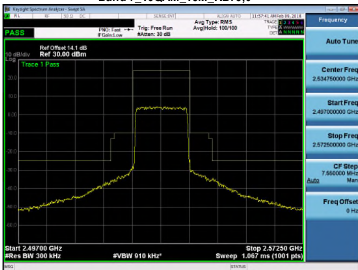
Band 7_16QAM_15M_RB75,0
