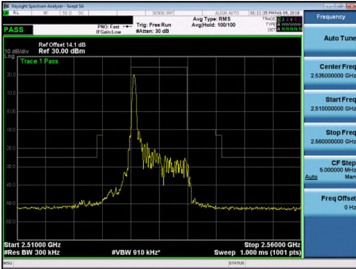
Band 7_16QAM_10M_RB1,49
