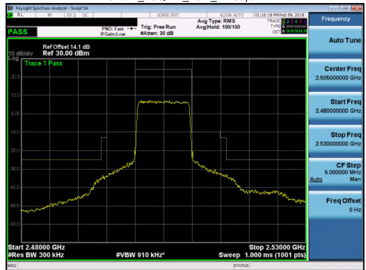
Band 7_16QAM_10M_RB50,0
