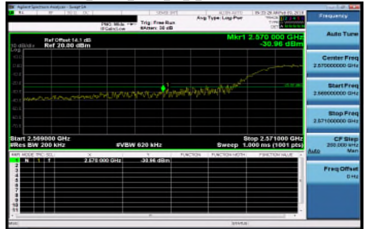
Band38_15MHz_QPSK_75_0_LowCH37825-2577.5
