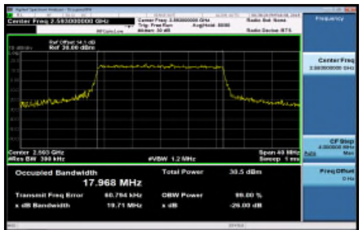
Band41_20MHz_QPSK_100_0_MidCH40620
