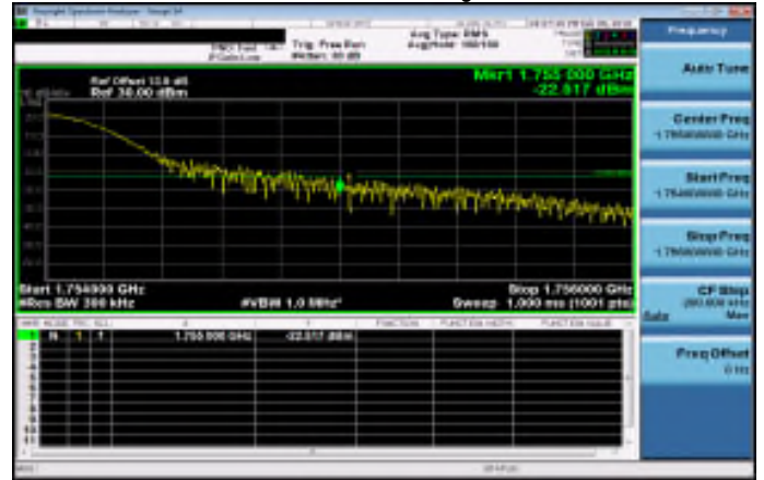
Band4_20MHz_QPSK_1_99_HighCH20300-1745
