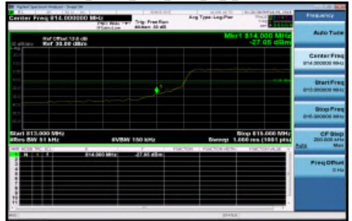
Part 90_Band26_5MHz_QPSK_25_0_LowCH26715
