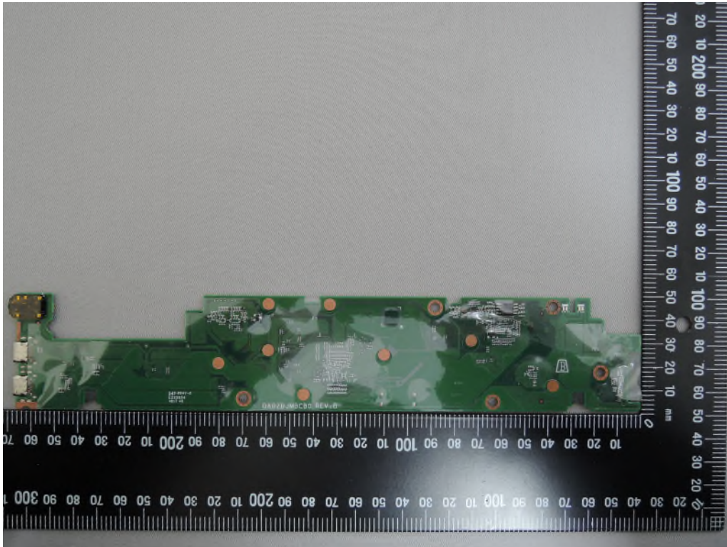
WWAN Module - 1 (Model No.: L850-GL)
