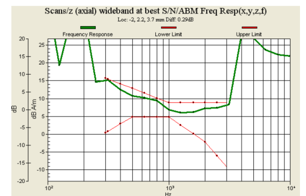
Fig. 9.4 GSM850 Ch189 (Battery 2)
