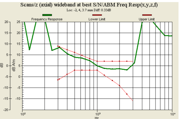
Fig. 9.10 WCDMA Band V Ch4132 (Battery 1)
