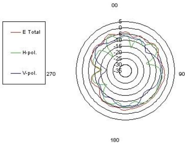
WLAN antenna @2.50GHz
