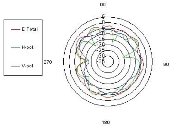
WLAN antenna @2.45GHz
