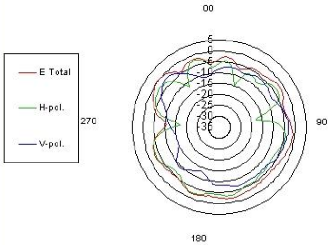
WLAN antenna @2.40GHz
