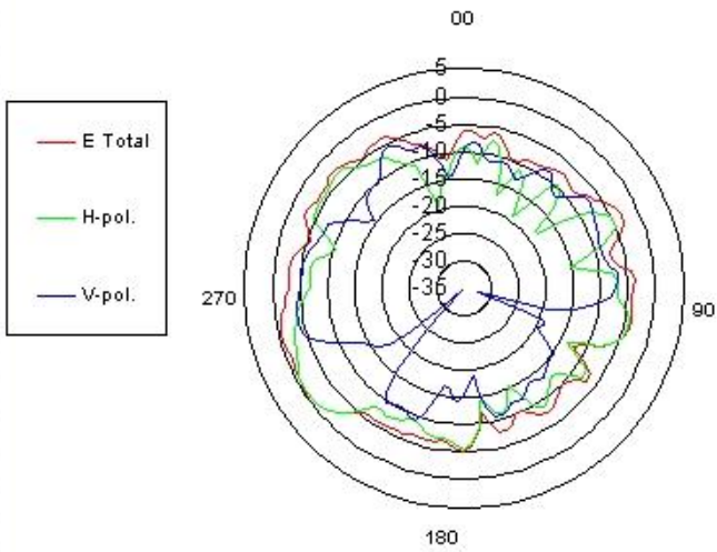
WLAN antenna @5470 MHz
