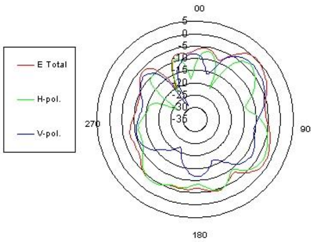
WLAN antenna @2500 MHz
