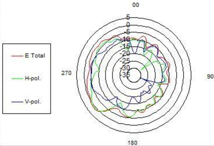
WLAN antenna @5250 MHz
