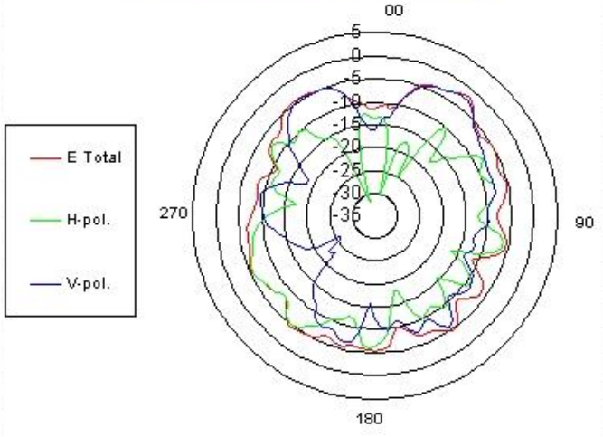
WLAN antenna @5785 MHz
