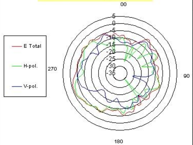
WLAN antenna @5600 MHz
