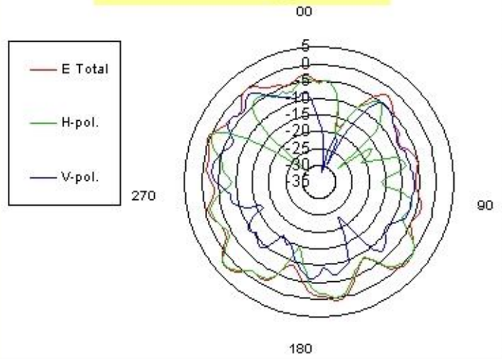
WLAN antenna @5.15 GHz
