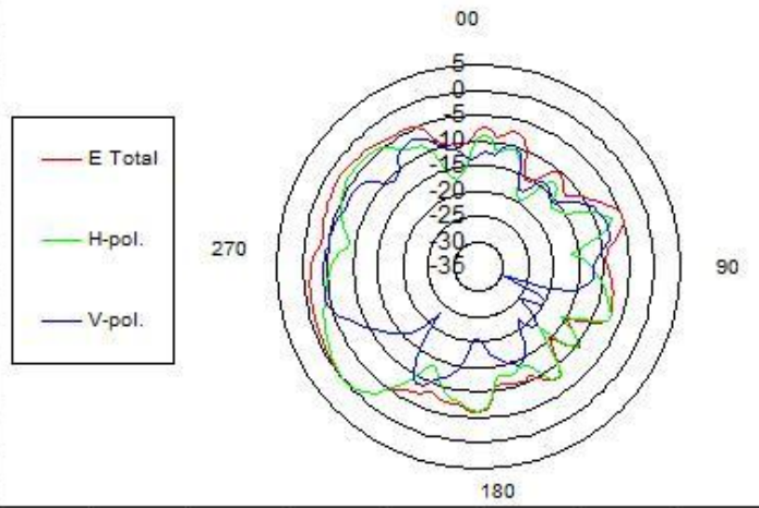
WLAN antenna @5350 MHz
