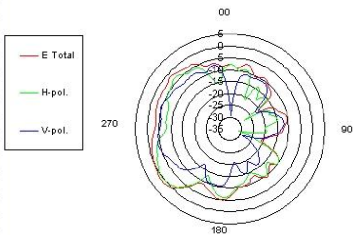
WLAN antenna @5150 MHz
