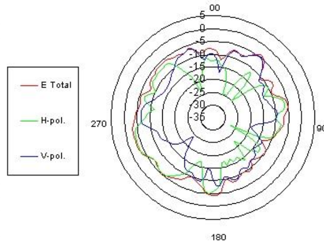
WLAN antenna @5725 MHz
