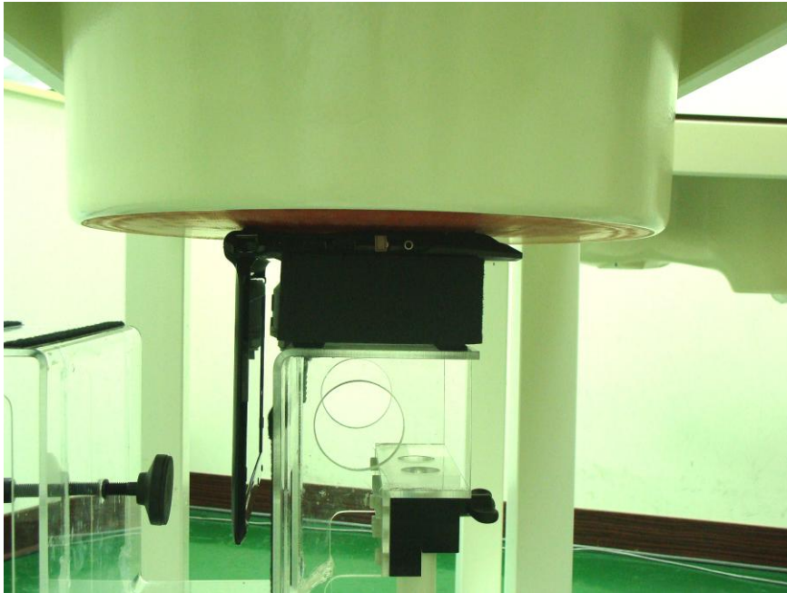
Bottom of the host notebook computer with Phantom 0 cm Gap
