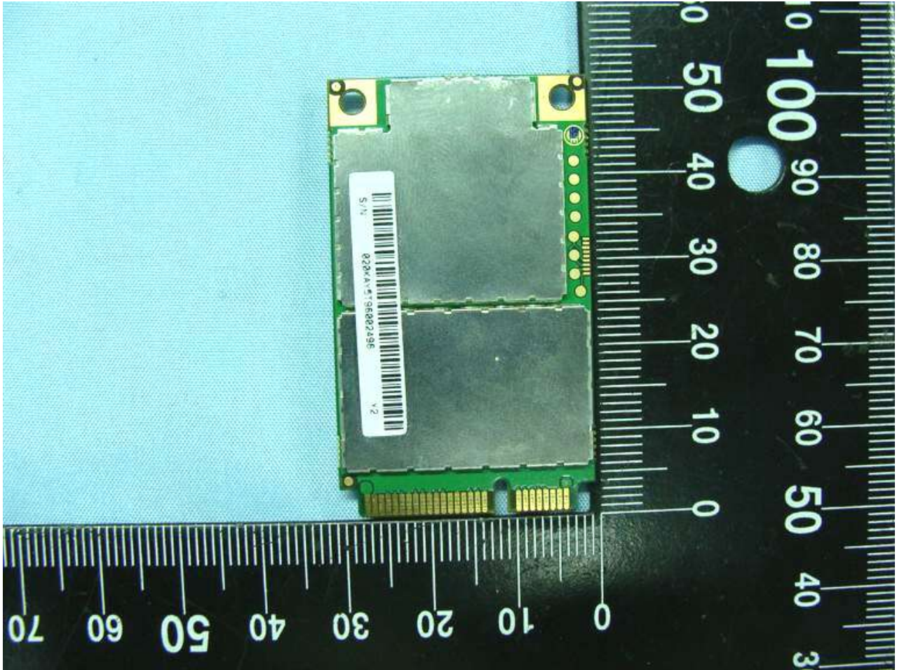
EUT: WWAN module (Acer, Gateway, PackardBell / EM770W)
