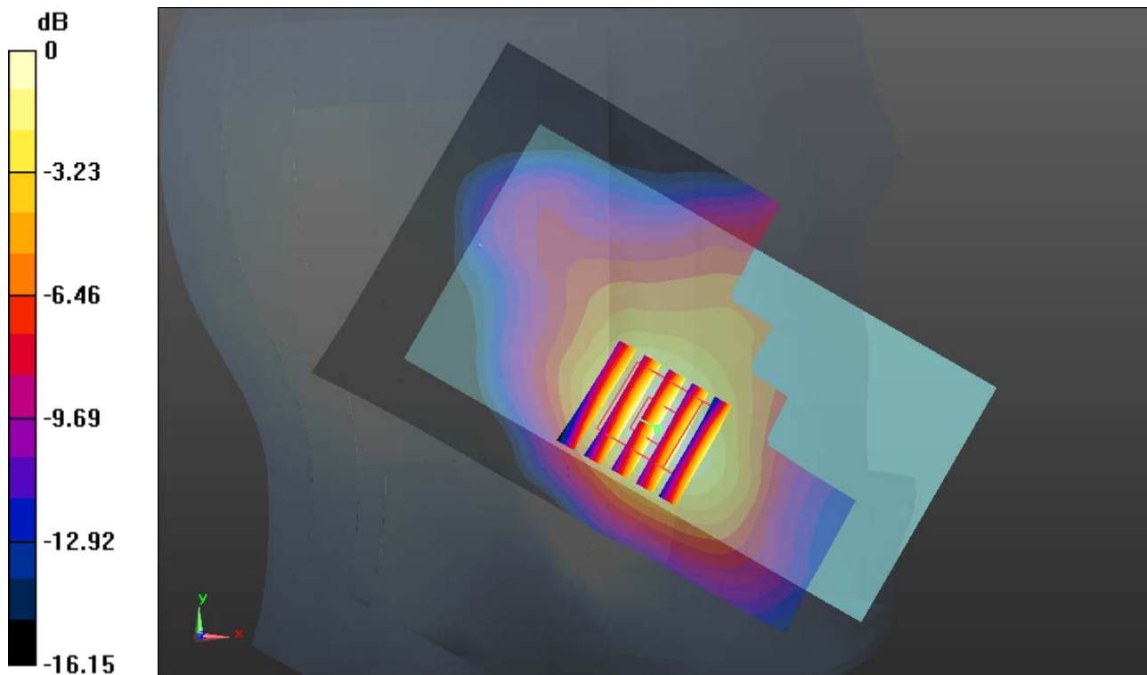
0 dB = 0.520mW/g
