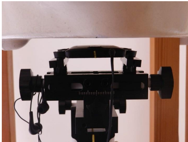
Back with headset, Test Separation 1.0 cm
