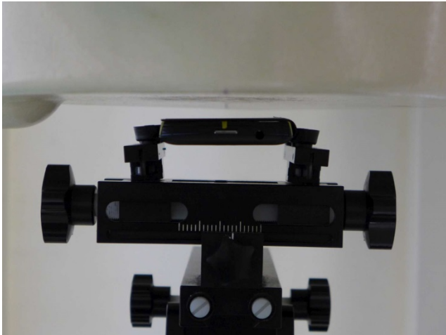
Front, Test Separation 1 cm with Holster Closed
