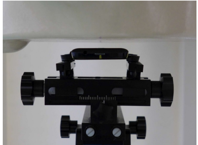
Back, Test Separation 1 cm with Holster Closed
