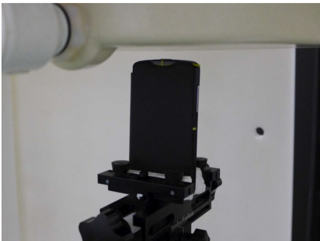
Top Side, Test Separation 1 cm with Holster Closed
