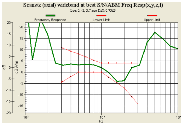
Fig. 9.15 WCDMA Band V Ch4182 for Sample B
