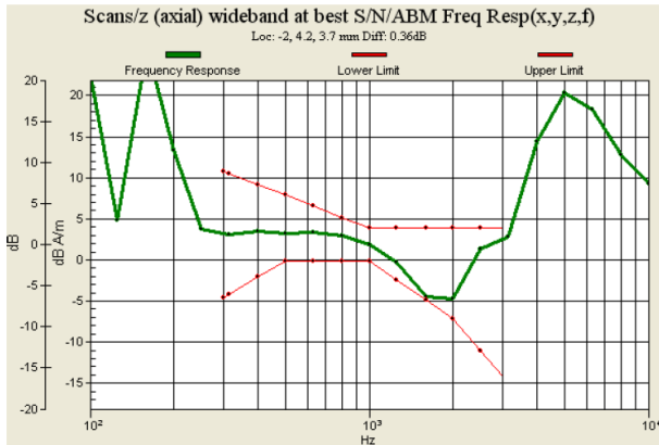
Fig. 9.7 WCDMA Band V Ch4132 for Sample A
