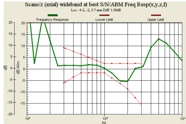
Fig. 9.10 WCDMA Band II Ch9262 for Sample A
