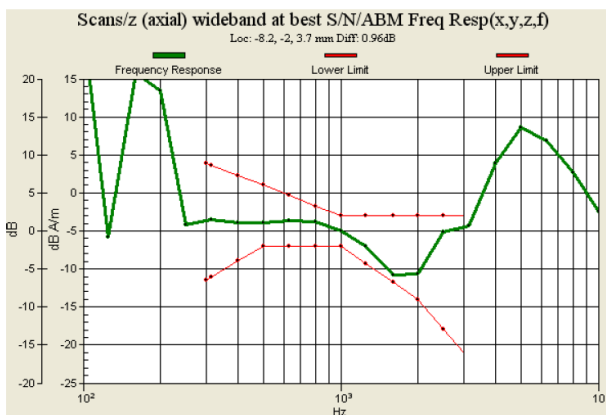
Fig. 9.11 WCDMA Band II Ch9400 for Sample A
