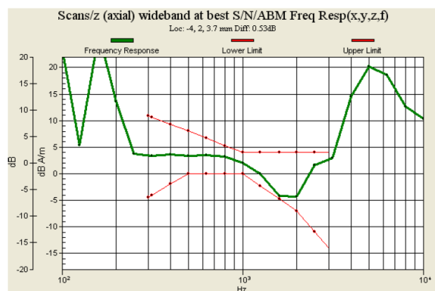
Fig. 9.12 WCDMA Band II Ch9538 for Sample A
