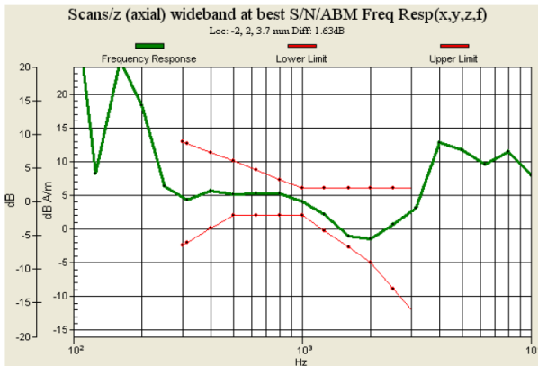
Fig. 9.13 GSM850 Ch189 for Sample B
