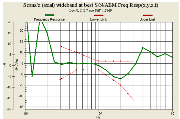
Fig. 9.4 GSM1900 Ch512 for Sample A
