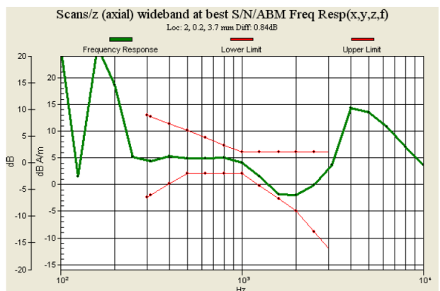
Fig. 9.6 GSM1900 Ch810 for Sample A
