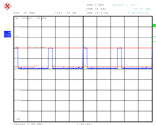
1880MHz - 80% AM
