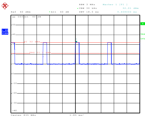
835MHz - 80% AM
