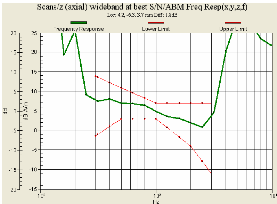
Figure 8.16: Frequency Response of GSM1900 for Ch512
