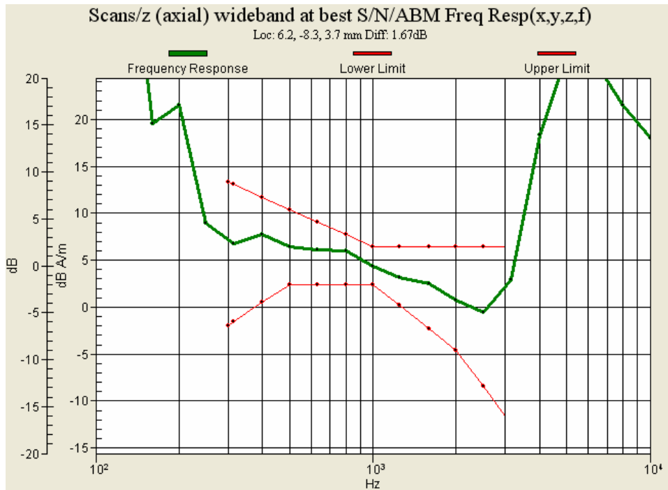
Figure 8.17: Frequency Response of GSM1900 for Ch661
