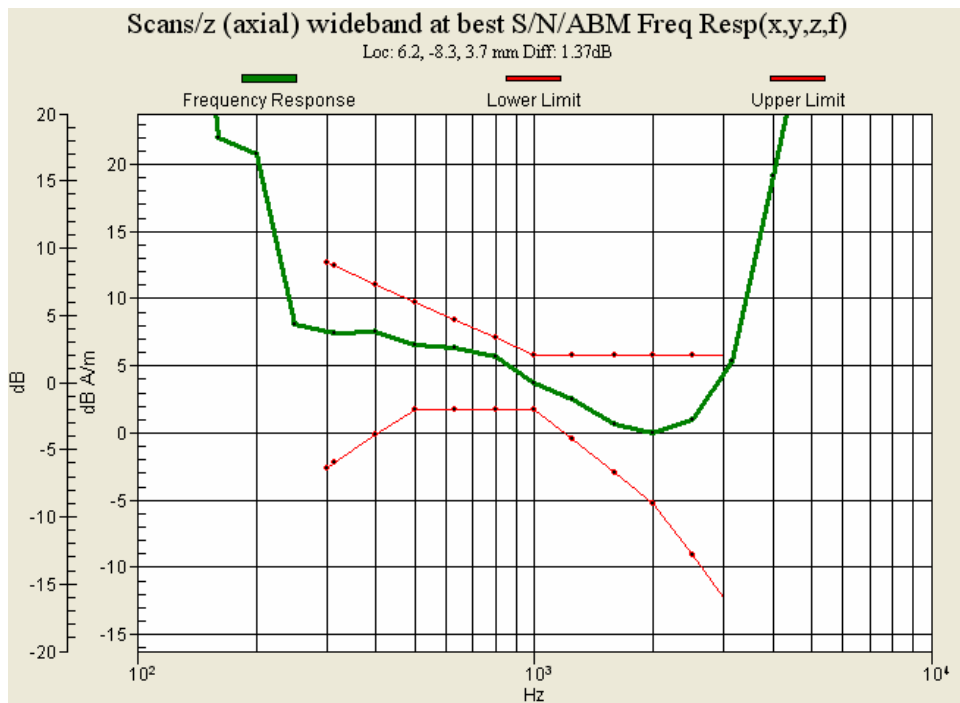
Figure 8.22: Frequency Response of WCDMA Band II for Ch9262
