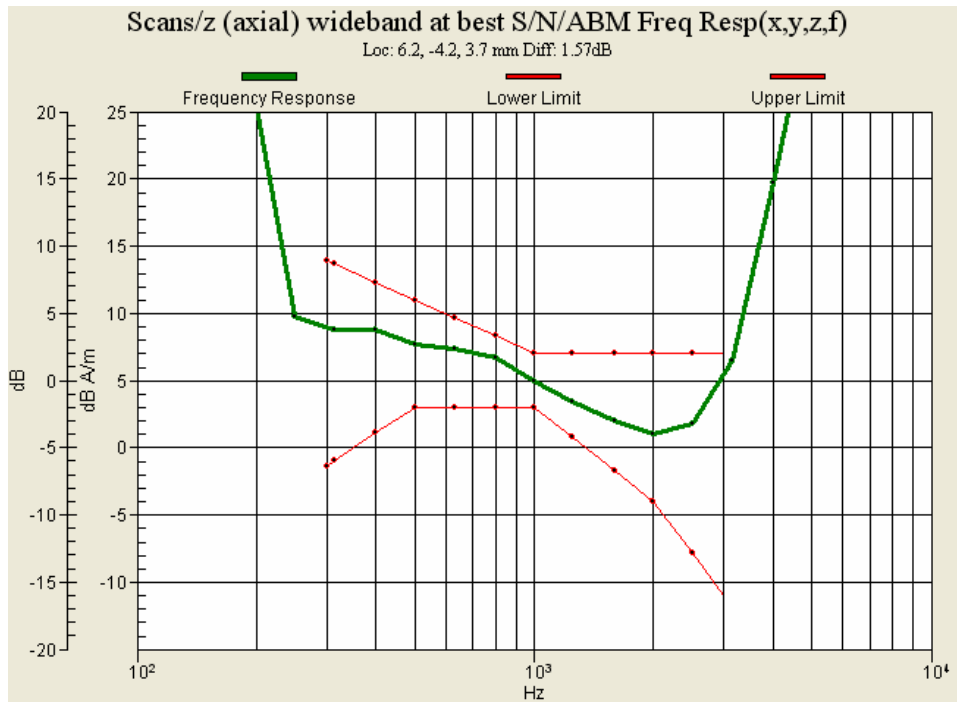
Figure 8.19: Frequency Response of WCDMA Band V for Ch4132
