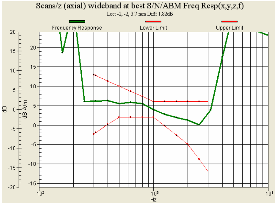
Figure 8.13: Frequency Response of GSM850 for Ch128
