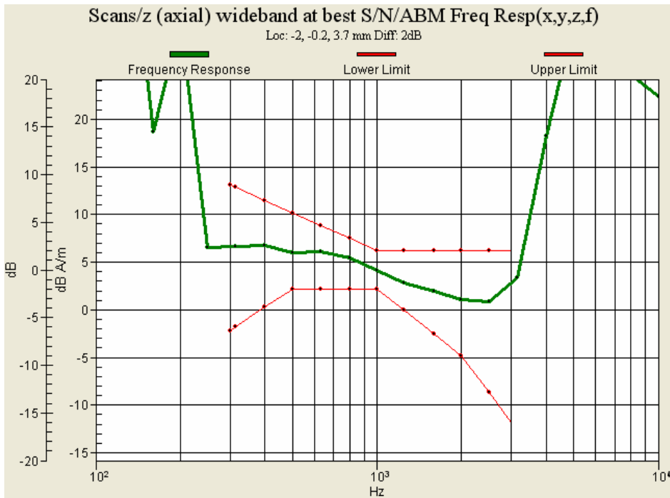
Figure 8.14: Frequency Response of GSM850 for Ch189
