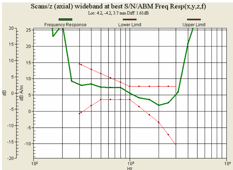
Figure 8.18: Frequency Response of GSM1900 for Ch810
