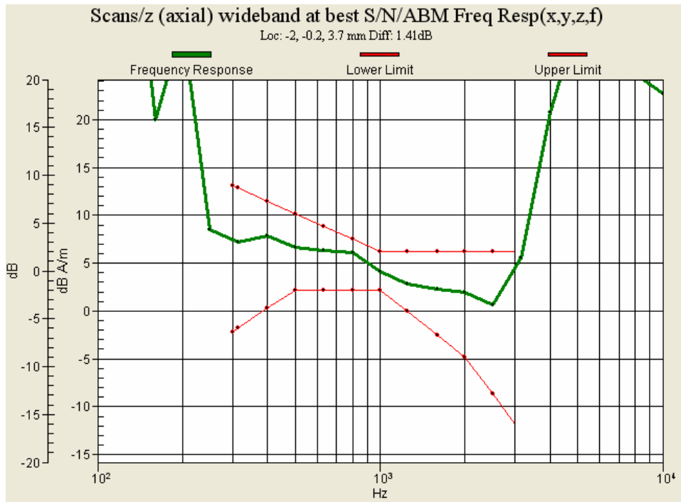
Figure 8.15: Frequency Response of GSM850 for Ch251
