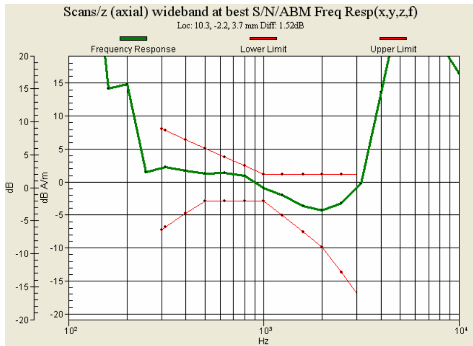
Figure 8.23: Frequency Response of WCDMA Band II for Ch9400
