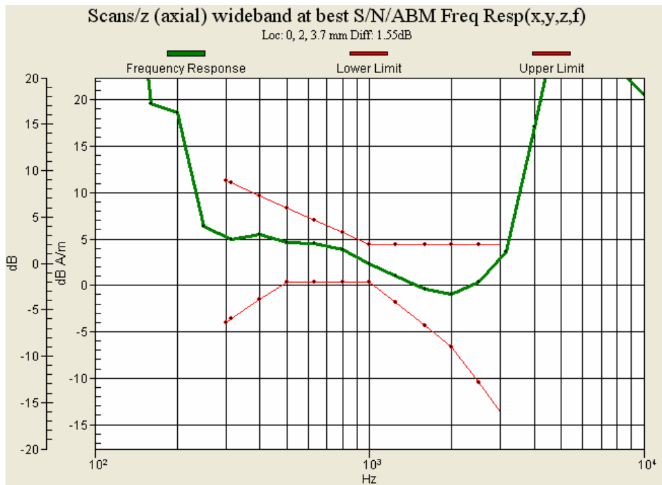
Figure 8.21: Frequency Response of WCDMA Band V for Ch4233
