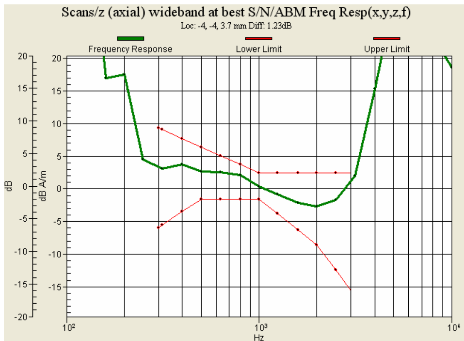
Figure 8.20: Frequency Response of WCDMA Band V for Ch4182
