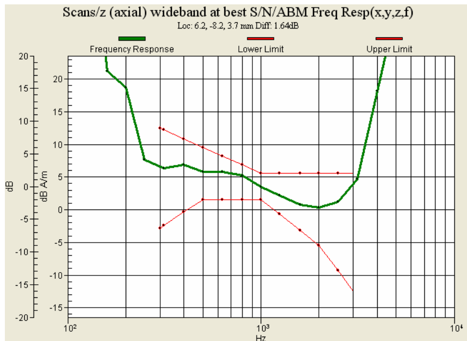
Figure 8.24: Frequency Response of WCDMA Band II for Ch9538
