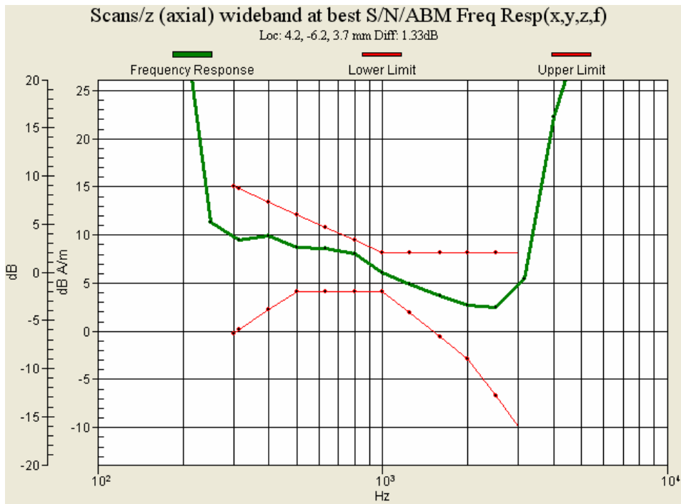
Figure 8.2: Frequency Response of GSM850 for Ch189
