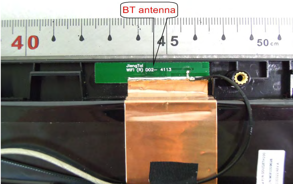
BT Antenna
