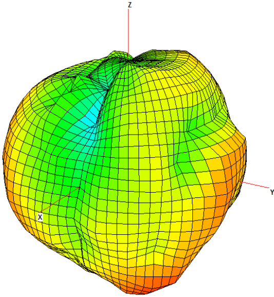
Radiation Pattern 2450 MHz BT
