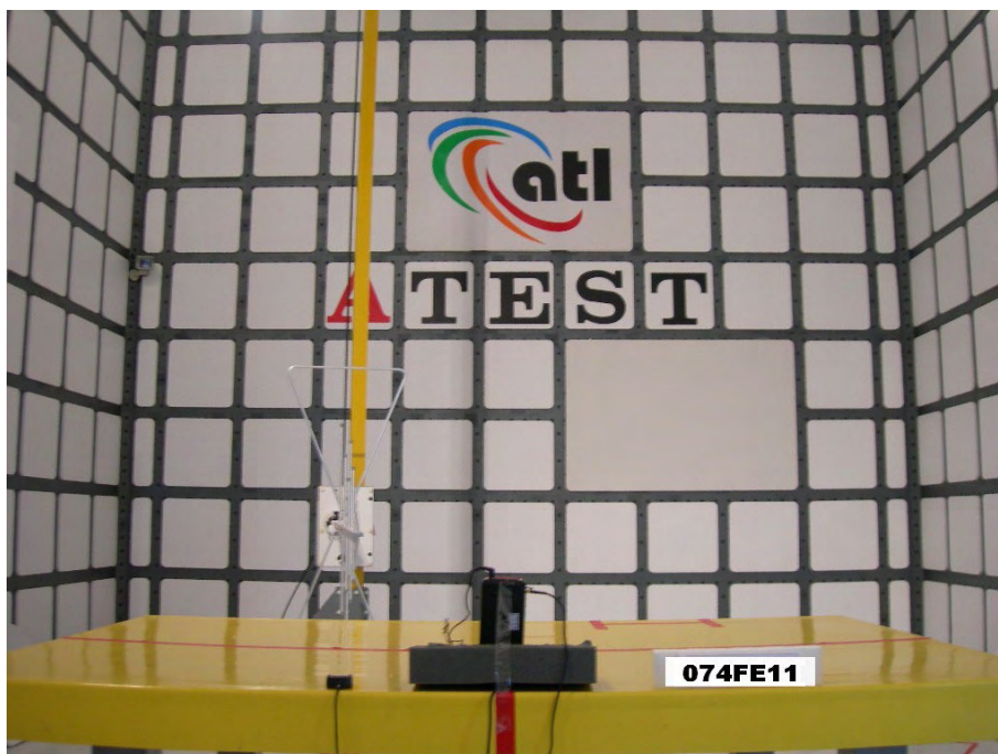
Figure 6. Rear View of the Test Configuration (AC Adapter)
