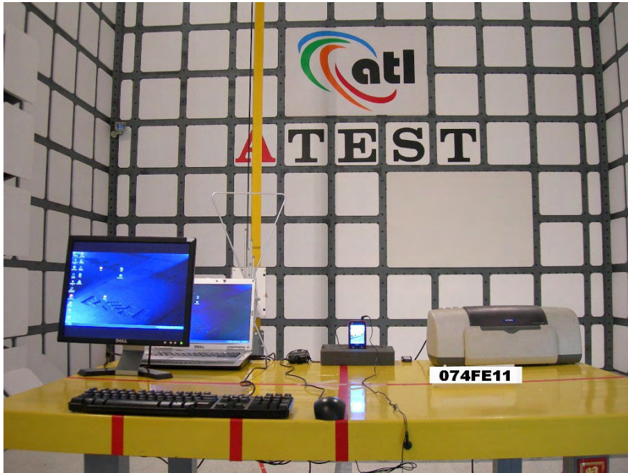
Figure 7. Front View of the Test Configuration (PC USB LINK)
