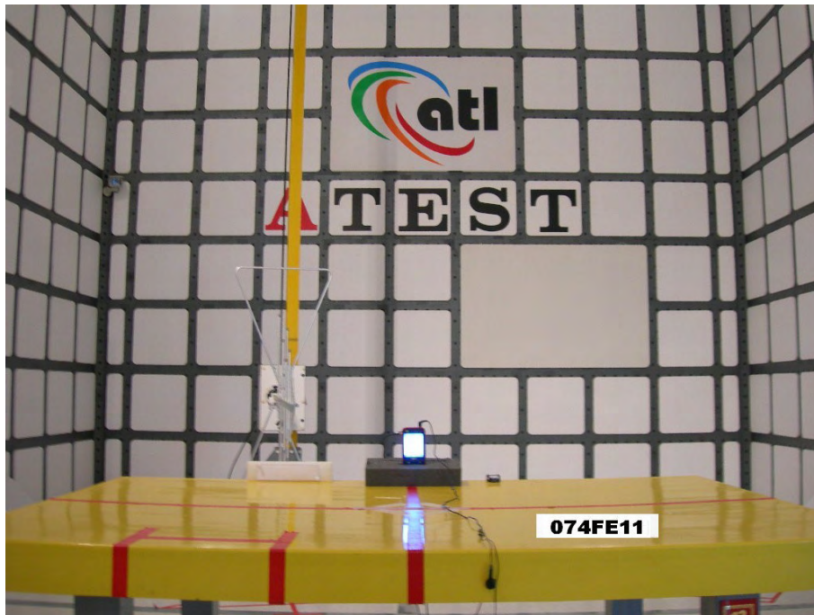
Figure 5. Front View of the Test Configuration (AC Adapter)
