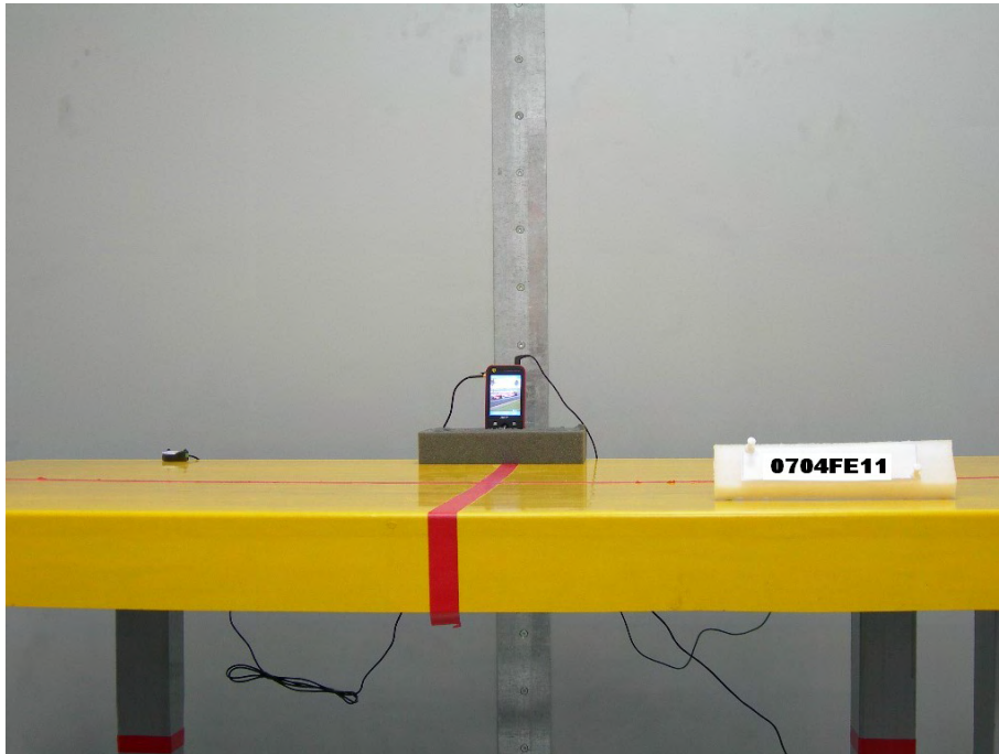
Figure 1. Front View of the Test Configuration (AC Adapter)
