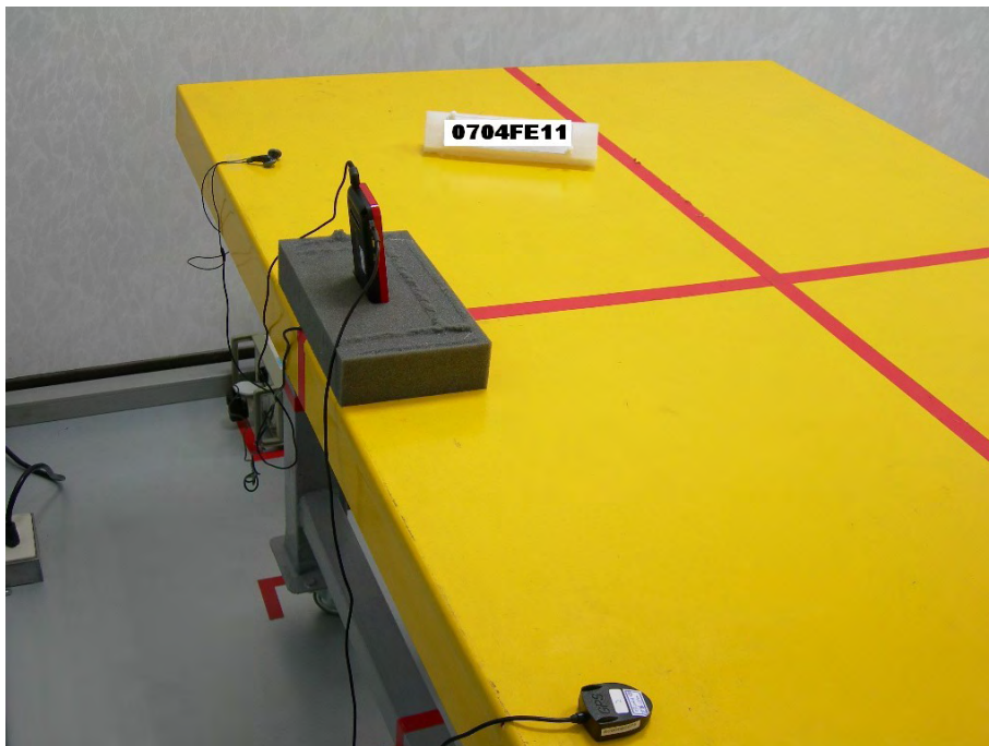
Figure 2. Rear View of the Test Configuration (AC Adapter)
