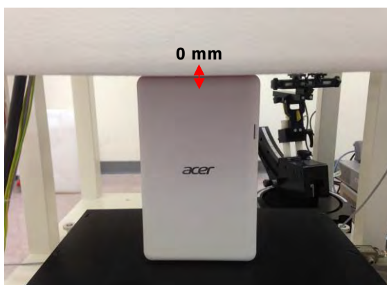
Fig.5 EUT Edge 1(Top) to flat phantom
