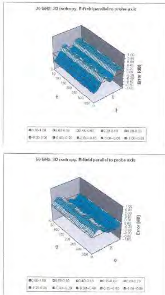
Probe isotropy for E_{loc} : probe rotated \varphi = 0^\circ to 360^\circ , tilted from field propagation direction \bar{k} Parallel to the field propagation ( \varphi = 0^\circ - 90^\circ ) at 30 GHz: deviation within \pm 0.40 dB Parallel to the field propagation ( \varphi = 0^\circ - 90^\circ ) at 60 GHz: deviation within \pm 0.38 dB
