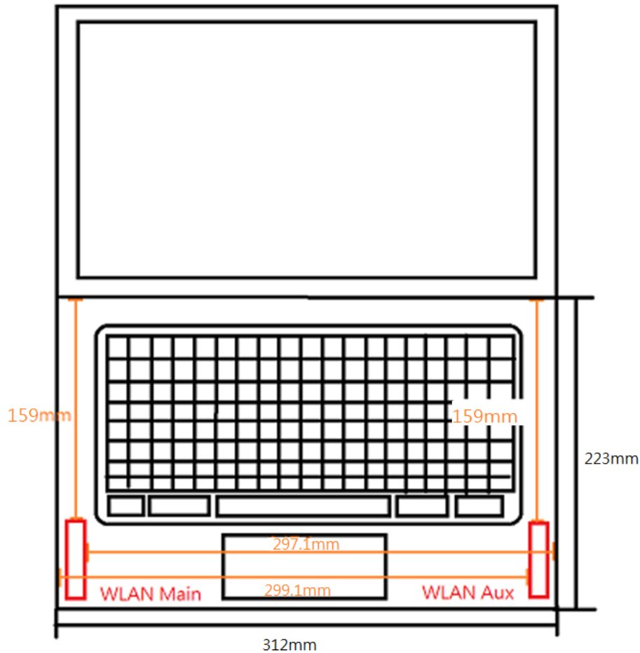
Photograph 17. Antenna position of EUT
