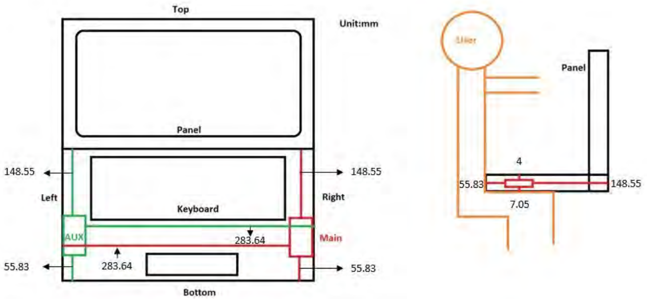
Fig.11 Antenna position of EUT
