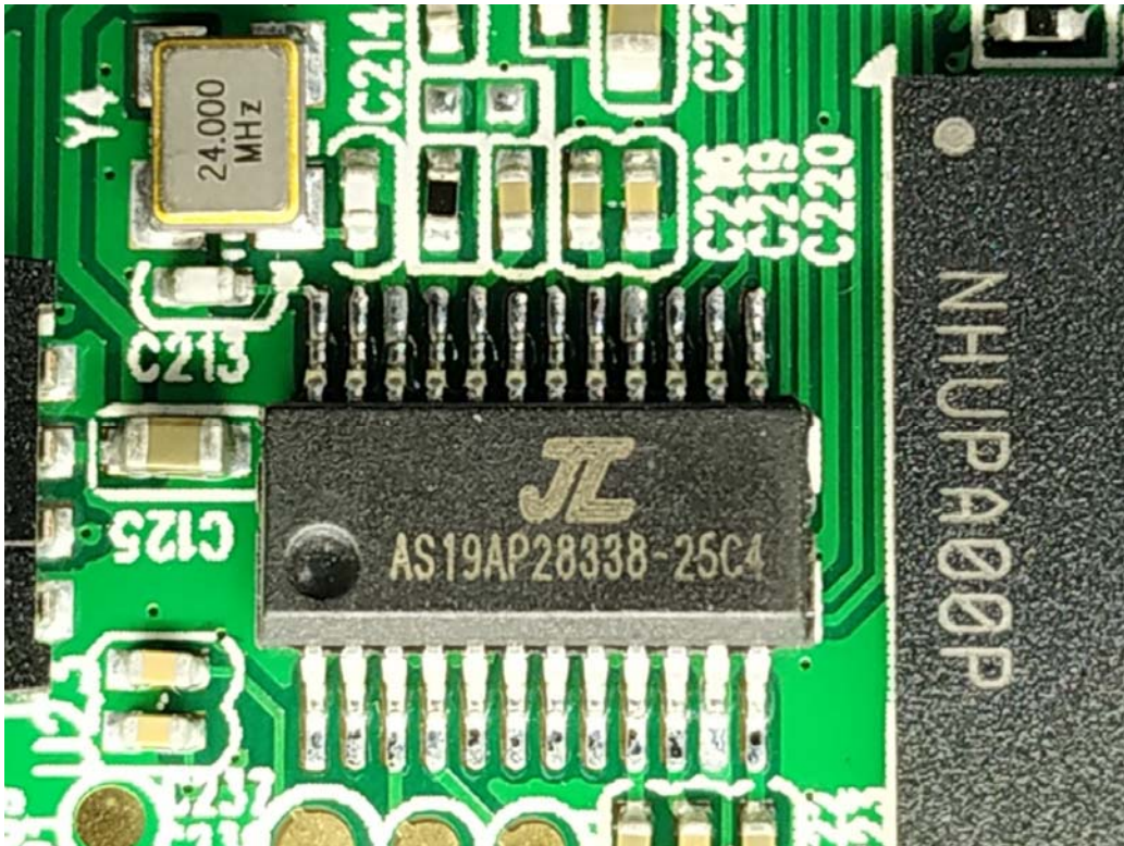
Radio 1 Chip
