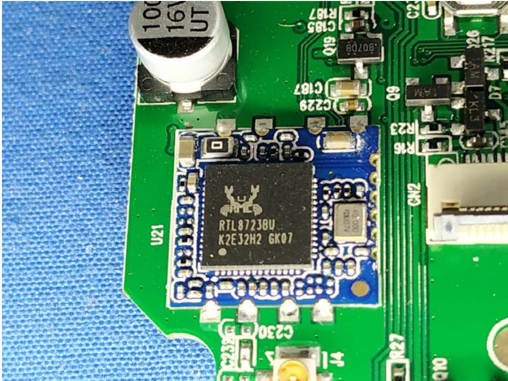
WIFI/BT module(Radio 2)
